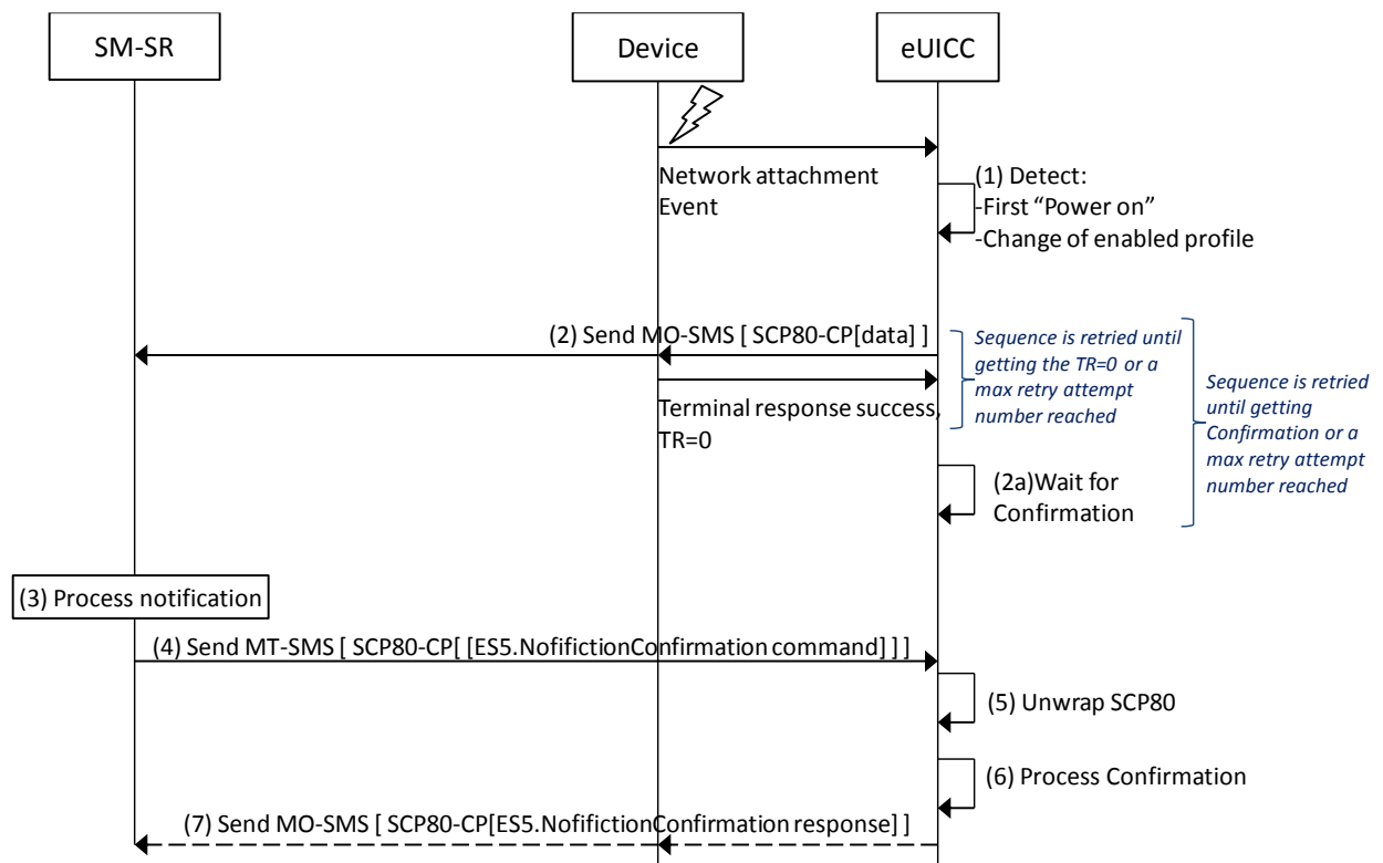
Figure 29: Sequence Flow of Notification Over SMS
