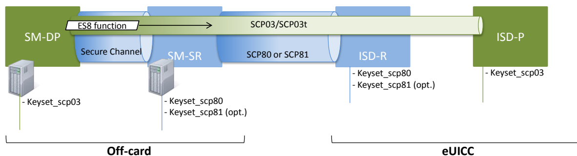
Figure 6: Secure Channel Between SM-DP and ISD-P
