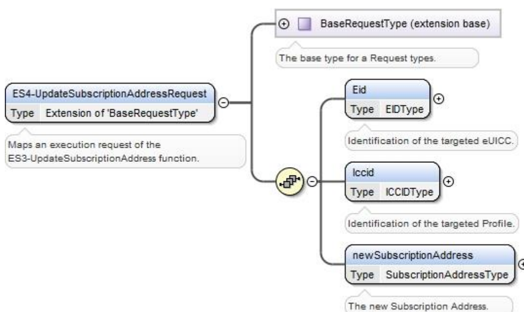
Figure 115: <rps:ES4-UpdateSubscriptionAddressRequest>
