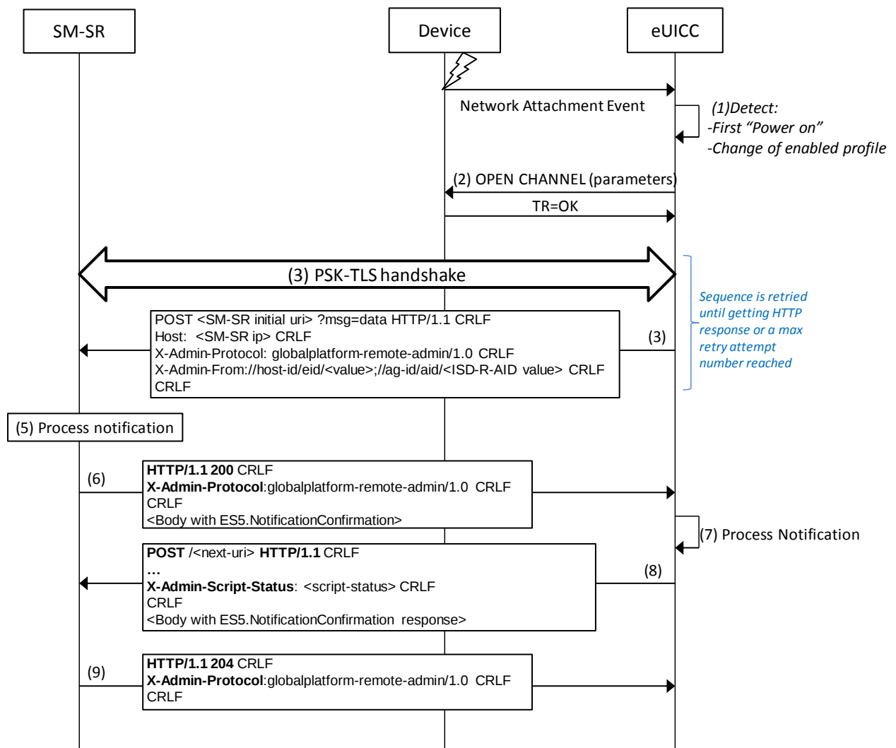
Figure 30: Sequence Flow of Notification Over HTTPS
