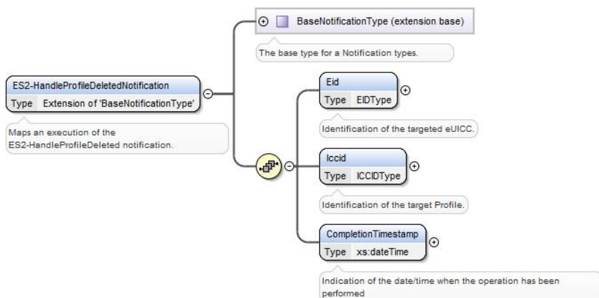
Figure 84: <rps:ES2-HandleProfileDeletedNotification >
