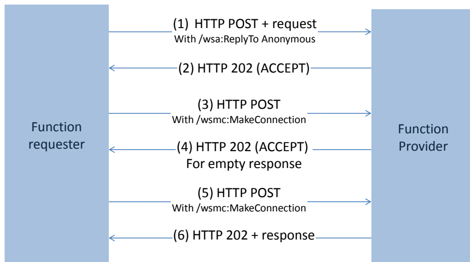
Figure 142: MEP: Asynchronous With Polling
