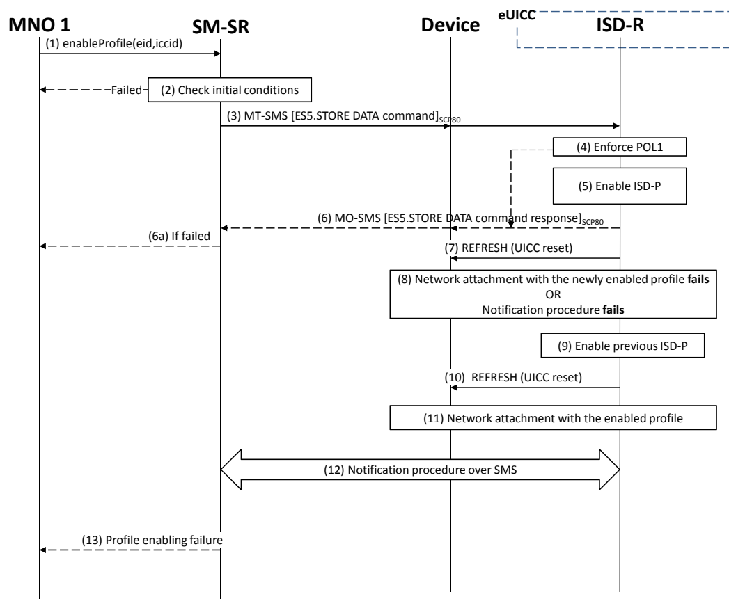
Figure 15: Profile Enabling, with fall-back
