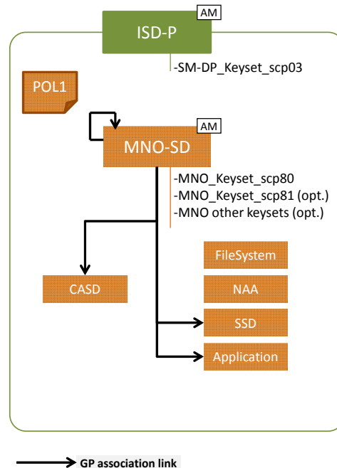
Figure 4: Profile Structure overview
