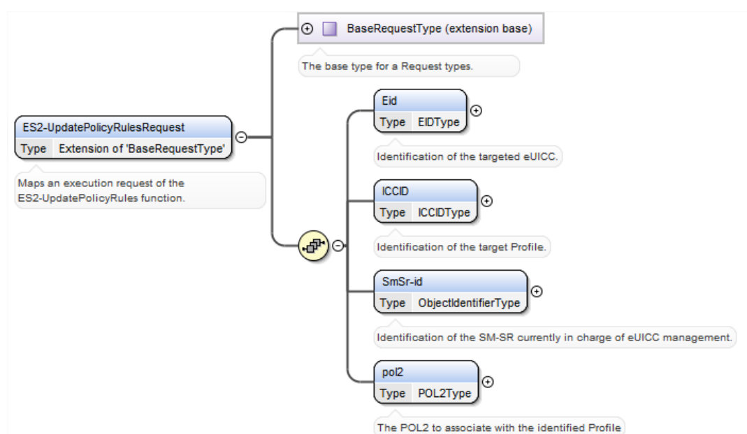
Figure 70 <rps:ES2-UpdatePolicyRulesRequest >
