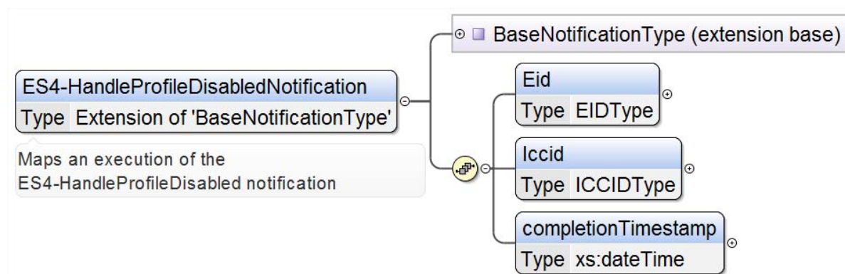
Figure 128 <rps:ES4-HandleProfileDisabledNotification>
