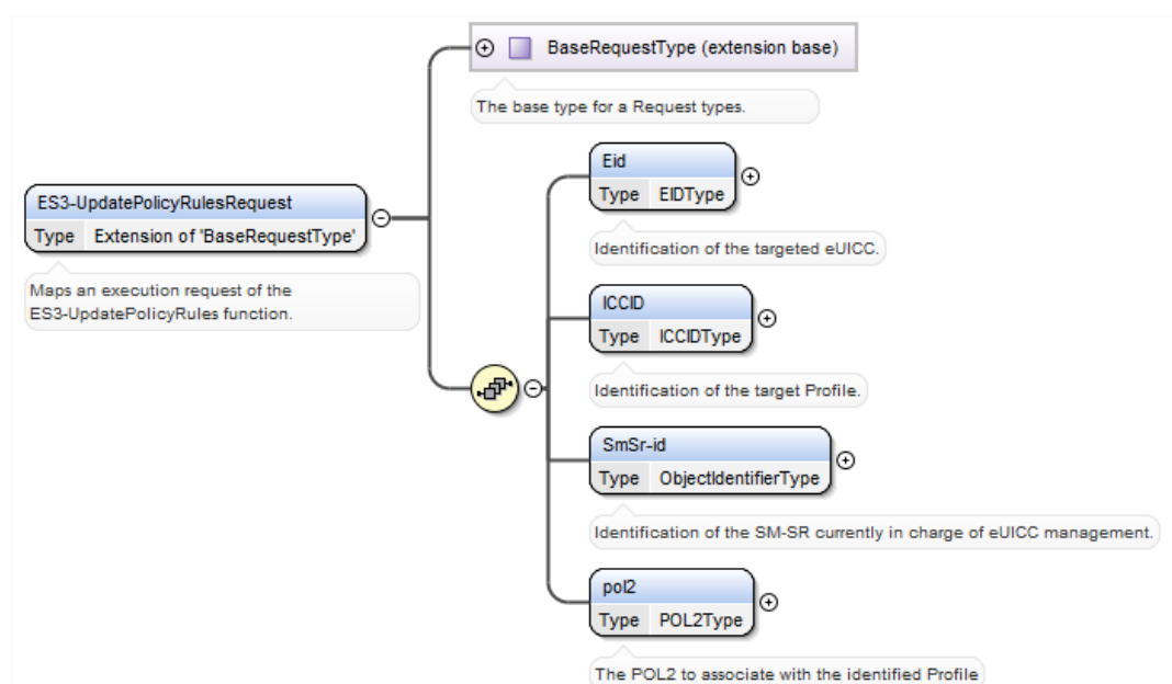
Figure 94 <rps:ES3-UpdatePolicyRulesRequest>
