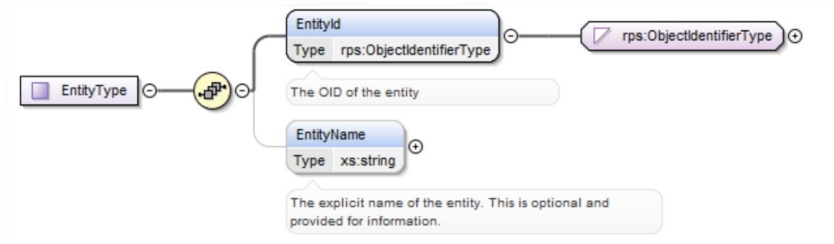
Figure 36 &lt;rps:Entity&gt;
