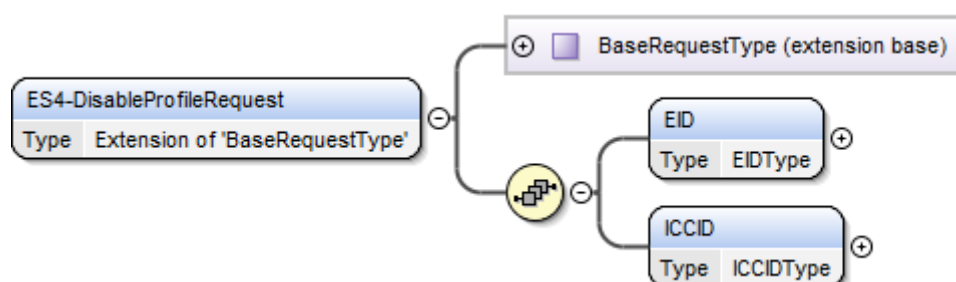
Figure 120 <rps:ES4-DisableProfile Request>
