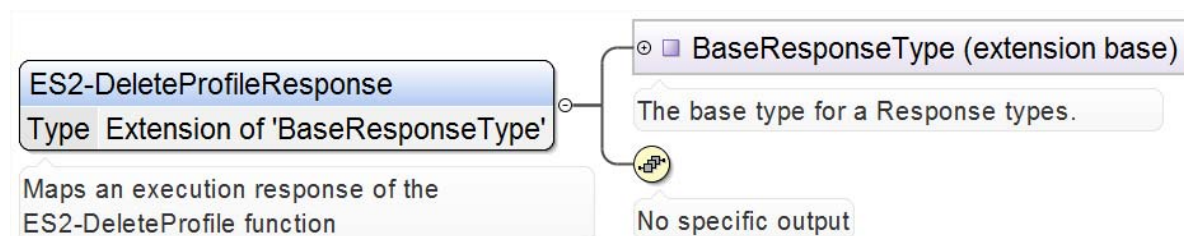
Figure 79 <rps:ES2-DeleteProfile Response>
