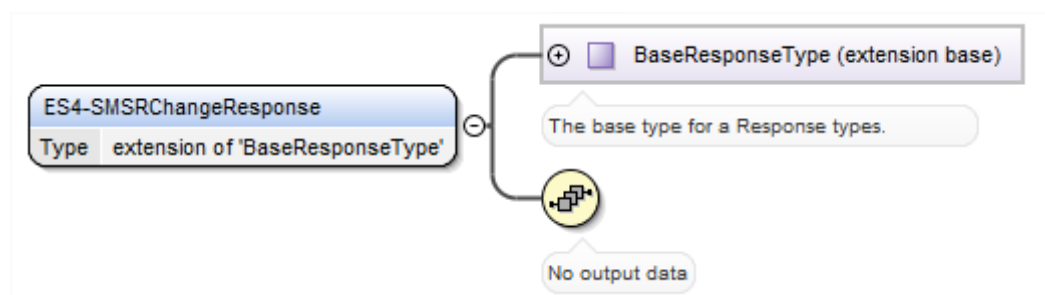
Figure 127 <rps:ES4-SMSRChangeResponse>
