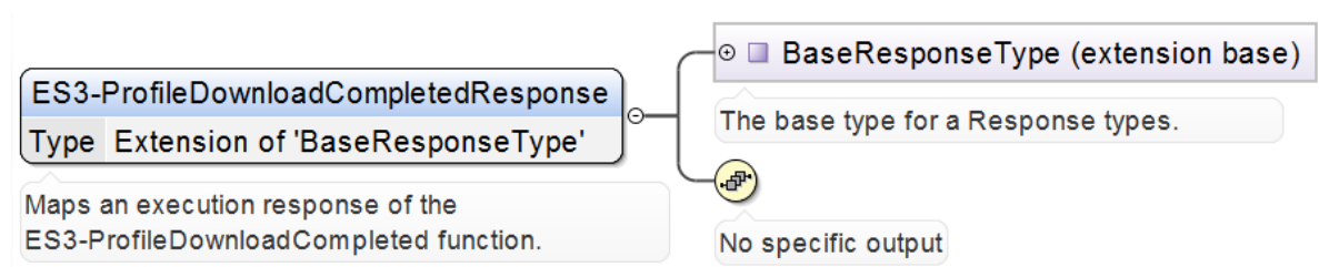
Figure 93 &lt;rps:ES3-ProfileDownloadCompleted Response&gt;
