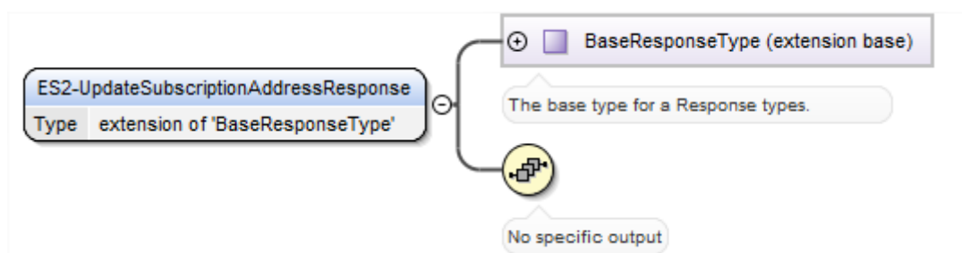
Figure 73 <rps:ES2-UpdateSubscriptionAddressResponse>
