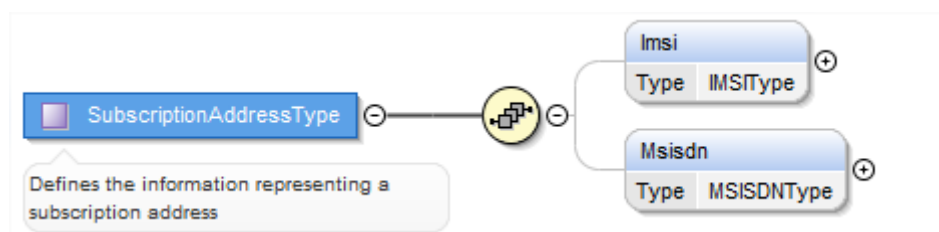
Figure 63 &lt;rps:SubscriptionAddressType&gt;
