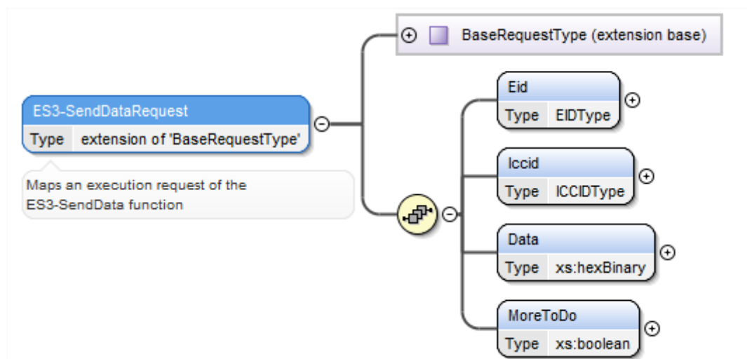
Figure 90 &lt;rps:ES3-SendDataRequest&gt;
