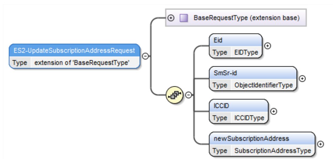
Figure 72 <rps:ES2-UpdateSubscriptionAddressRequest>
