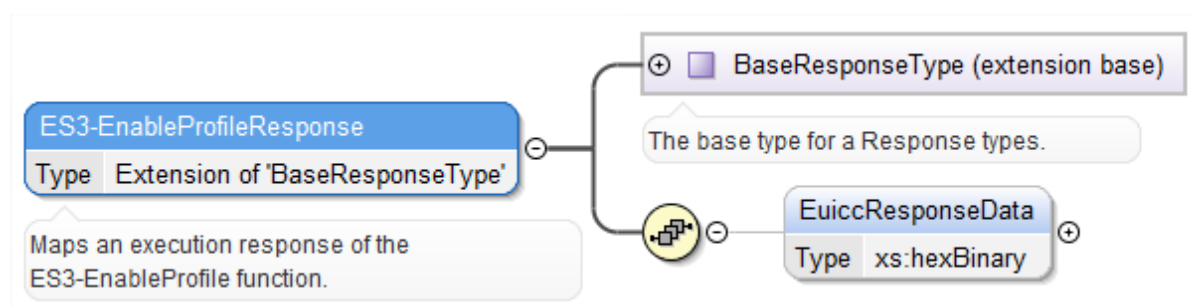
Figure 99 <rps:ES3-EnableProfileResponse>
