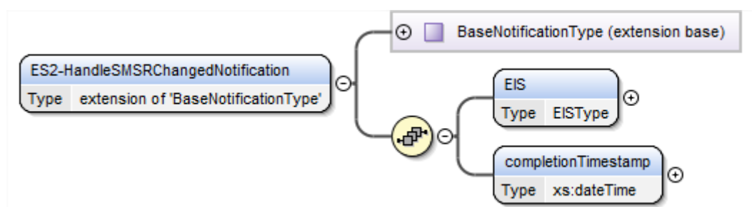
Figure 82 <rps:ES2-HandleSMSRChangeNotification>
