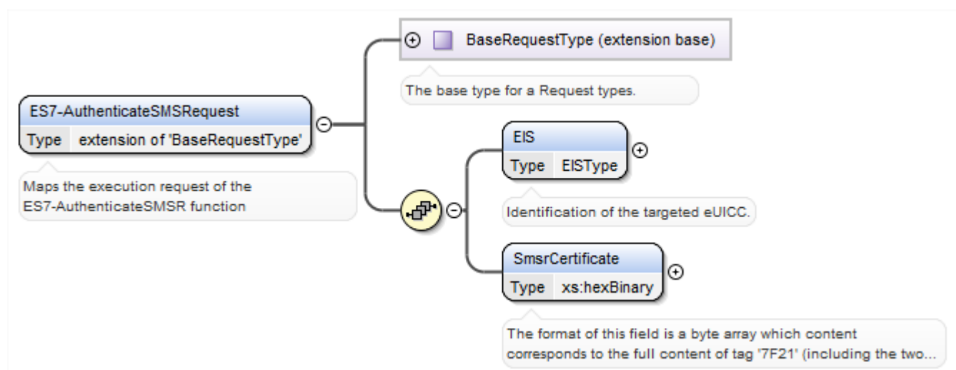
Figure 136 <rps:ES7-AuthenticateSMSRRequest>
