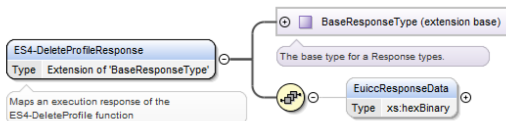
Figure 123 &lt;rps:ES4-DeleteProfile Response&gt;
