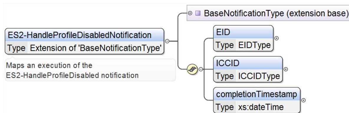
Figure 80 <rps:ES2- HandleProfileDisabledNotification >
