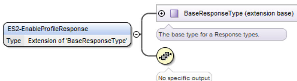
Figure 75 <rps:ES2-EnableProfileResponse>
