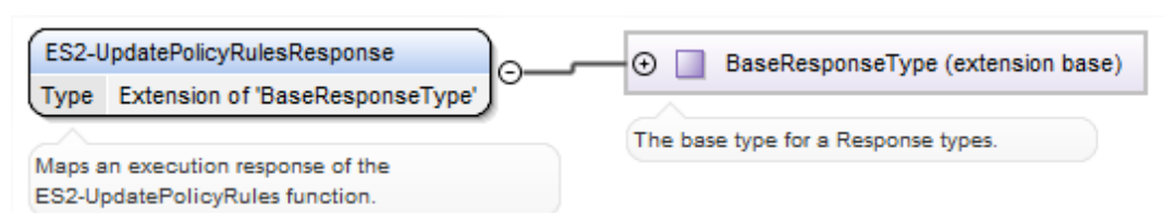
Figure 71 <rps:ES2-UpdatePolicyRulesResponse >
