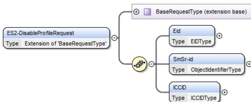
Figure 76 <rps:ES2-DisableProfile Request>
