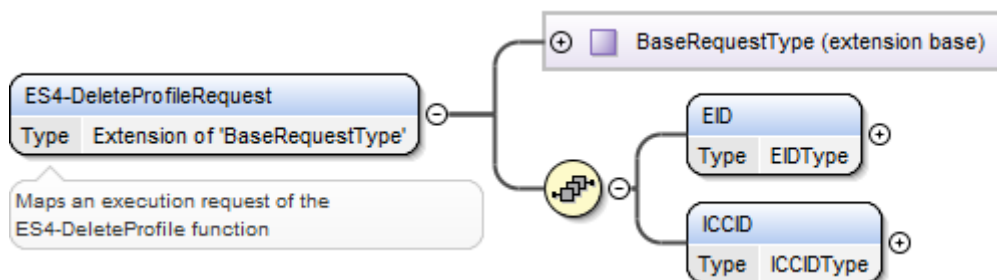
Figure 122 <rps:ES4-DeleteProfile Request>
