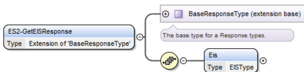
Figure 67 <rps:ES2-GetEISResponse>
