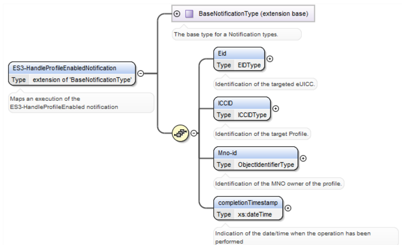
Figure 107 &lt;rps:ES3-HandleProfileEnabledNotification&gt;
