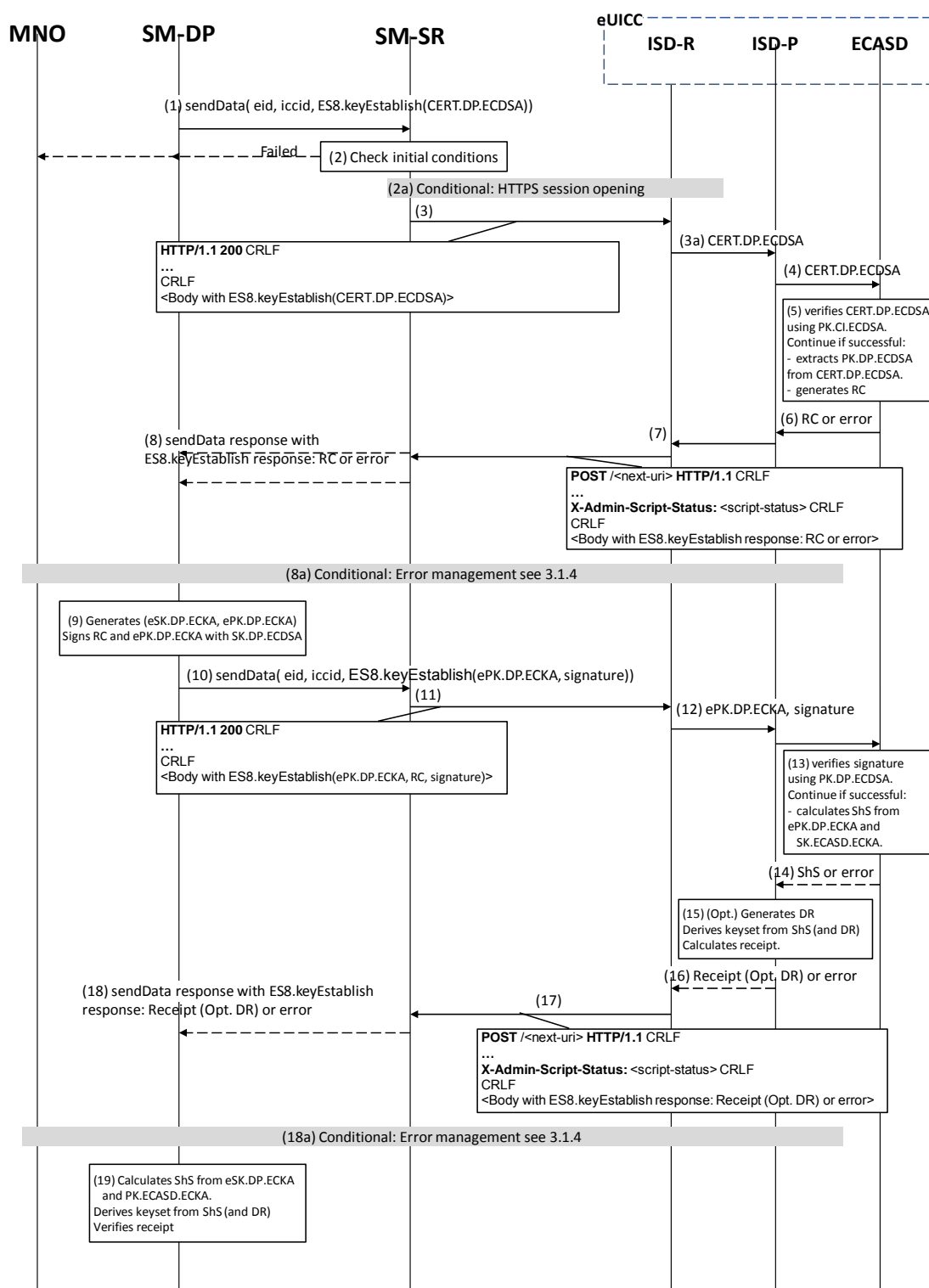
Figure 11: Key Establishment, Scenario #3
