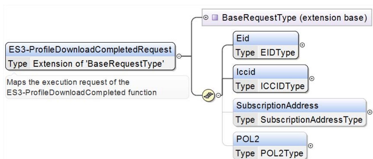
Figure 92 &lt;rps:ES3-ProfileDownloadCompleted Request&gt;
