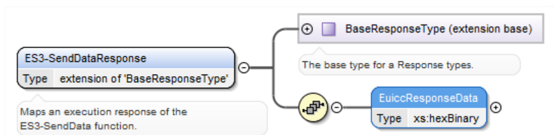
Figure 91 &lt;rps:SendDataResponse&gt;
