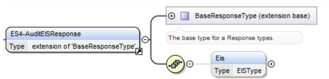
Figure 117 <rps:ES4-AuditEISResponse>
