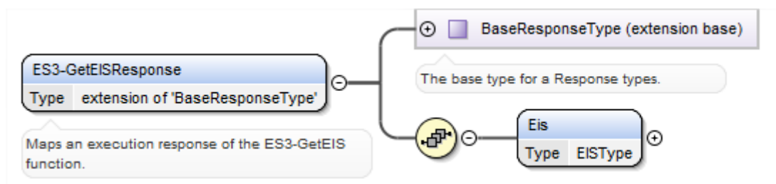
Figure 85 &lt;rps:GetEISResponse&gt;
