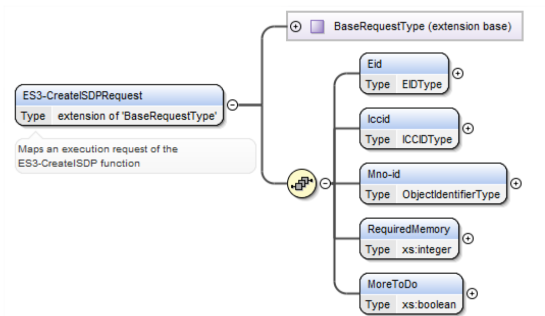
Figure 88 <rps:ES3-CreateISDPRequest>
