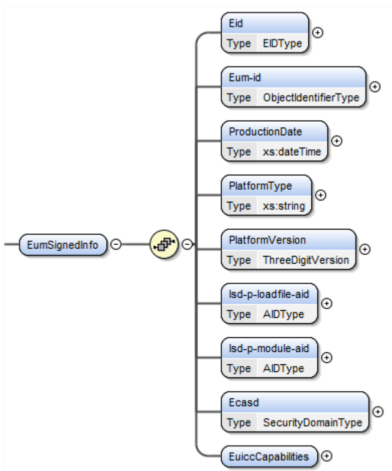
Figure 53 <rps:EumSignedInfo>
