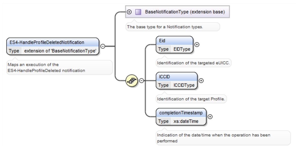
Figure 131 <rps:ES4-HandleProfileDeletedNotification>
