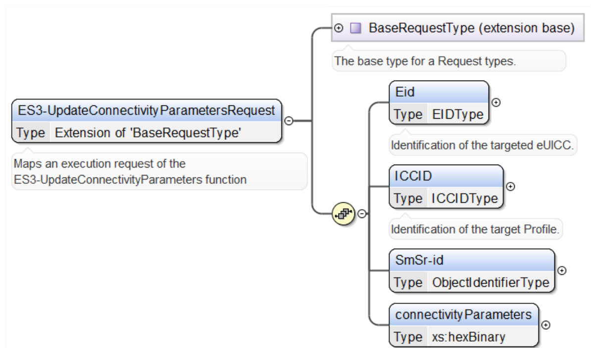
Figure 104 <rps:ES3- UpdateConnectivityParametersRequest>
