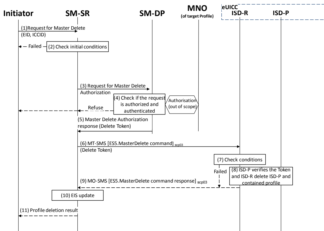
Figure 24: Master Delete
