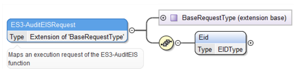
Figure 86 &lt;rps:ES3-AuditEIS Request&gt;
