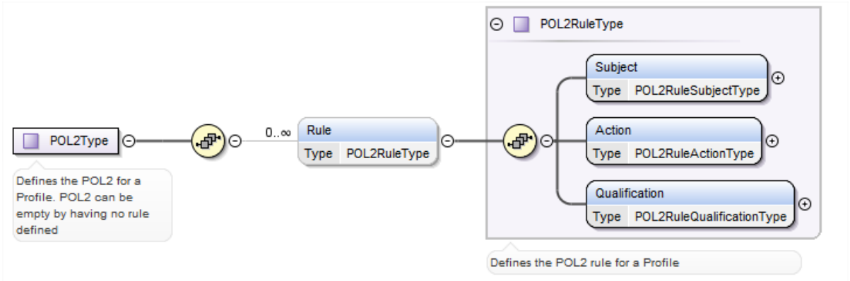
Figure 62 <rps:POL2Type>
