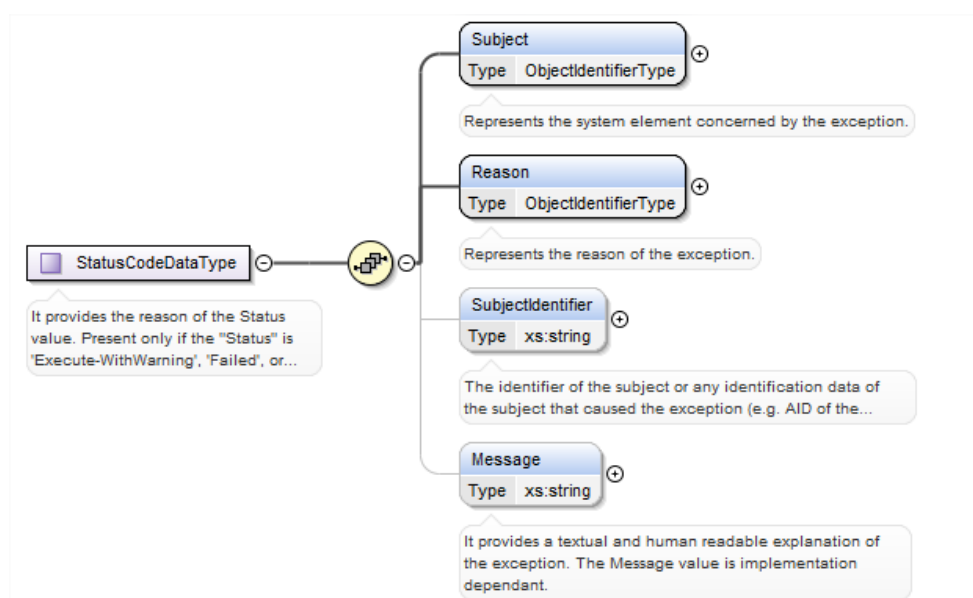
Figure 42 &lt;rs:StatusCodeDataType&gt;
