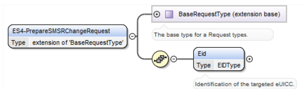
Figure 124 &lt;rps:ES4-PrepareSMSRChangeRequest&gt;
