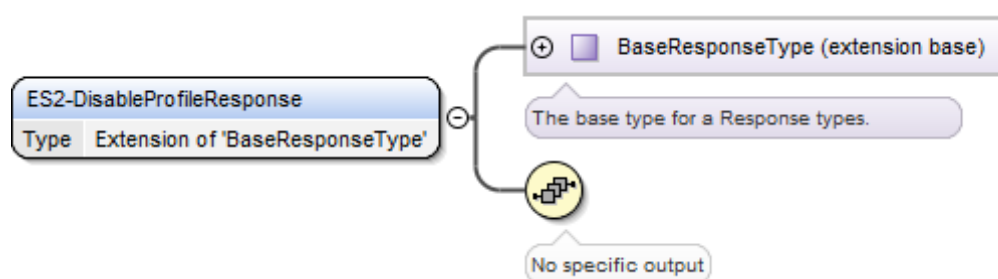
Figure 77 <rps:ES2-DisableProfileResponse>
