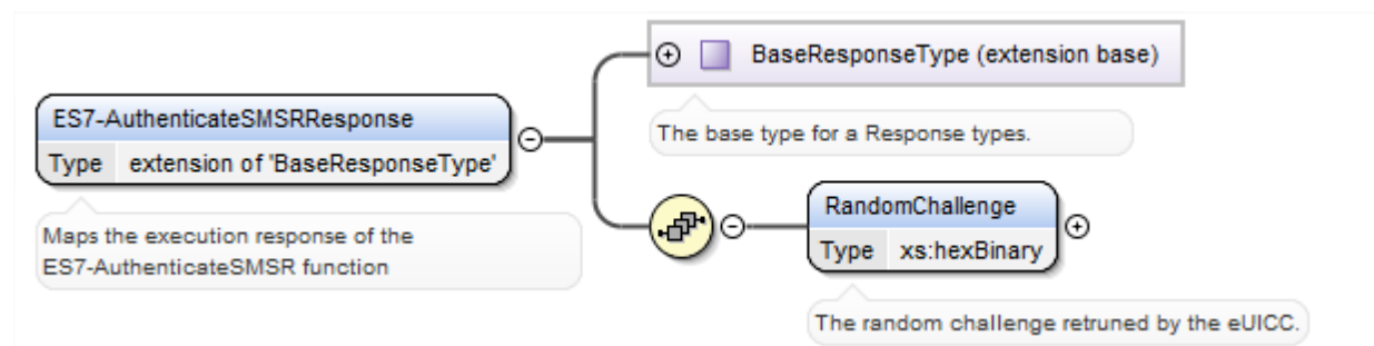
Figure 137 <rps:ES7-AuthenticateSMSRResponse>
