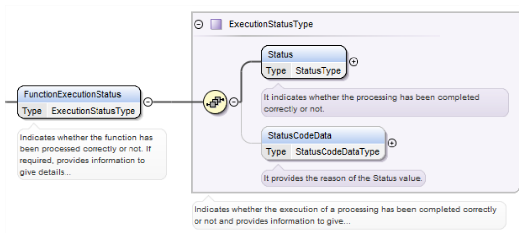
Figure 41 &lt;rs:FunctionExecutionStatusType&gt;
