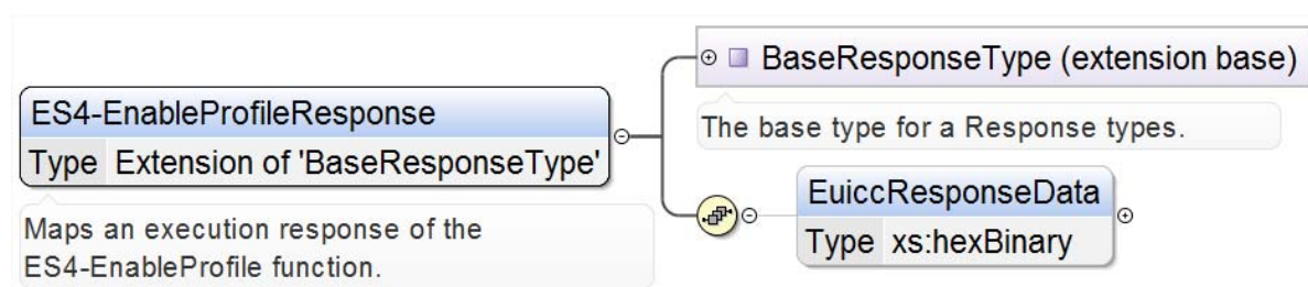
Figure 119 <rps:ES4-EnableProfileResponse>
