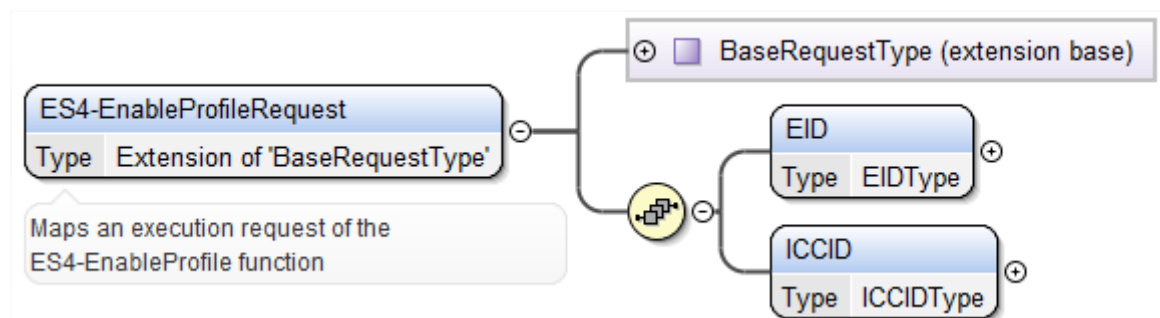
Figure 118 <rps:ES4-EnableProfile Request>
