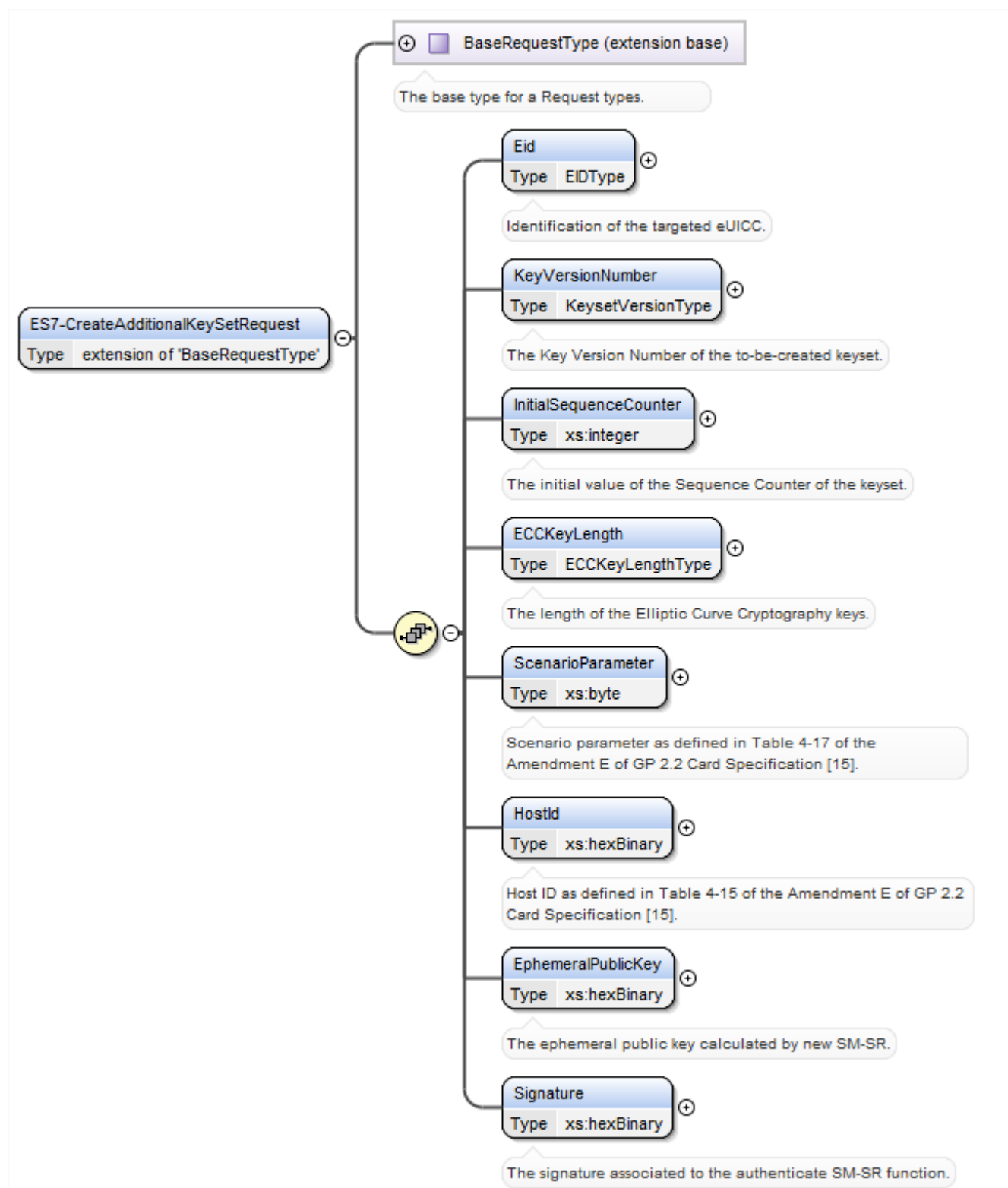
Figure 132 <rps:ES7-CreateAdditionalKeySetRequest>
