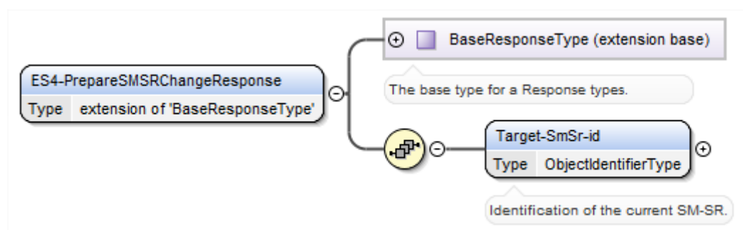
Figure 125 &lt;rps:ES4-PrepareSMSRChangeResponse&gt;
