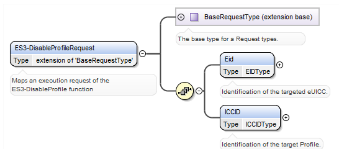
Figure 100 <rps:ES3-DisableProfile Request>
