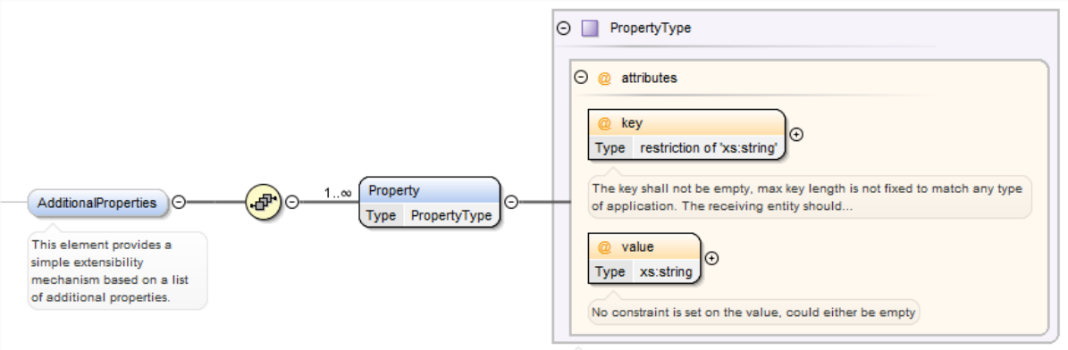
Figure 52 <rps: EISType >
