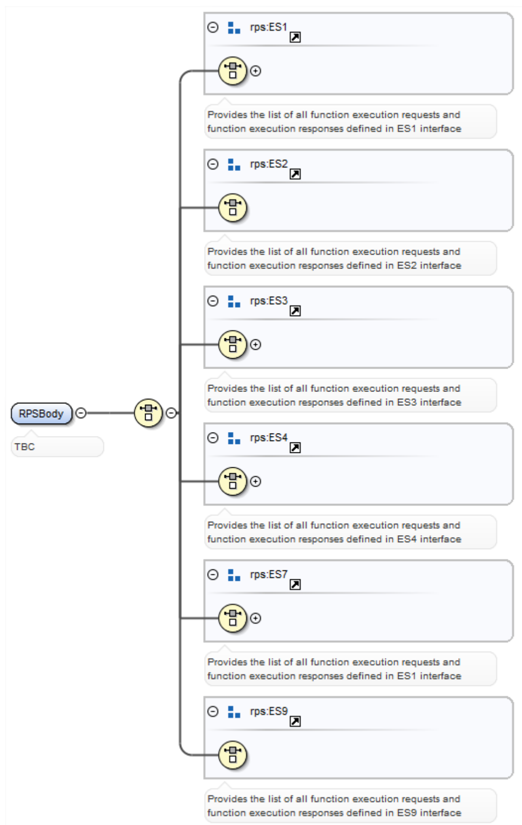
Figure 37 <rps:RPSBody>
