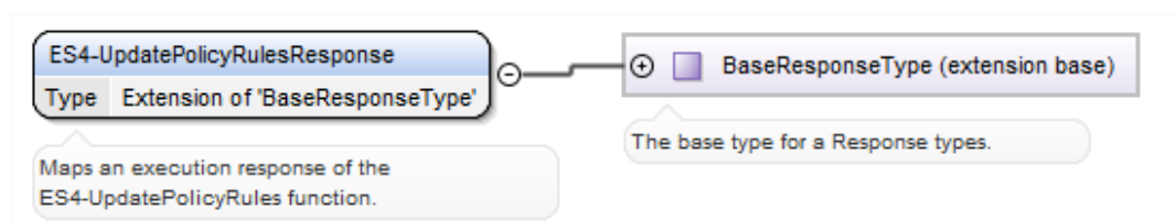
Figure 113 <rps:ES4.UpdatePolicyRulesResponse>
