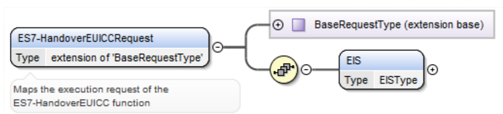
Figure 134 <rps:ES7-HandoverEUICCRequest>
