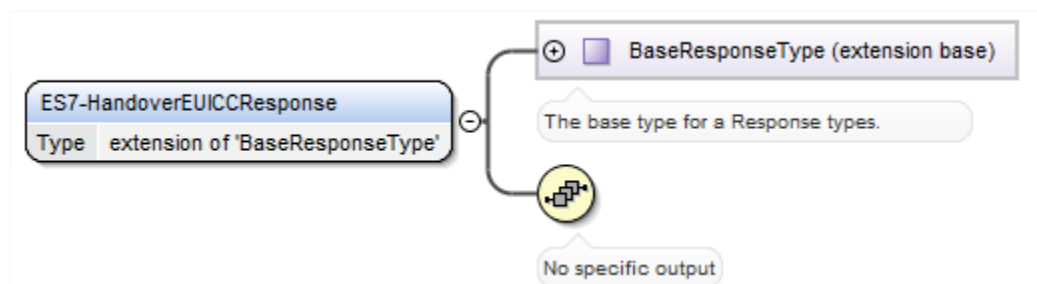
Figure 135 <rps:ES7-HandoverEUICCResponse>
