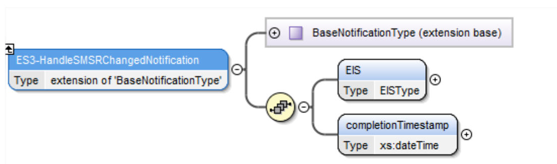
Figure 108 &lt;rps:ES3-HandleSMSRChangeNotification&gt;
