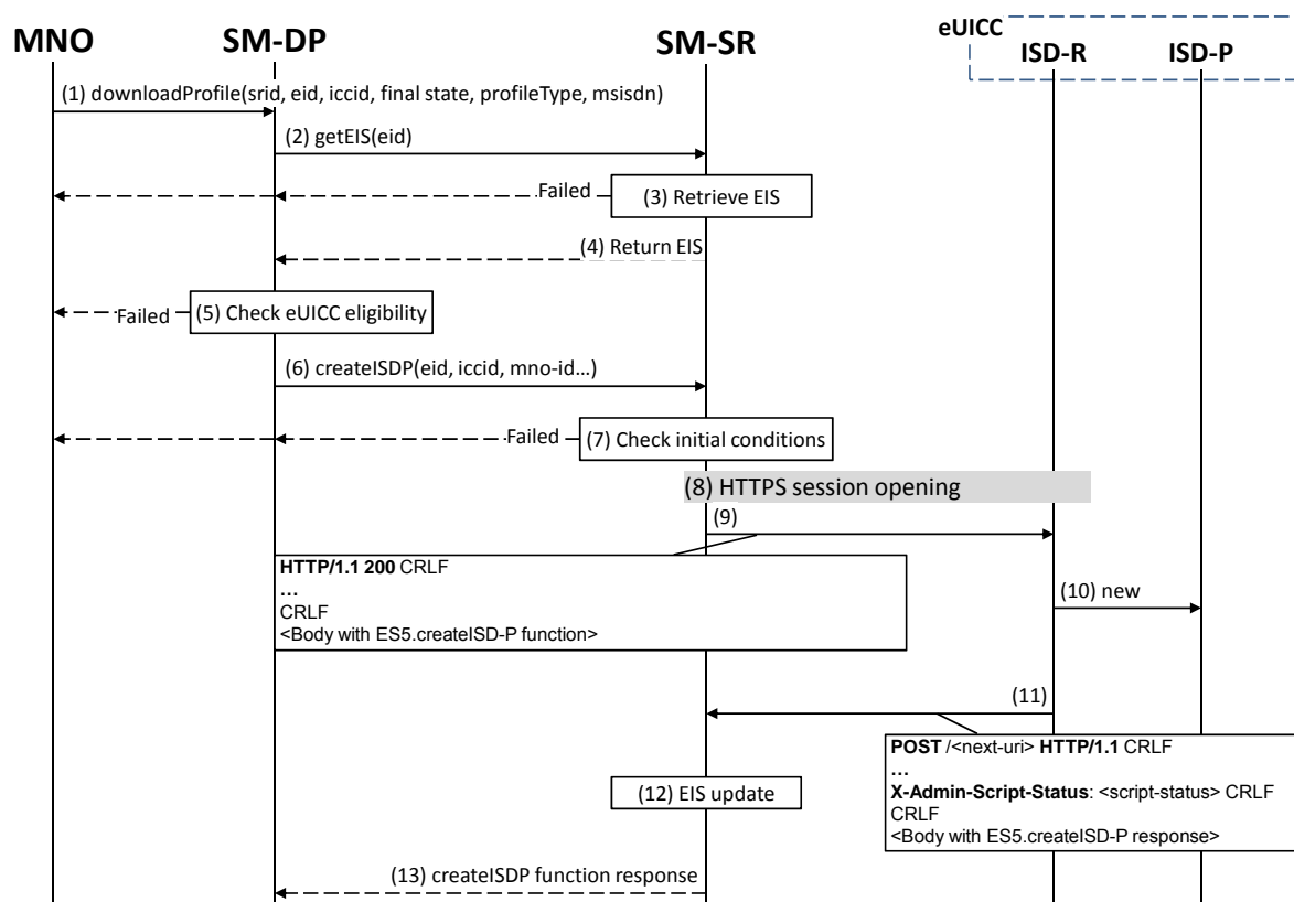
Figure 10: ISD-P creation
