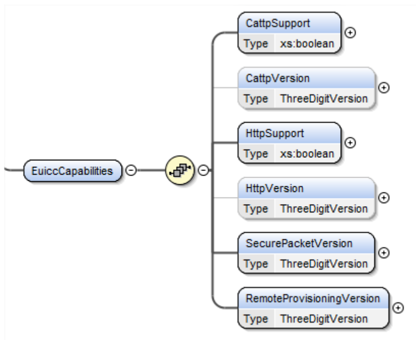
Figure 61 <rps:EuiccCapabilities>
