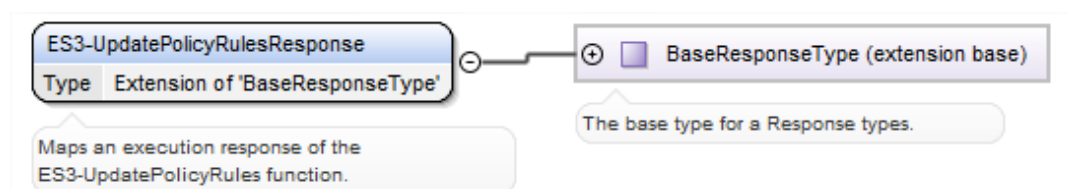
Figure 95 <rps:ES3-UpdatePolicyRulesResponse >
