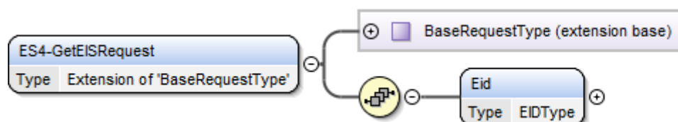
Figure 110 <rps:ES4-GetEISRequest>
