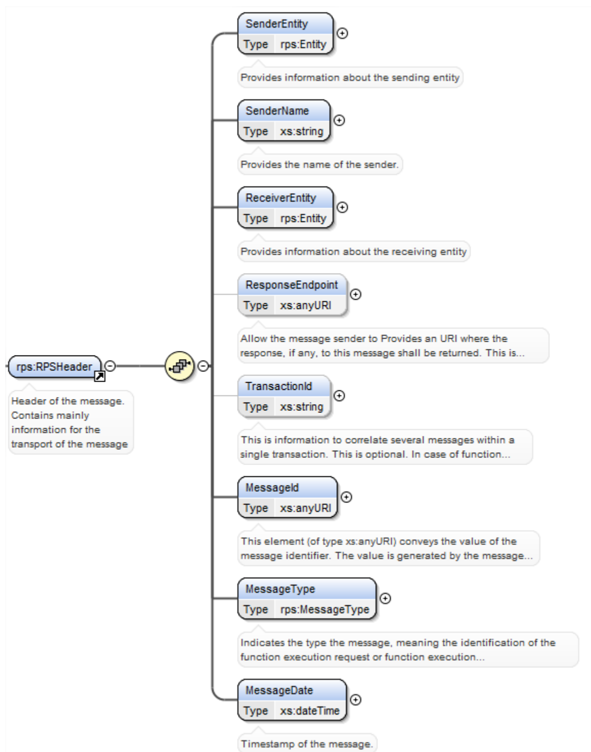
Figure 35: <rps:RPSHeader>
