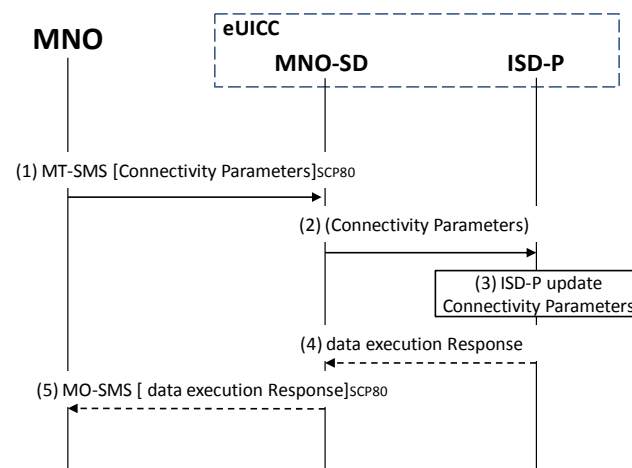
Figure 27: Connectivity Parameters Update by MNO
