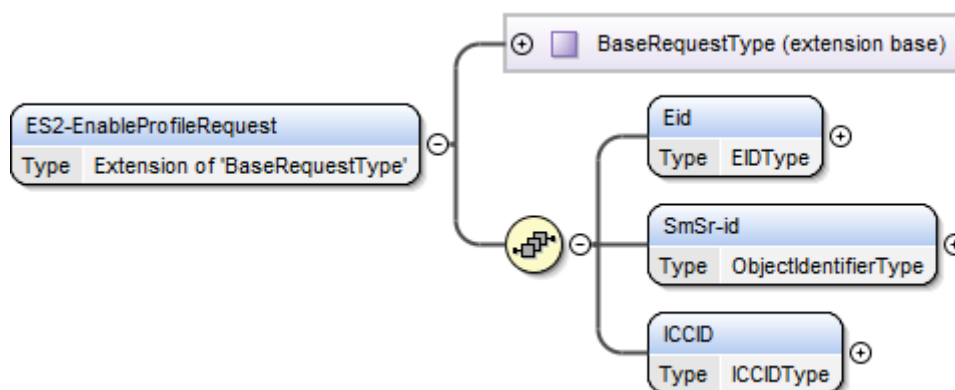
Figure 74 <rps:ES2-EnableProfile Request>
