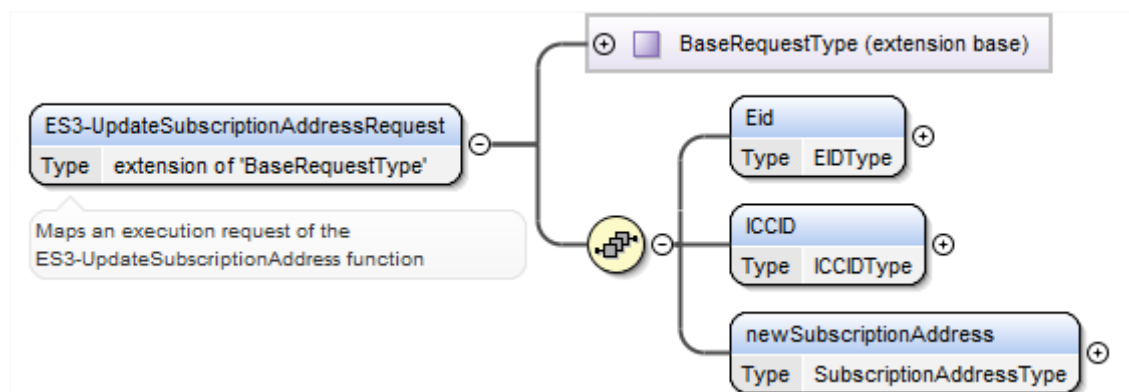
Figure 96 <rps:ES3-UpdateSubscriptionAddressRequest>
