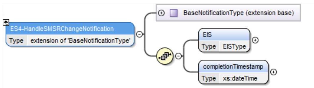
Figure 130 <rps:ES4-HandleSMSRChangeNotification>
