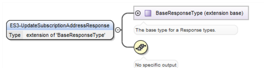
Figure 97 <rps:ES3-UpdateSubscriptionAddressResponse>
