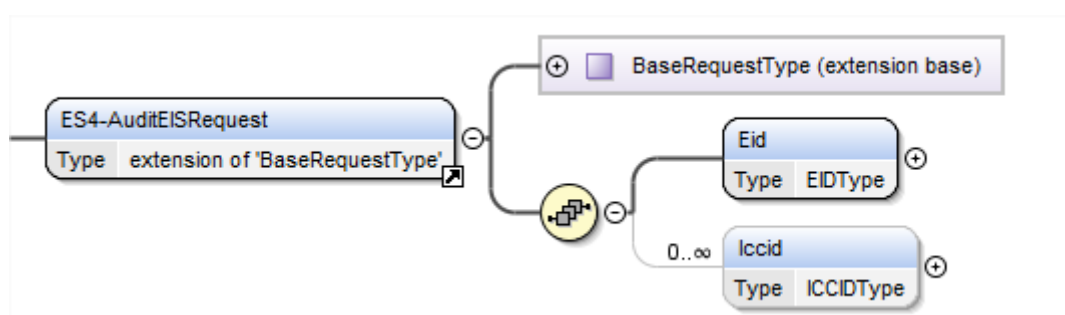
Figure 116 <rps:ES4-AuditEISRequest>
