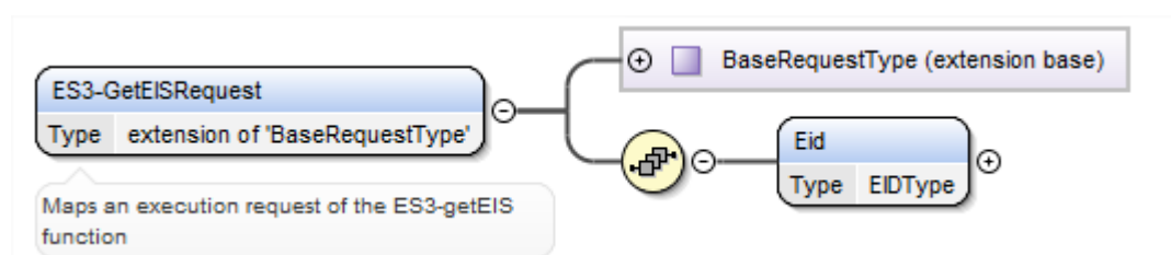
Figure 84 <rps:GetEISRequest>
