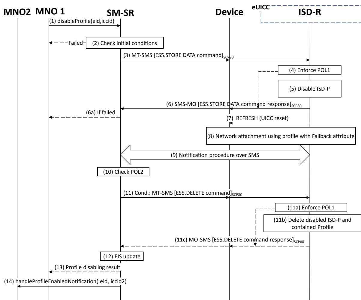
Figure 18: Profile Disabling
