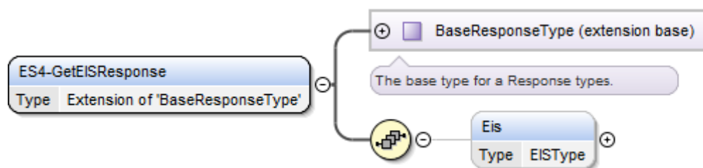
Figure 111 <rps:ES4-GetEISResponse>
