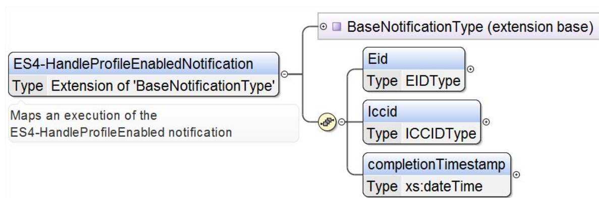
Figure 129 <rps:ES4-HandleProfileEnabledNotification>
