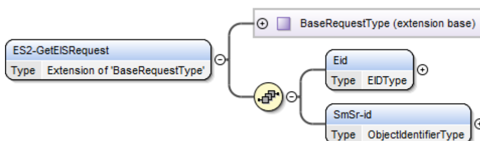
Figure 66 <rps:ES2-GetEISRequest>
