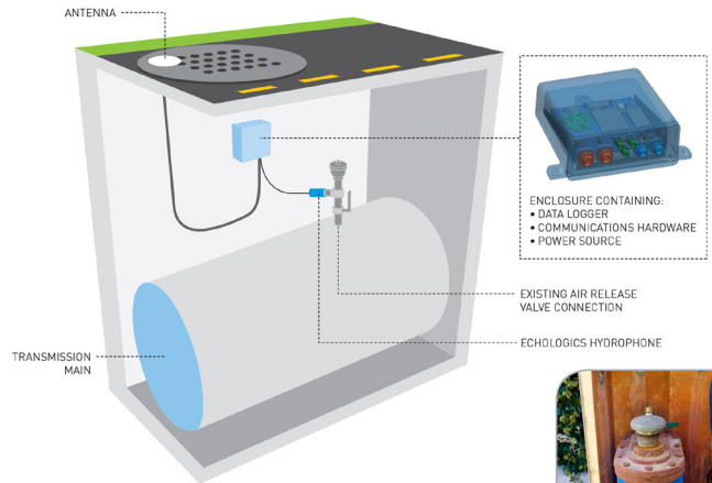
Permanent acoustic sensors installed in chambers are monitoring 4 miles of the water main pipeline installed under Las Vegas Boulevard.
