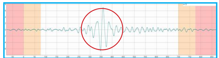
Acoustic nodes detect a leak which was simulated during commissioning of the EchoShore-TX system – leak is circled in red. The acoustic signal of the leak clearly differentiates itself from the normal acoustic noises with the water main. IBM smart water management solutions use this information to enable utilities to become proactive, predictive and prescriptive.
