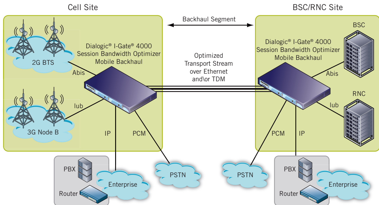
Figure 2. Dialogic® I-Gate® 4000 Session Bandwidth Optimizer Mobile Backhaul Optimizing Various Streams in the Backhaul Segment of a Mobile Network
