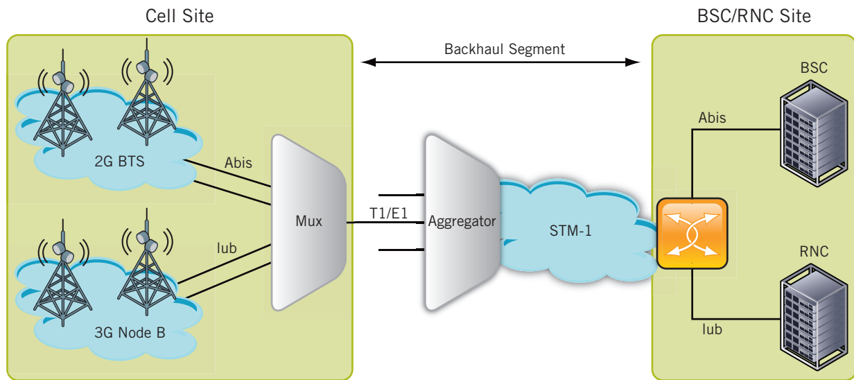
Figure 1. Backhaul in the Mobile Network
