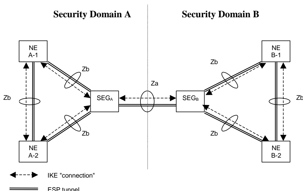
Figure D-1: NDS/IP Architecture
