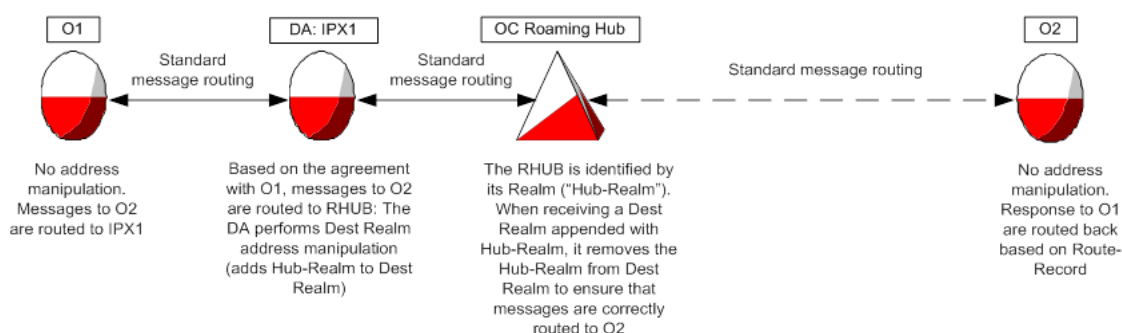
Figure 6.6.3: Destination realm modification
