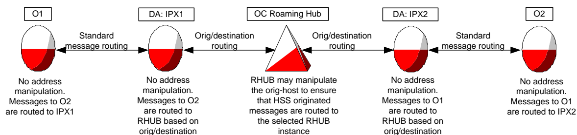
Figure 6.6.2: Origin/Destination realm based routing
