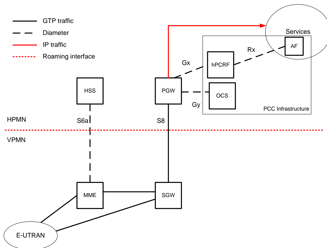
Figure 7.1-1: PCC Architecture with Home Routed architecture and S8 GTP based
