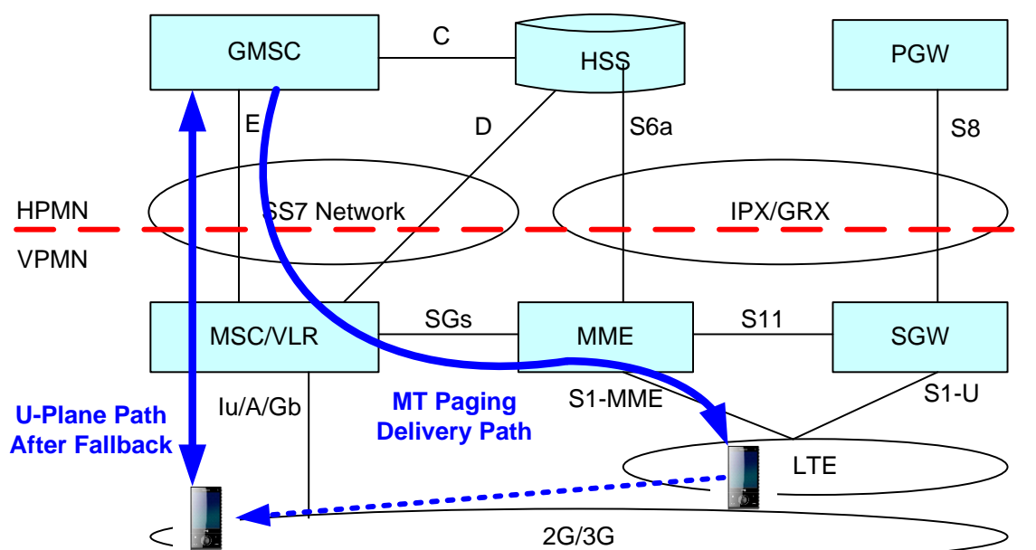
Figure 5.2.1.1-1: CSFB Roaming Architecture
