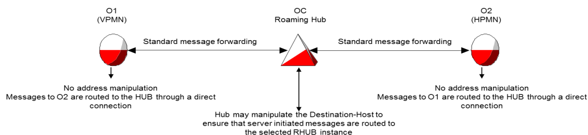
Figure 6.6.1: Direct connection
