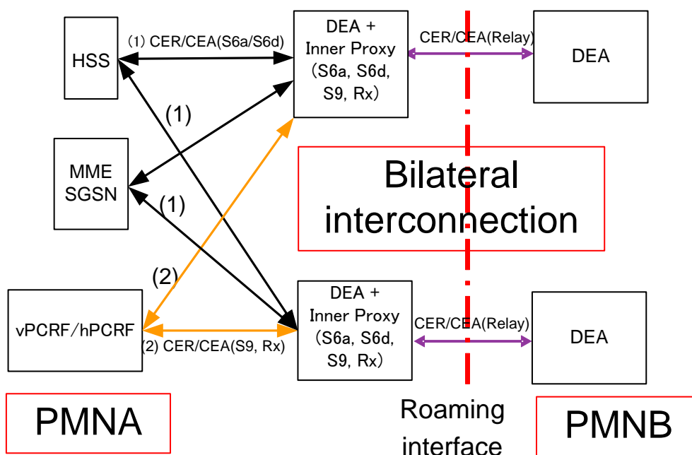
Figure 32: Diameter architecture example 2
