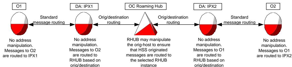
Figure 27: Origin/Destination realm based routing
