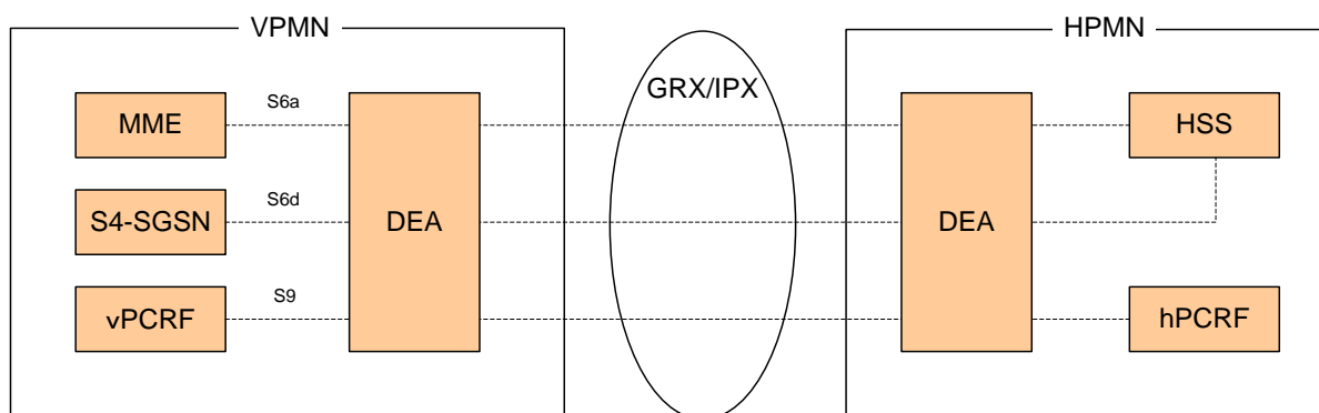
Figure 4: Diameter Roaming Implementation Architecture
