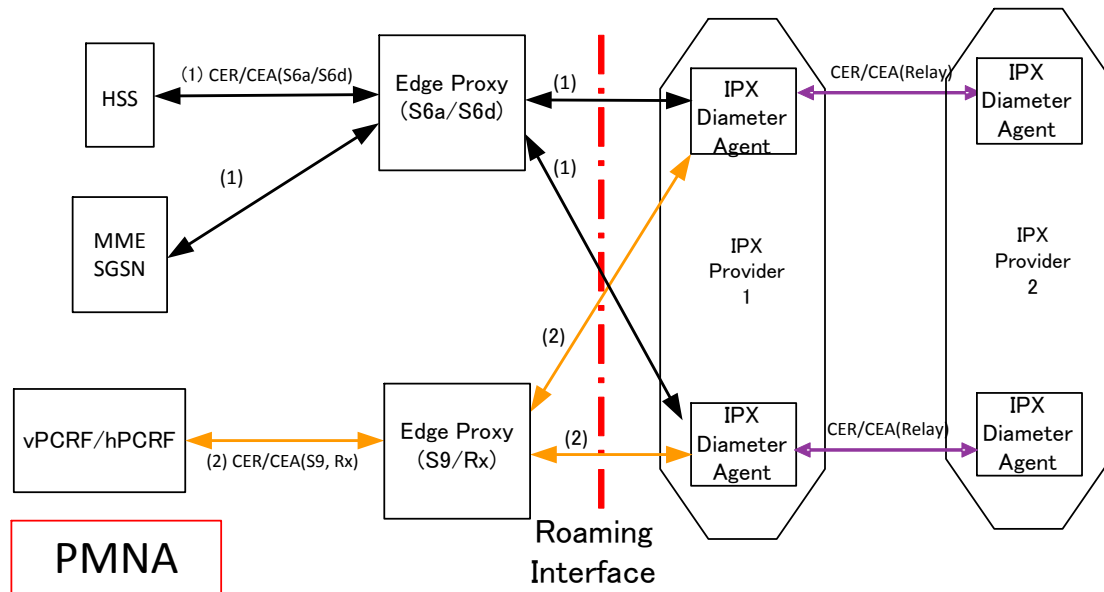
Figure 35: Diameter architecture example 5
