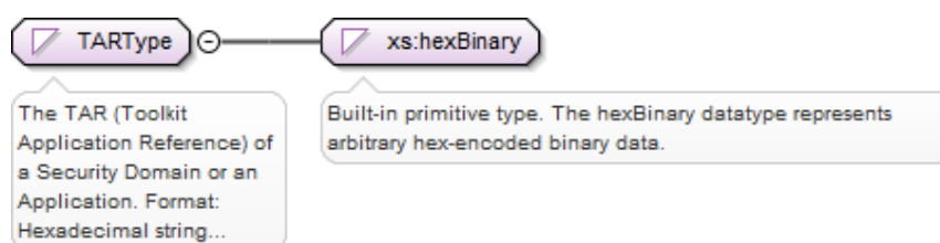
Figure 48: <rps:TARType>
