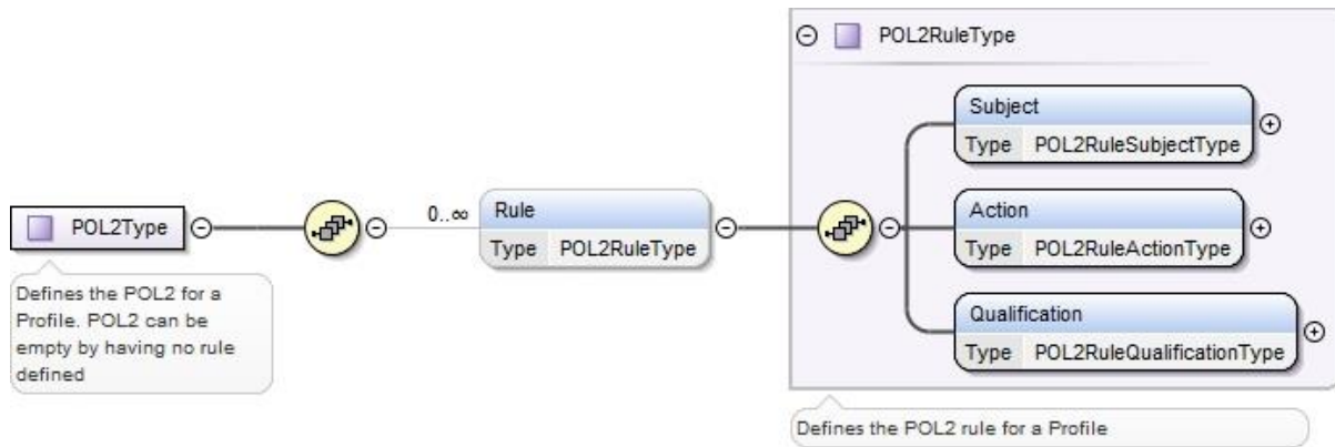
Figure 61: <rs:POL2Type>
