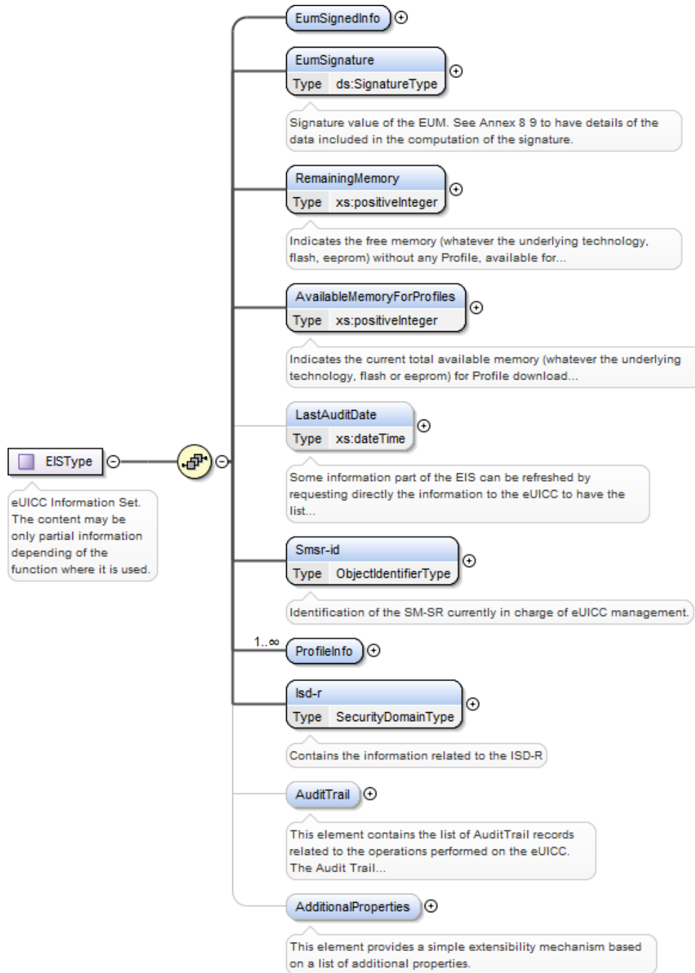
Figure 50: <rps: EISType >
