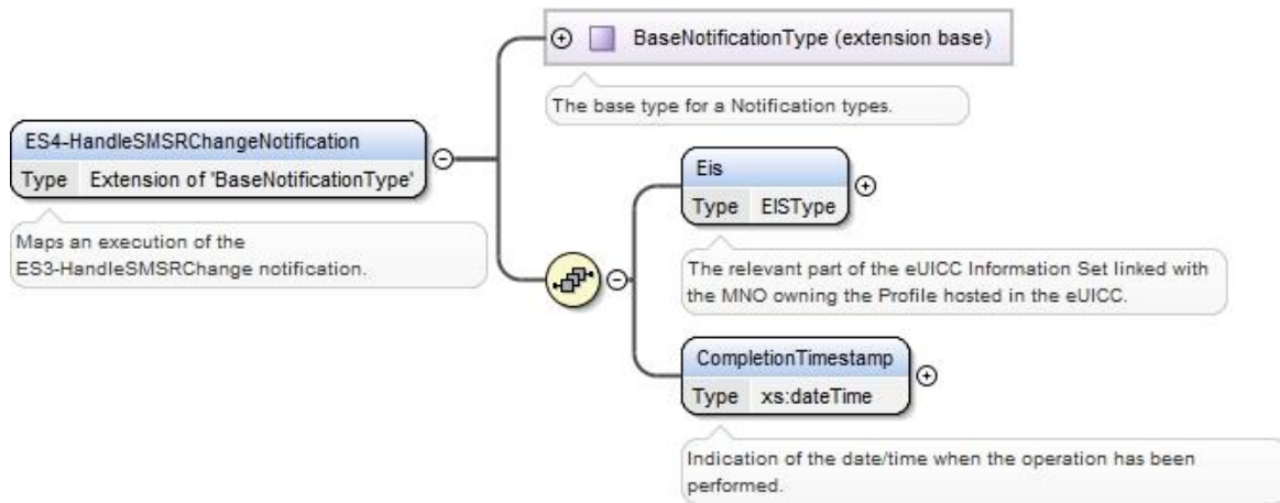
Figure 129: <rps:ES4-HandleSMSRChangeNotification>
