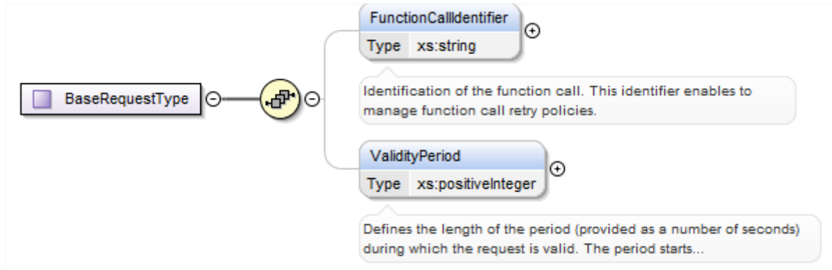
Figure 38: <rps:BaseRequestType>
