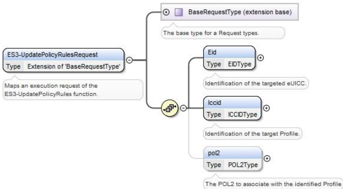
Figure 93: <rps:ES3-UpdatePolicyRulesRequest>
