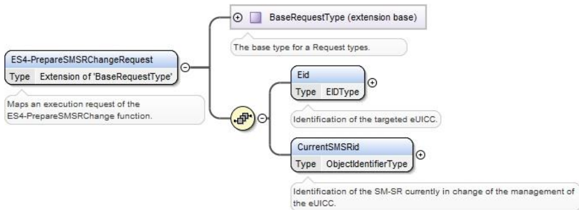
Figure 123: <rps:ES4-PrepareSMSRChangeRequest>
