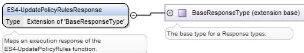
Figure 112: <rps:ES4-UpdatePolicyRulesResponse>
