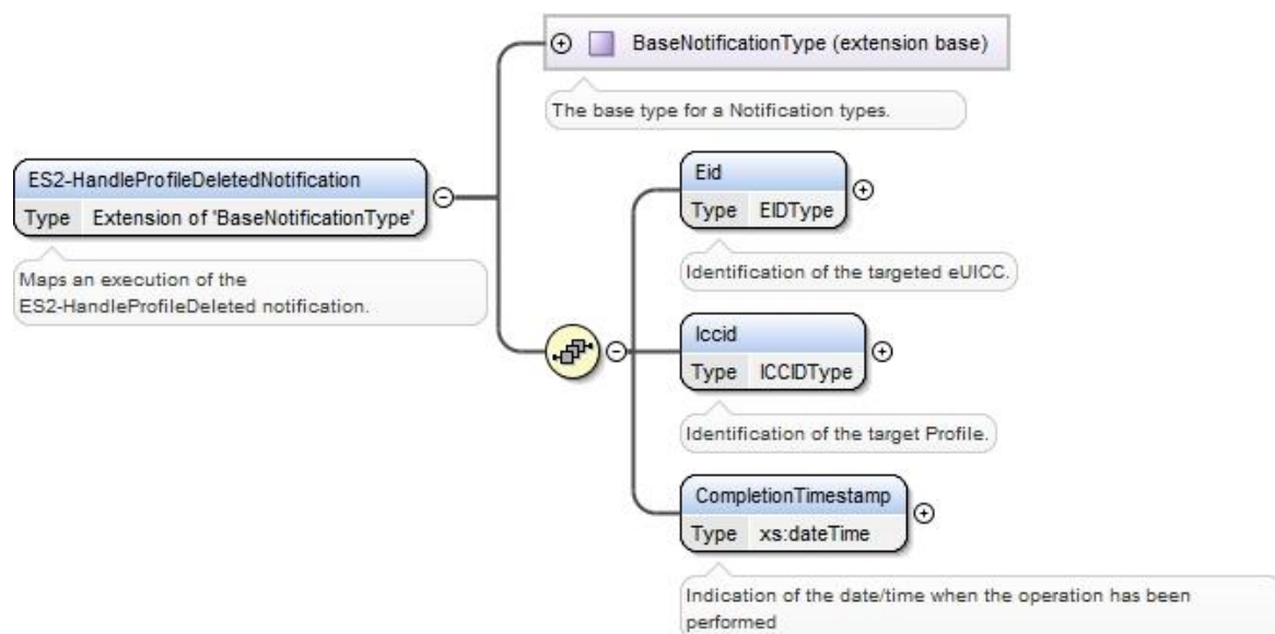
Figure 82: <rps:ES2-HandleProfileDeletedNotification >
