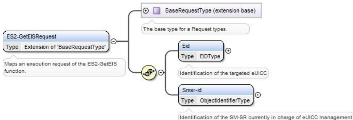
Figure 65: <rps:ES2-GetEISRequest>
