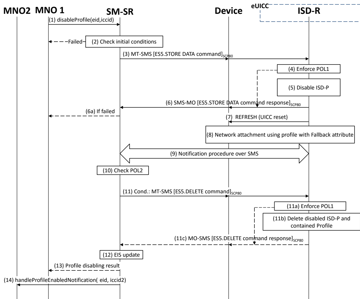
Figure 18: Profile Disabling
