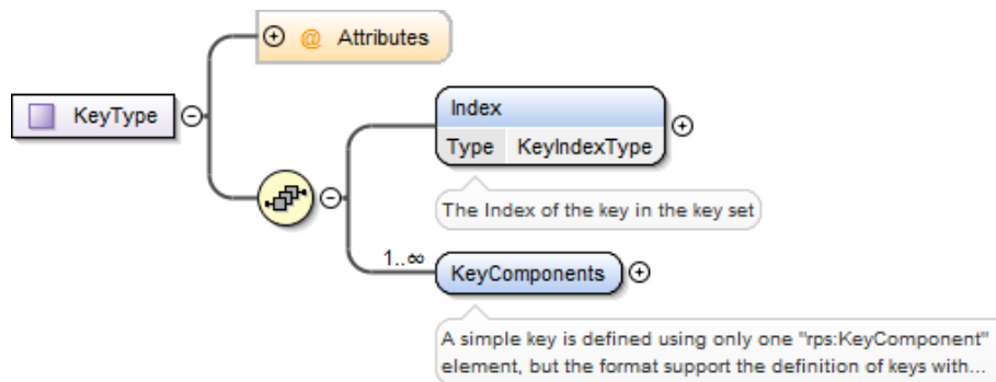
Figure 56: <rps:KeyType>
