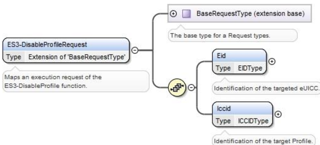
Figure 99: <rps:ES3-DisableProfile Request>
