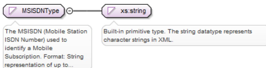
Figure 45: <rps:MSISDNType>
