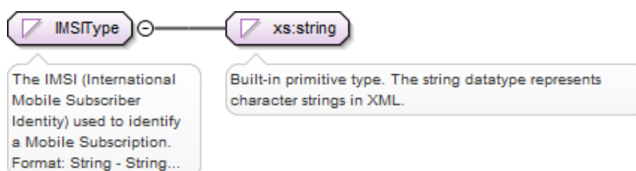
Figure 46: <rps:IMSIType>
