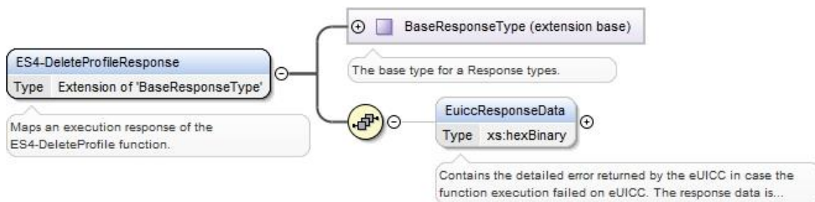
Figure 122: <rps:ES4-DeleteProfile Response>
