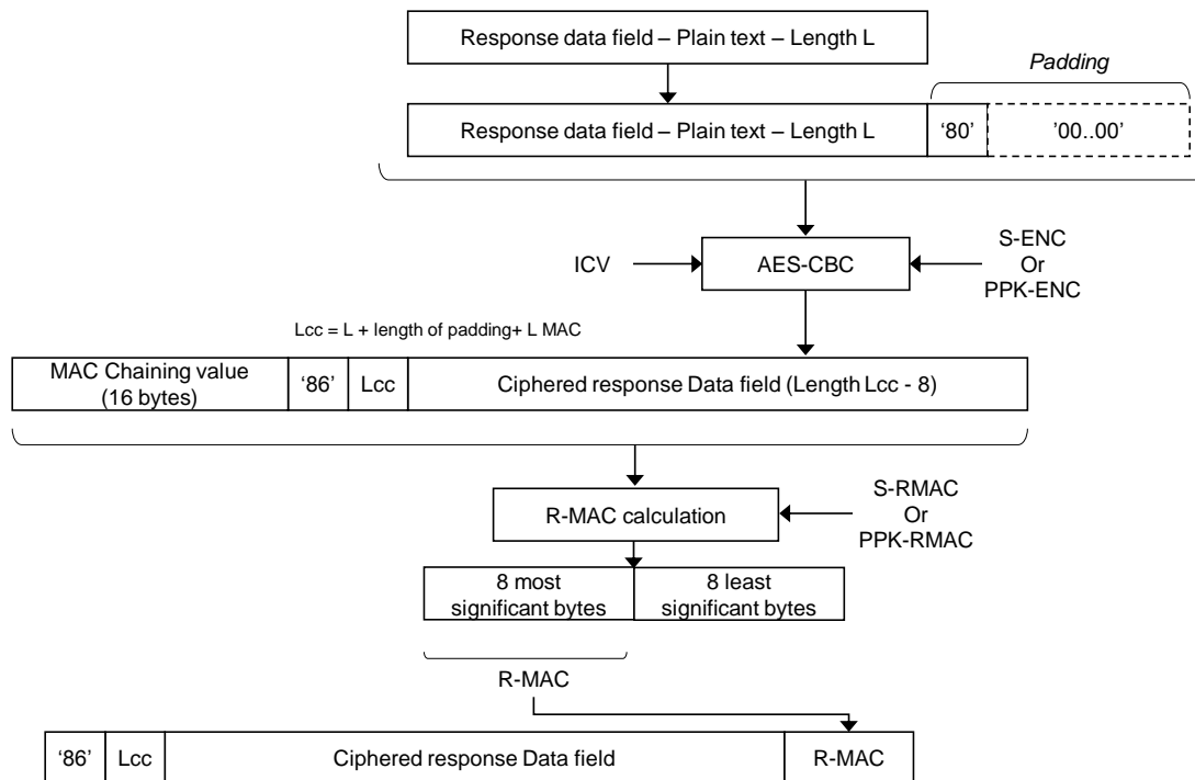
Figure 5: Building of Protected Response messages for BPP's TLV '86'
