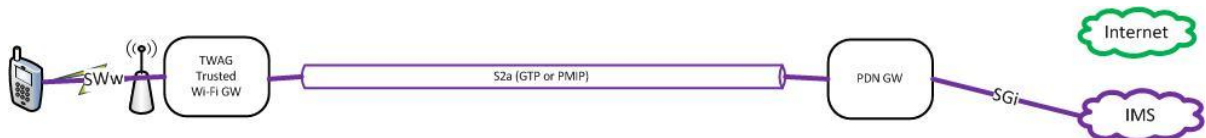
Figure 2 VoWiFi on trusted WLAN based on SWw and S2a (3GPP Rel-11 & SaMOG)
