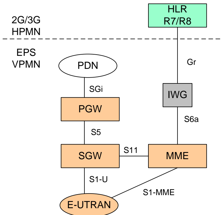
Figure 4.1.3-1: HPMN Legacy Roaming Architecture (local break-out)
