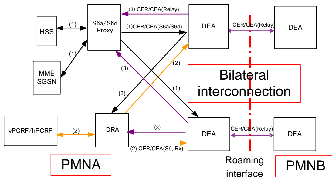
Figure B-1: Diameter architecture example 1
