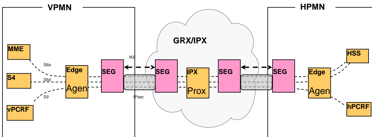
Figure 6.5.1-3: Security for IPX Service Hub connectivity
