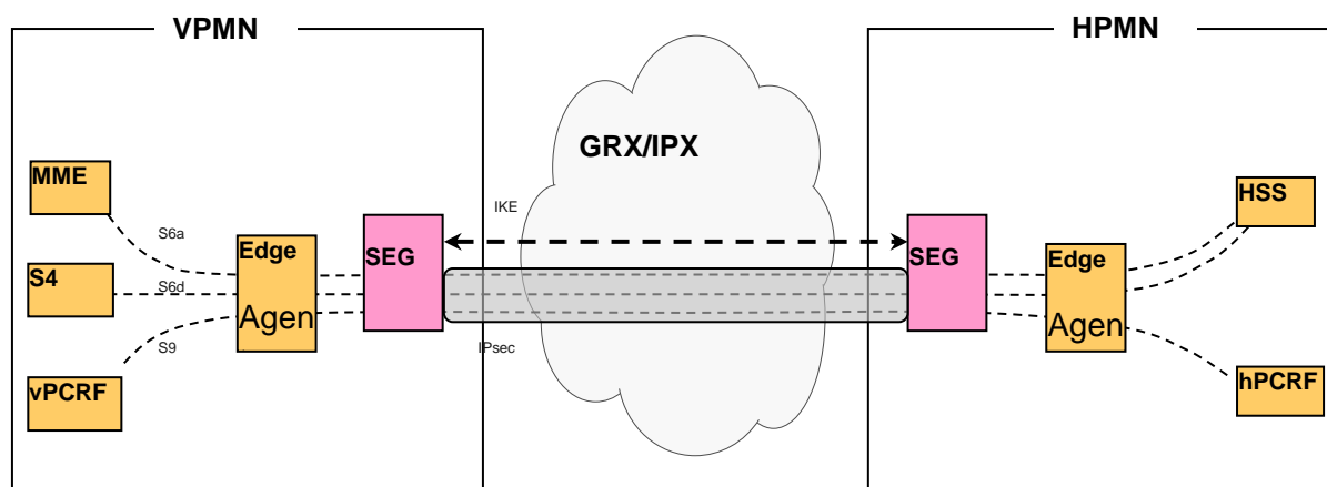
Figure 6.5.1-2: Security for IPX Transport connectivity
