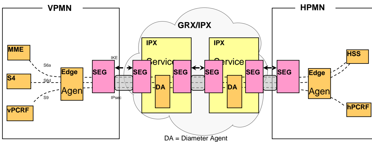
Figure 6.5.1-4: Security for connectivity with two IPX Service Hubs
