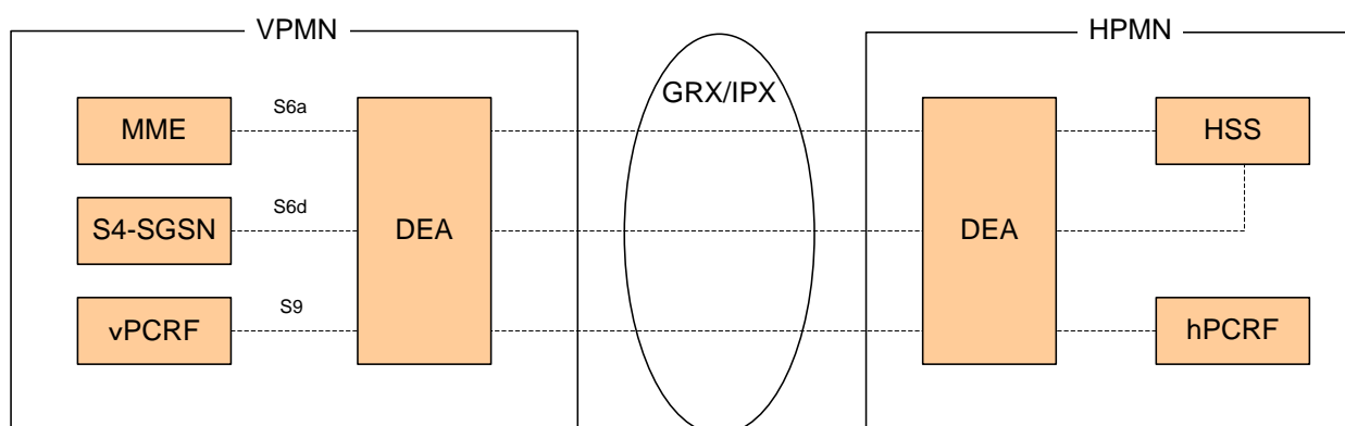
Figure 3.1.3.3-1: Diameter Roaming Implementation Architecture
