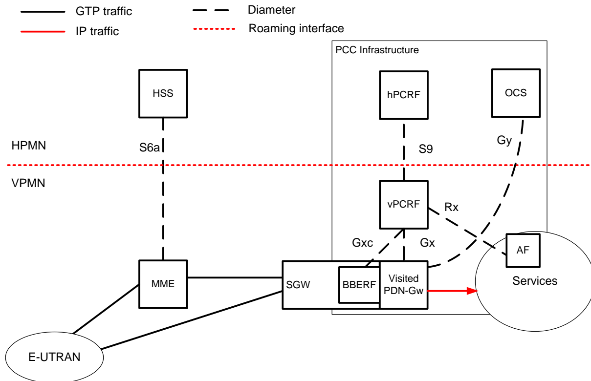
Figure 7.3-1: PCC Architecture with Local Break Out architecture
