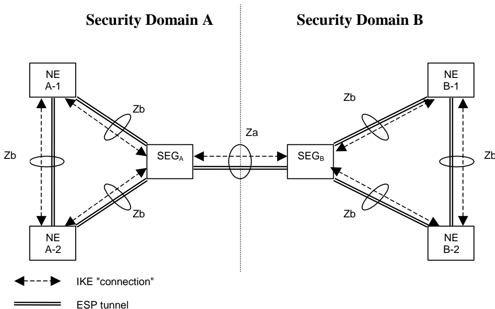
Figure 6.5.1-1: NDS/IP Architecture
