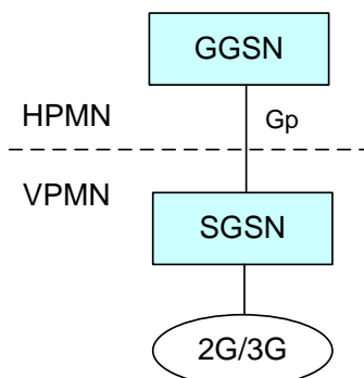
Figure 4.2.2.1-1: Scenario 1 - Legacy GPRS roaming
