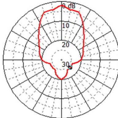
Figure 34: Horizontal pattern of alternative phased array antenna
