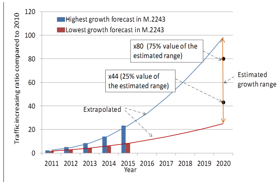
Figure A-3: Mobile traffic forecasts towards 2020 by extrapolation [Source: ITU 18 ]
