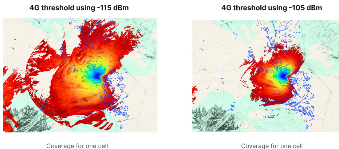
Figure 31 Coverage of a site using different signal-strength thresholds.
