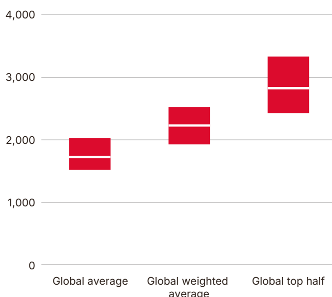
Figure 10: Total mid-band spectrum needs in 2035–2040, global (MHz)
