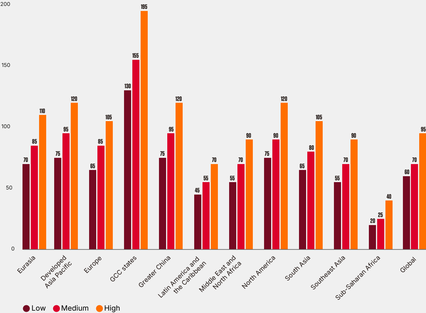
Figure A1: Regional traffic forecasts in low, medium and high growth scenarios, 2040 (GB/connections/month)
