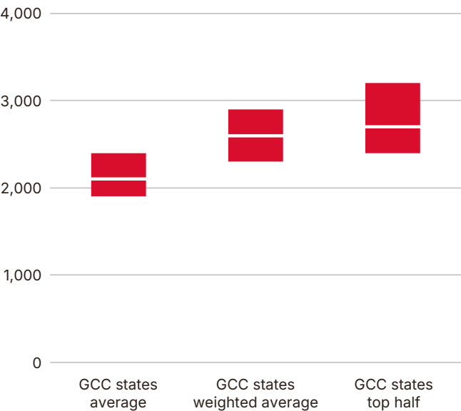
Figure 18: Total mid-band spectrum needs in 2035–2040, GCC states (MHz)
