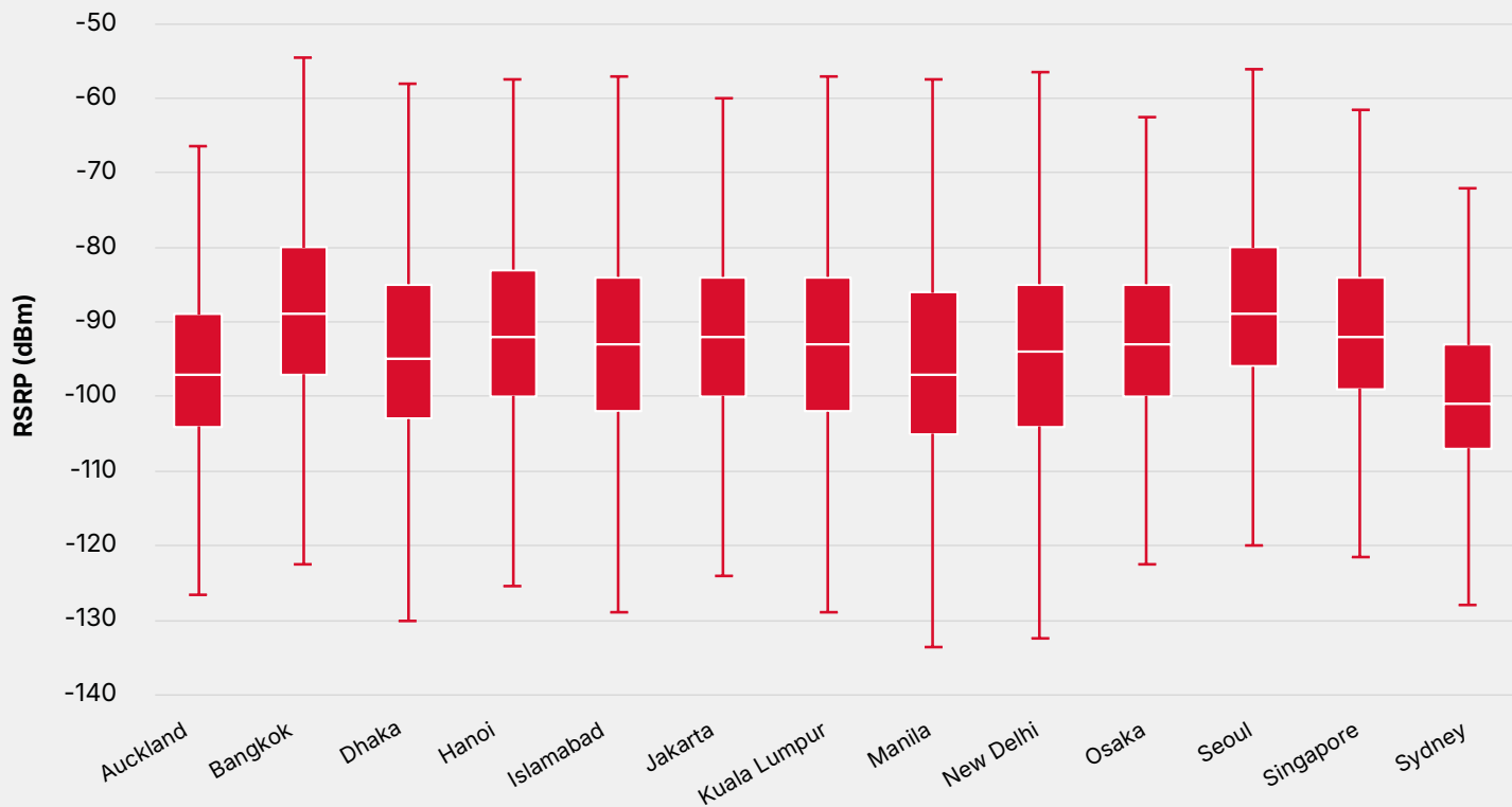
Figure 6 Indoor mid-band signal strength (4G/5G)
