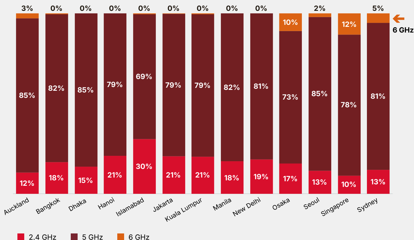
Figure 9 Distribution of Wi-Fi 6 / 6E and Wi-Fi 7 scans by band
