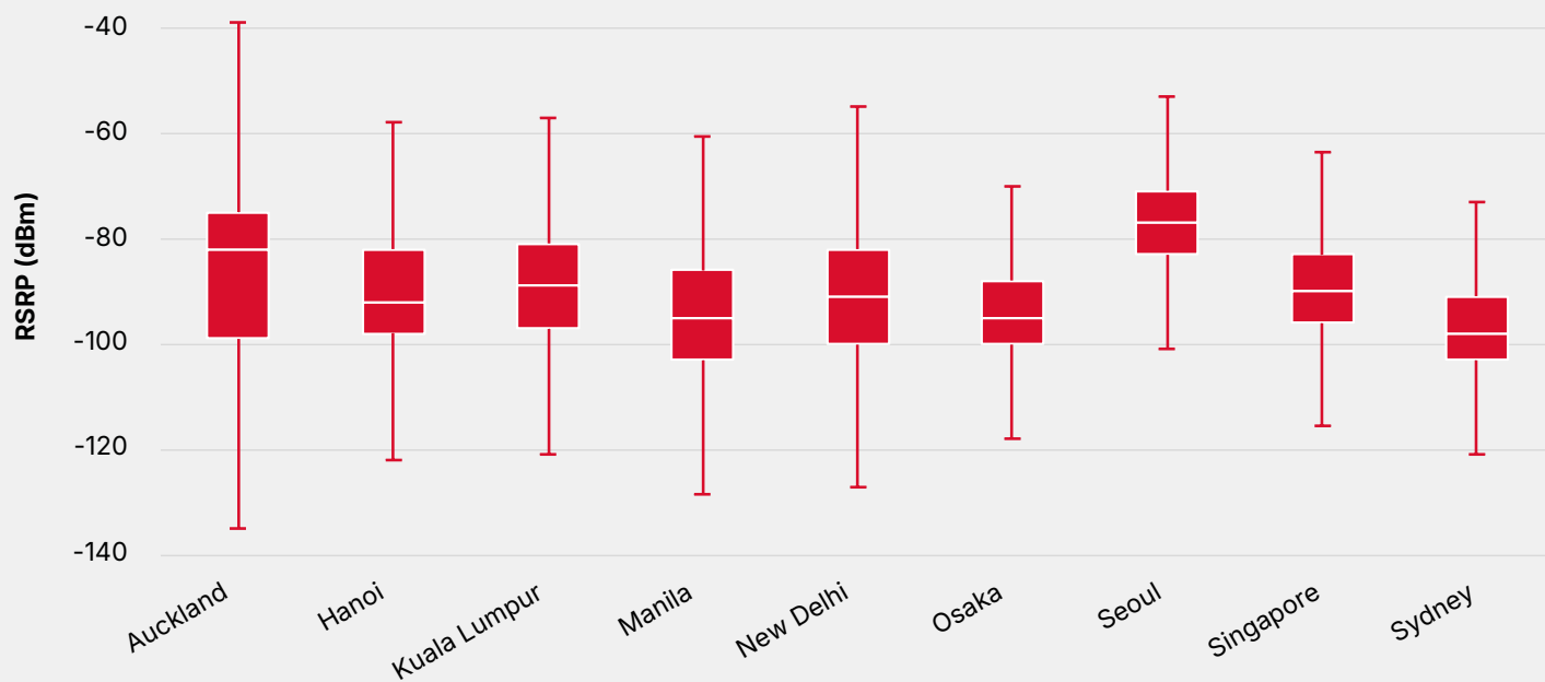
Figure 7 Indoor 3.5 GHz signal strength (5G)
