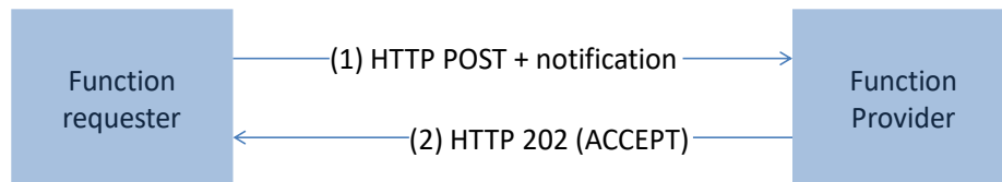
Figure 145: MEP: Synchronous Request-Response
