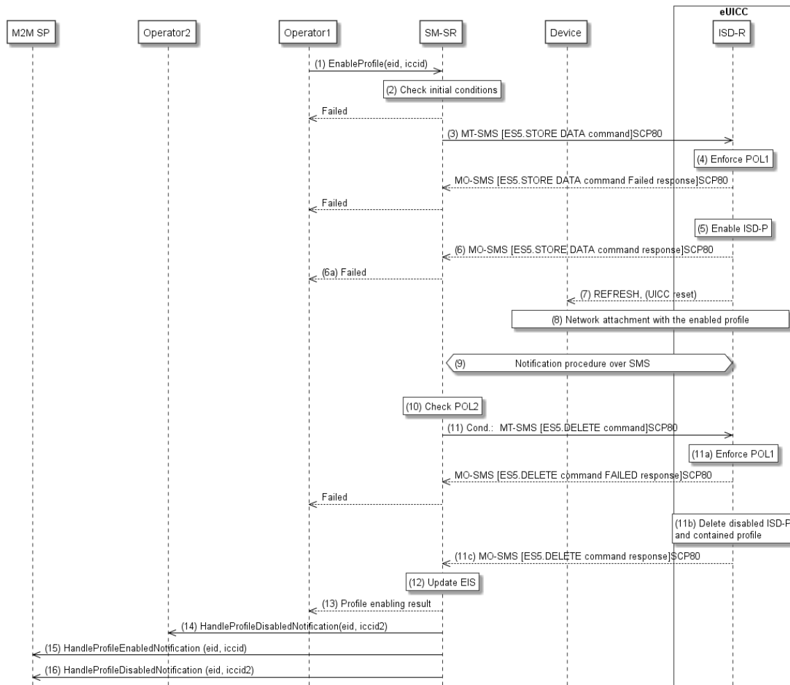
Figure 15: Profile Enabling, Success Case
