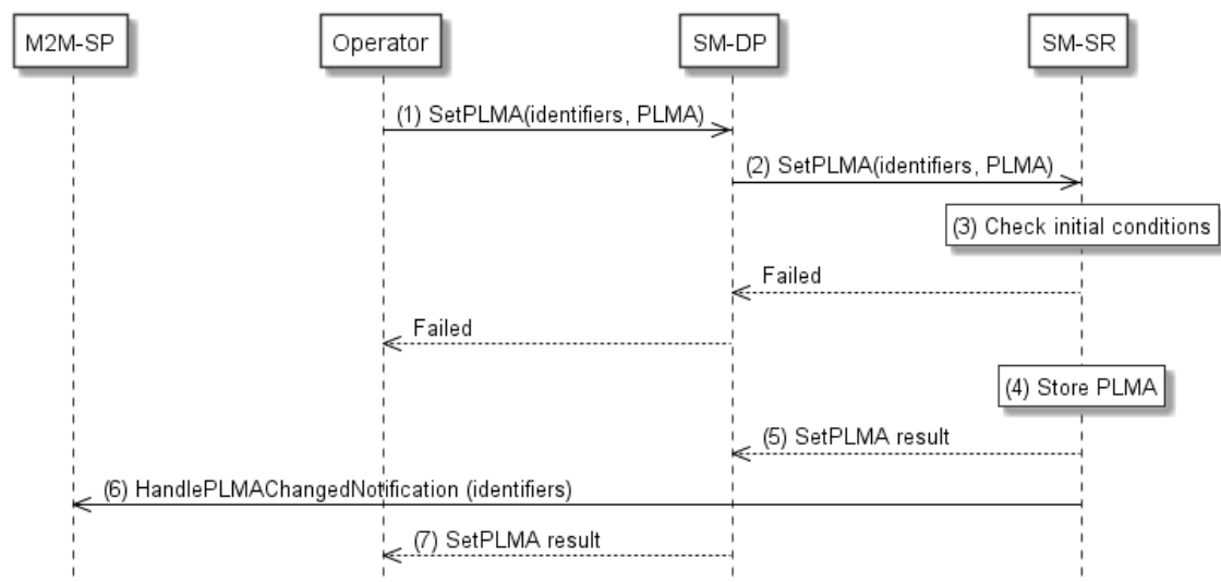
Figure 38: Set PLMA via SM-DP
