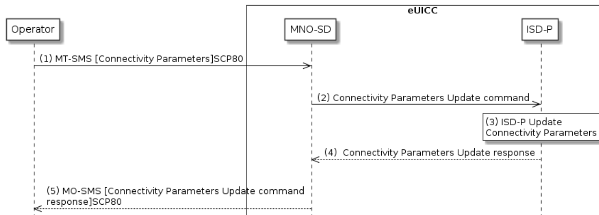
Figure 28: Connectivity Parameters Update by Operator
