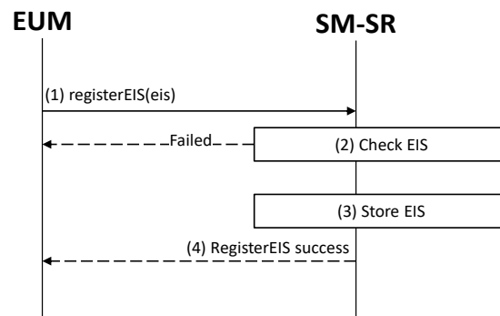
Figure 24: EIS Registration at SM-SR
