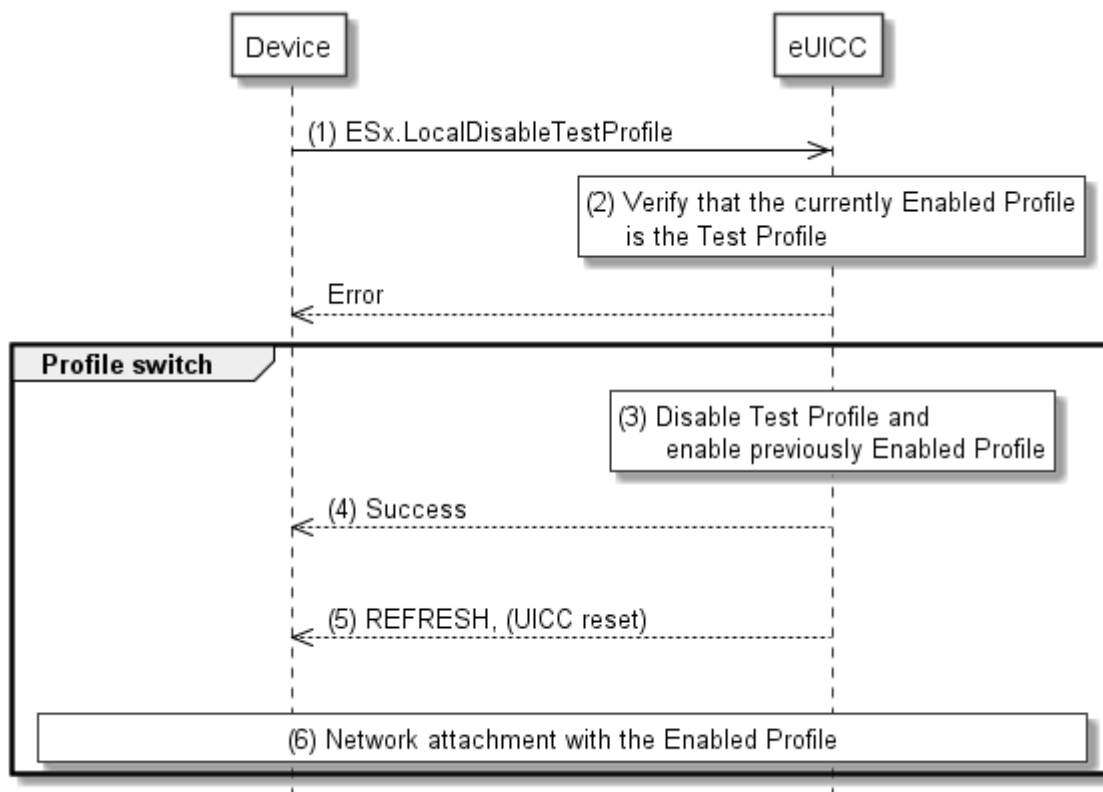
Figure 323: Local Disable of Test Profile
