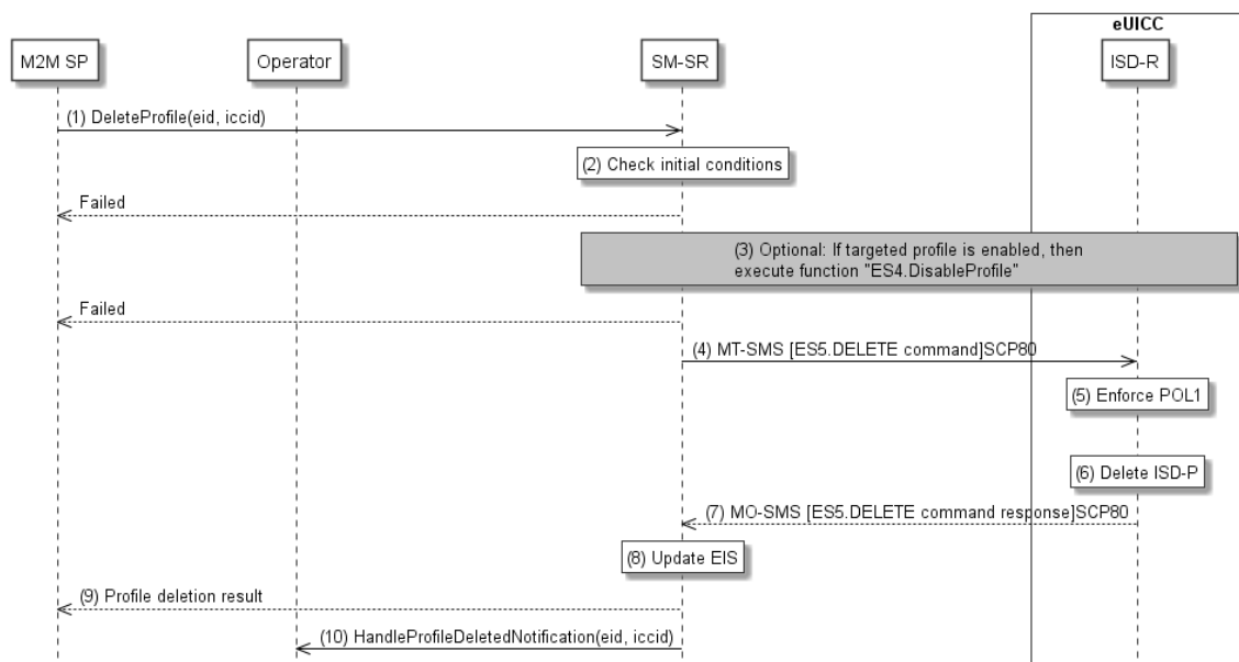
Figure 36: Profile and ISD-P Deletion via M2M SP
