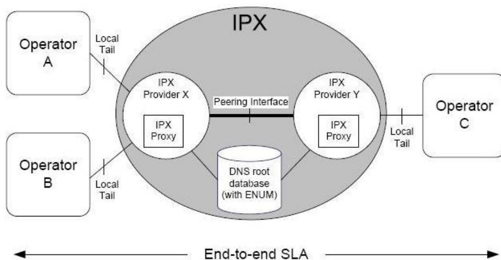
Figure 2: High-Level View of IPX (from IR.34)
