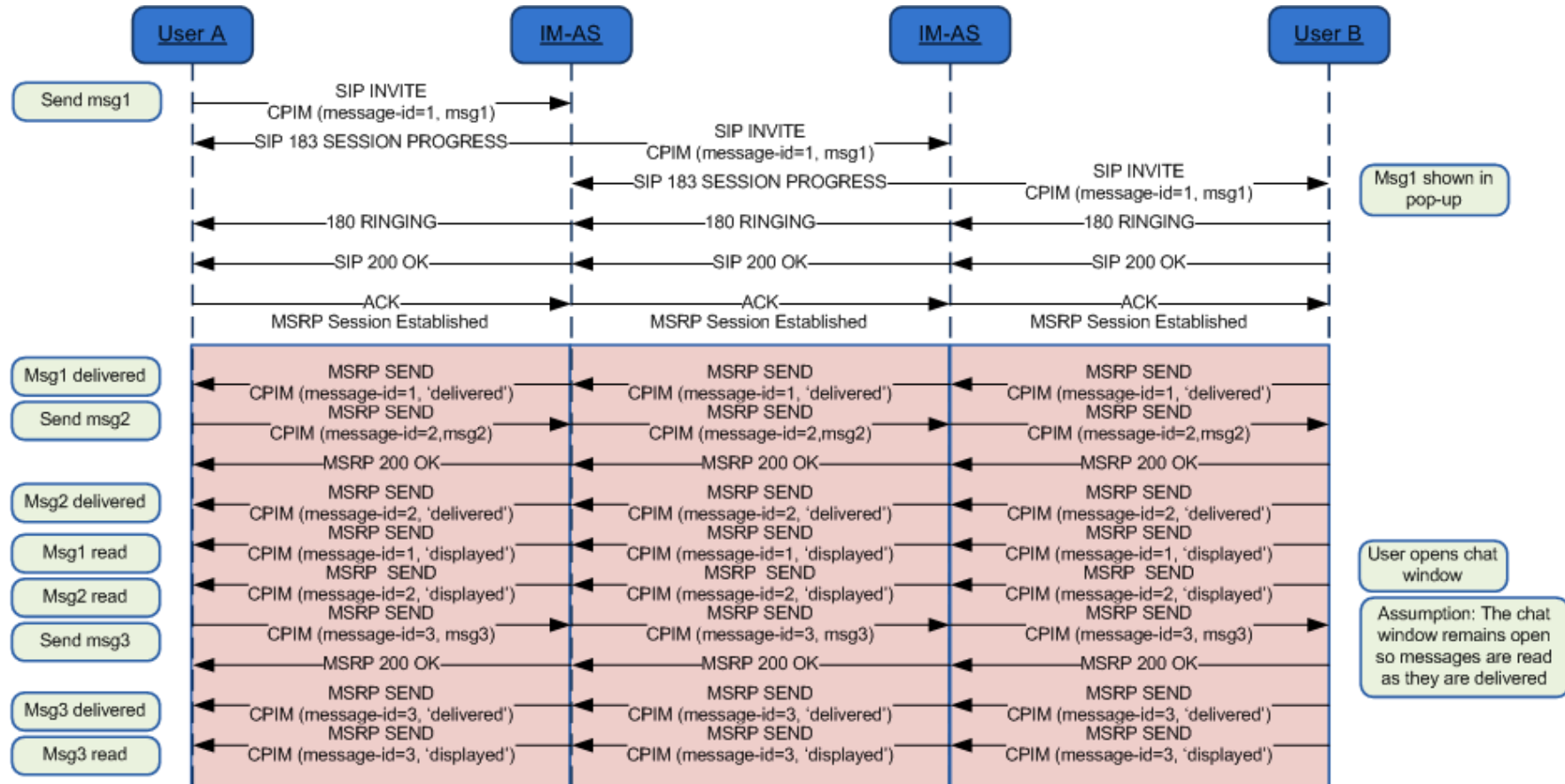
Figure 165: Chat flow without store and forward *
