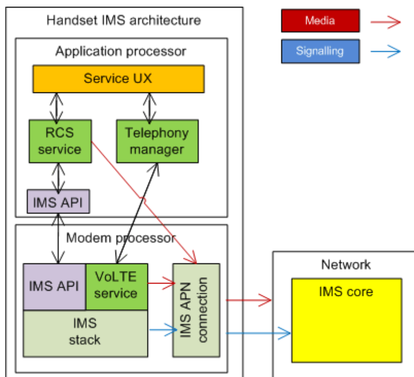
Figure 173: IMS API – single device stack architecture approach
