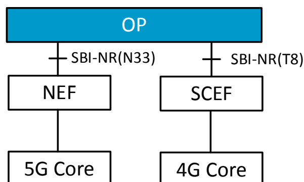
Figure 7: Functional mapping between OP and NEF/SCEF
