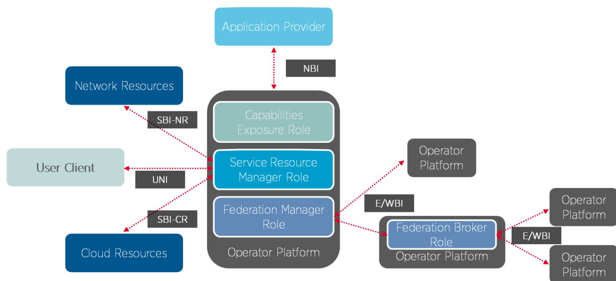
Figure 2: OP Roles and Interfaces Reference Architecture
