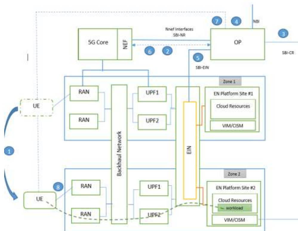
Figure 14: OP Application Relocation flow
