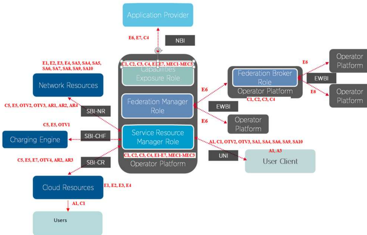
Figure 31: OP Threat Vectors
