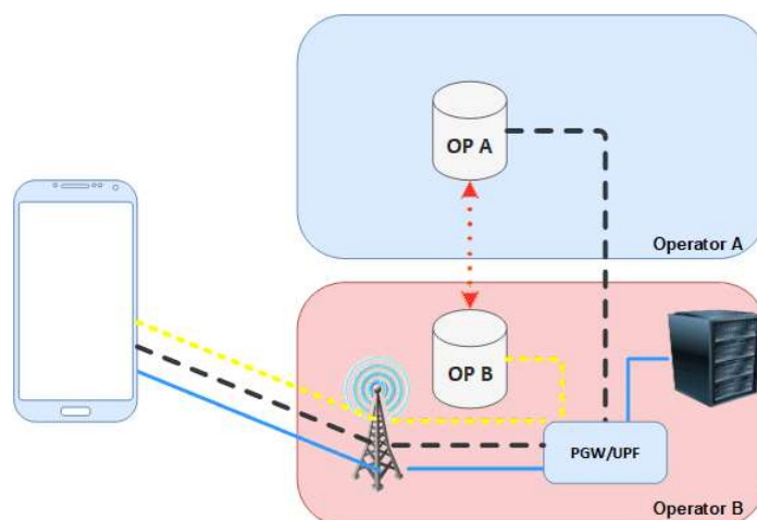
Figure 11: Roaming access to OP and edge resource – local breakout
