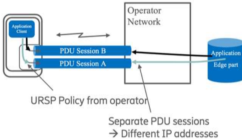
Figure 32: URSP mapping to operator services
