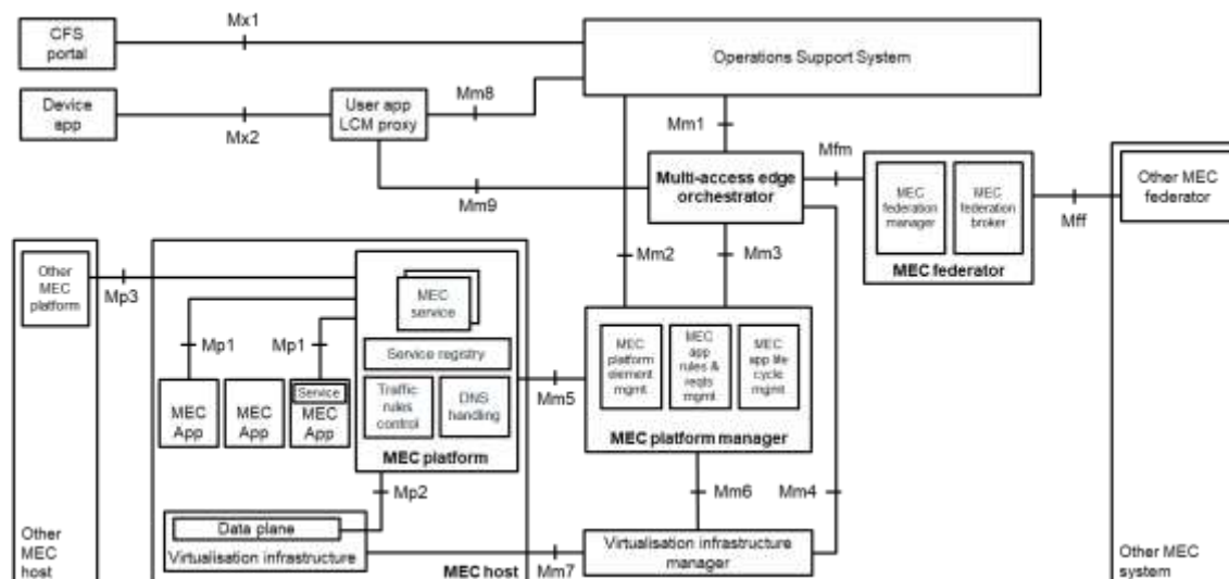
Figure 24: Multi-access edge system reference architecture variant for MEC federation in ETSI MEC003 [18]
