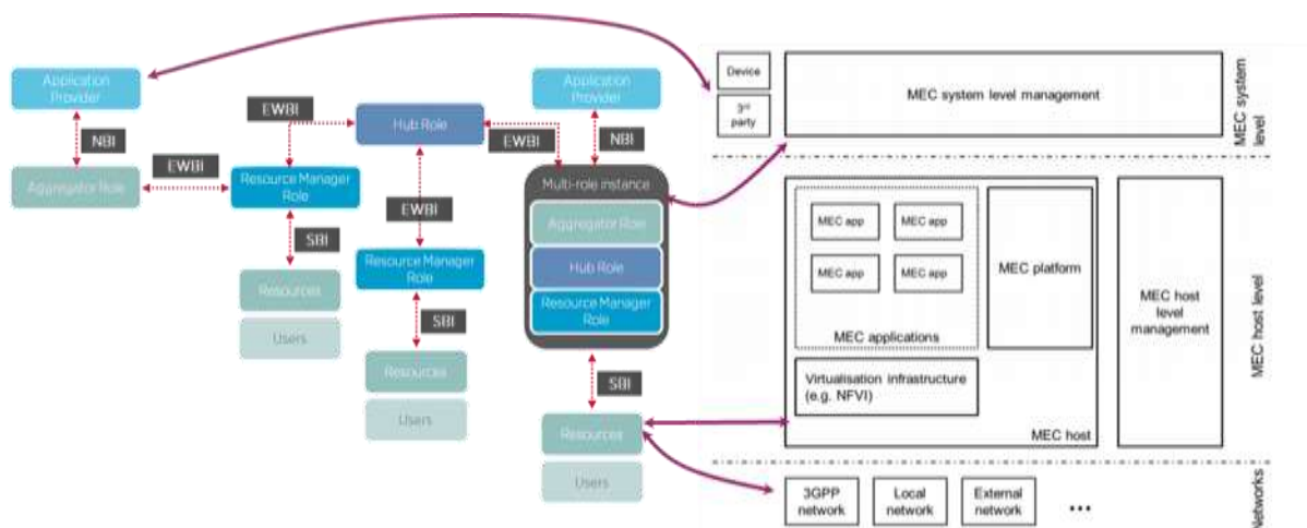
Figure 29: OP to ETSI ISG MEC mapping
