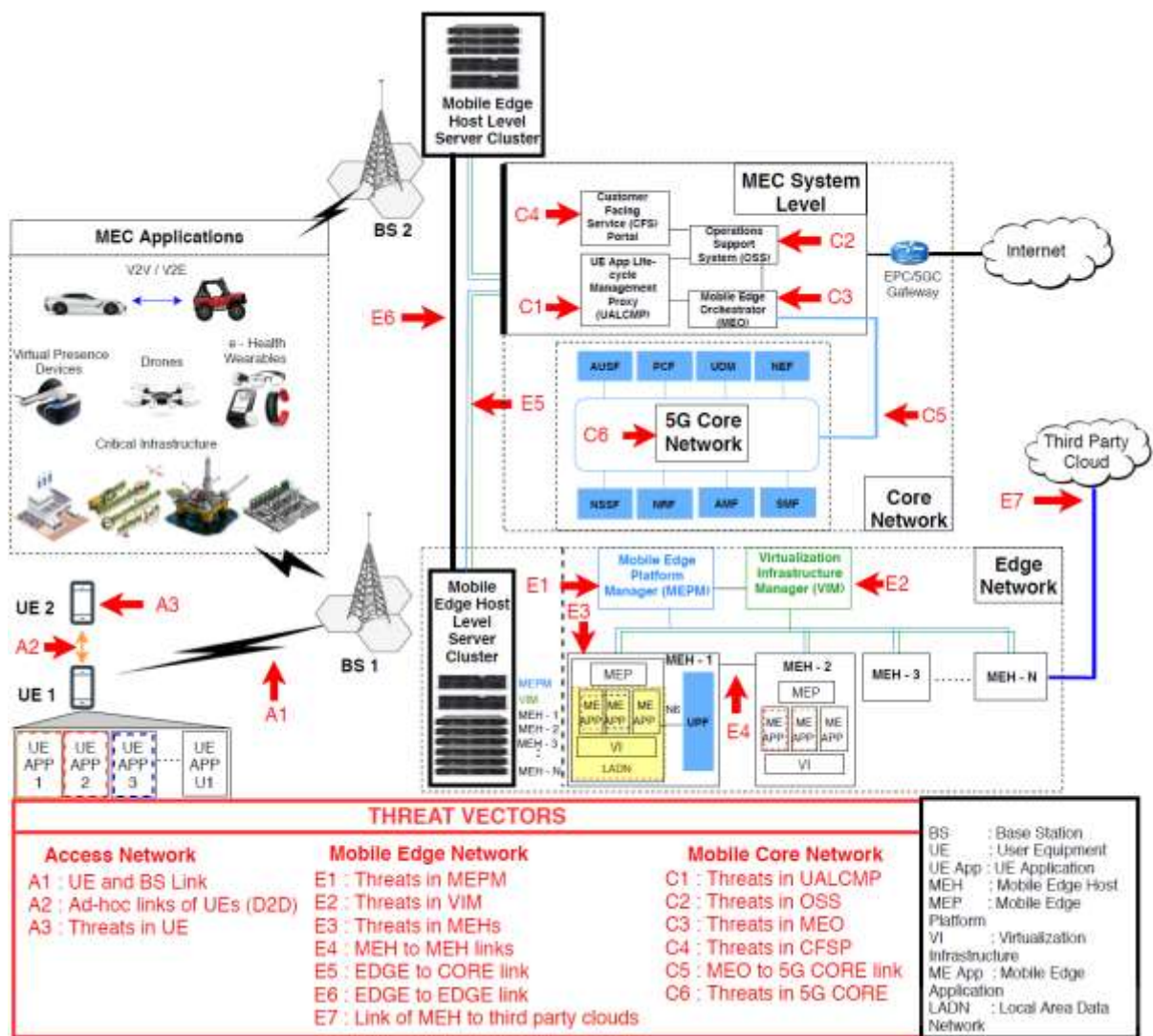
Figure 30: ETSI ISG MEC Access, Edge and Core Threat Vectors (from [15])
