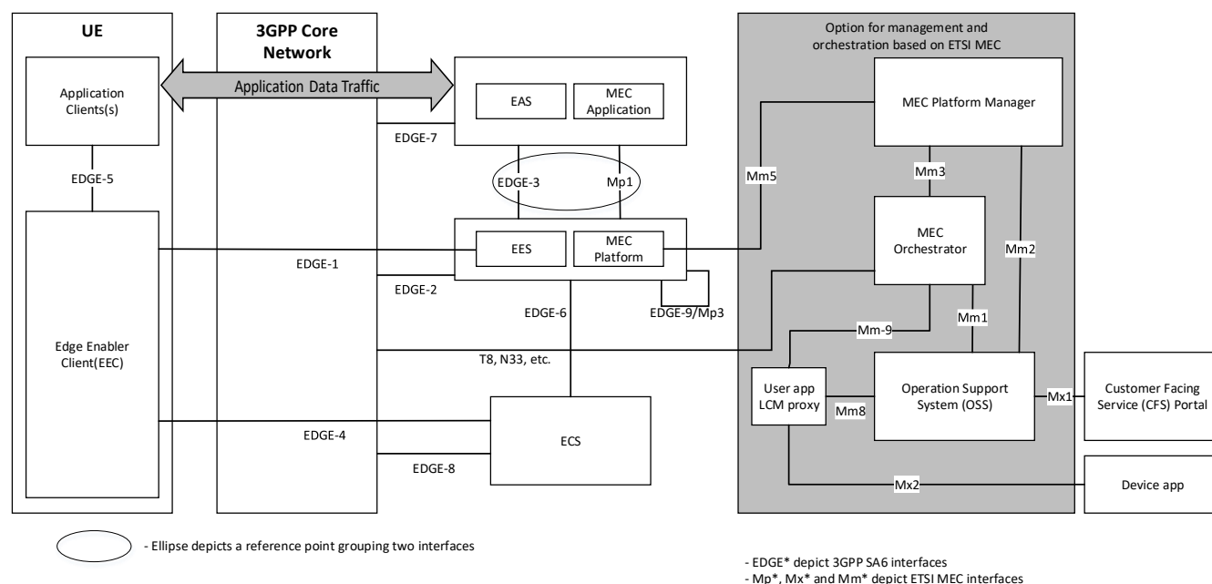
Figure 23: Relationship between ETSI ISG-MEC and 3GPP EDGEAPP architectures [17]
