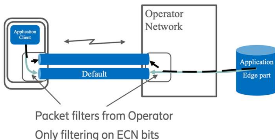
Figure 34: L4S based queue selection
