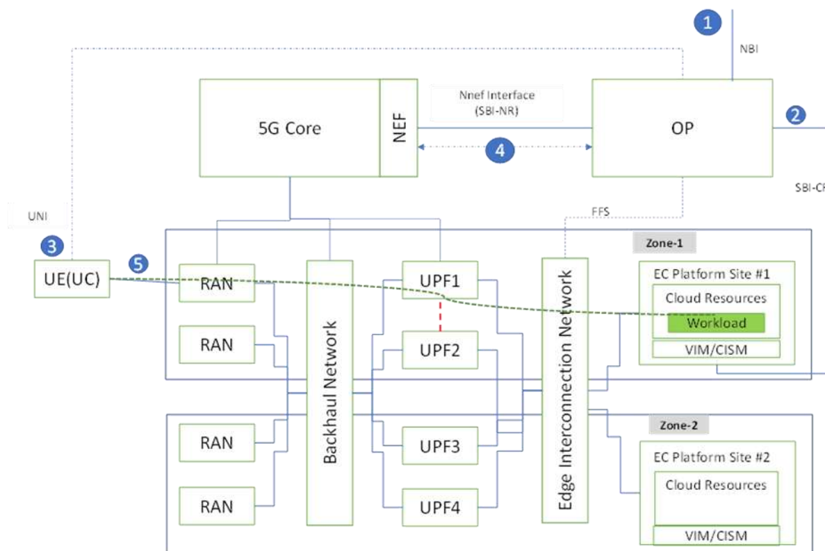
Figure 13: OP SBI-NR Subscription flow
