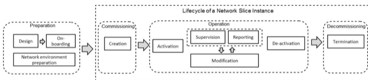
Figure 38: Management aspects of network slicing [34]
