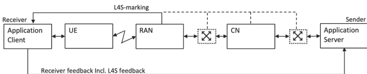
Figure 33: L4S handling
