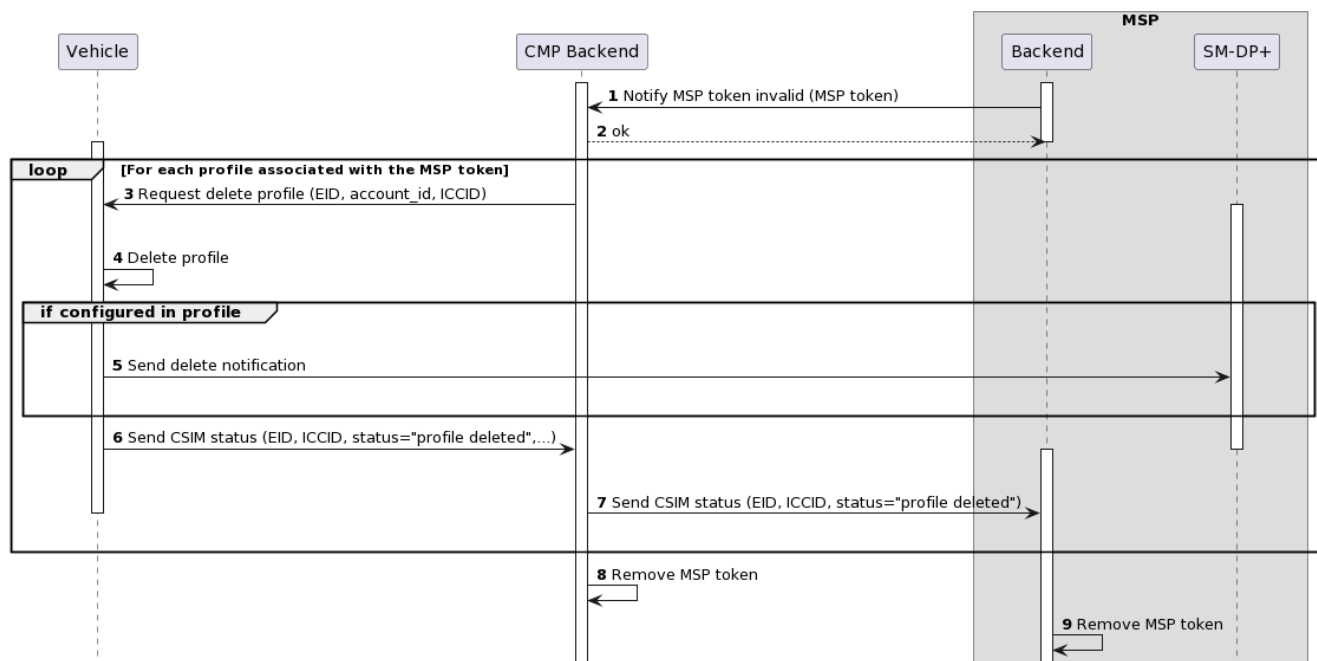
Figure 9 Withdraw Onboarding via MSP Touchpoint
