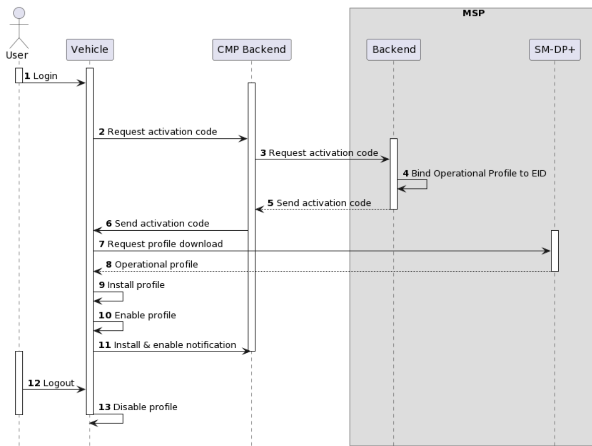
Figure 6: Car Provisioning Procedure
