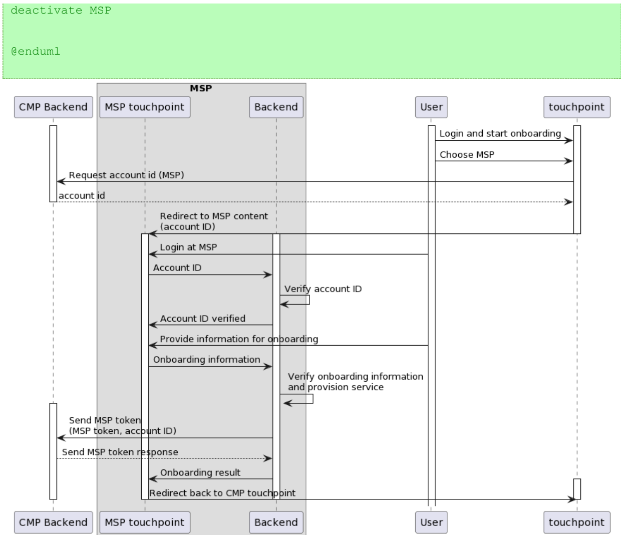
Figure 4: MSP Onboarding via CMP Touchpoint procedure
