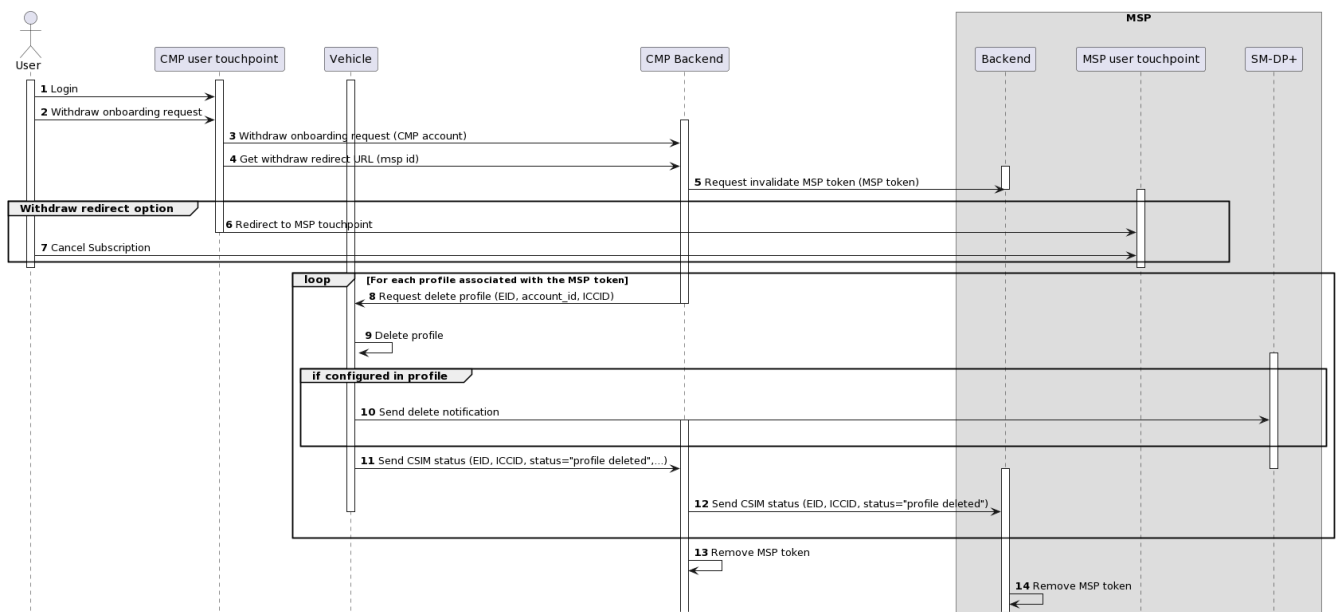
Figure 8 Withdraw Onboarding via CMP Touchpoint
