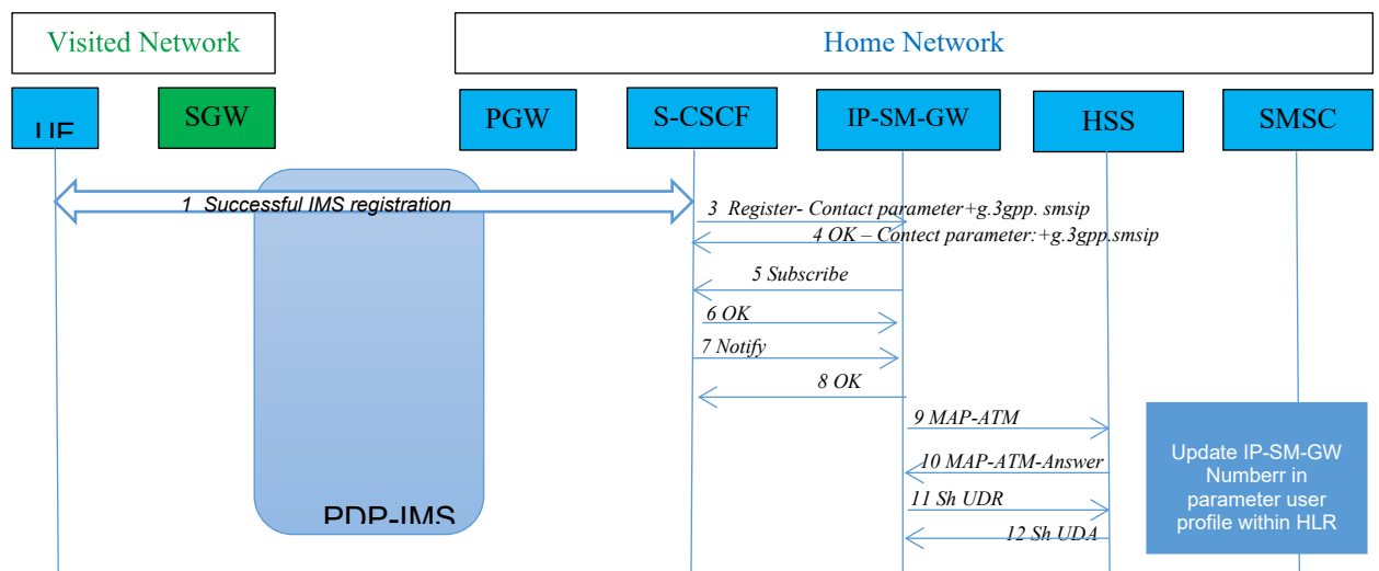
Figure 4: IMS Registration
