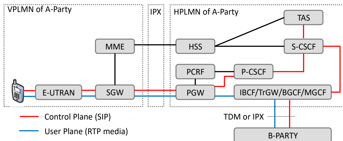
Figure 5: S8HR architecture
