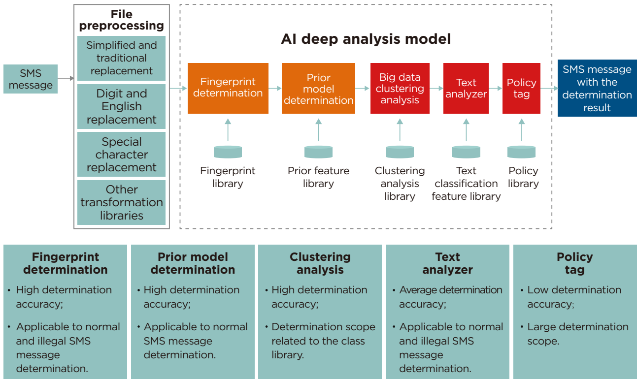
Figure 3-36 AI-based comprehensive junk SMS message determination model
