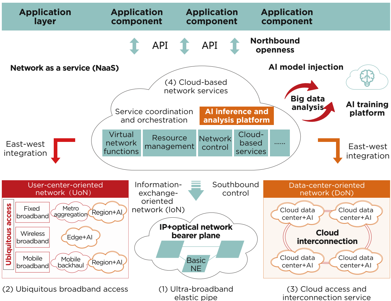
Figure 1-5 Architecture of China Unicom's CUBE-Net2.0+ network
