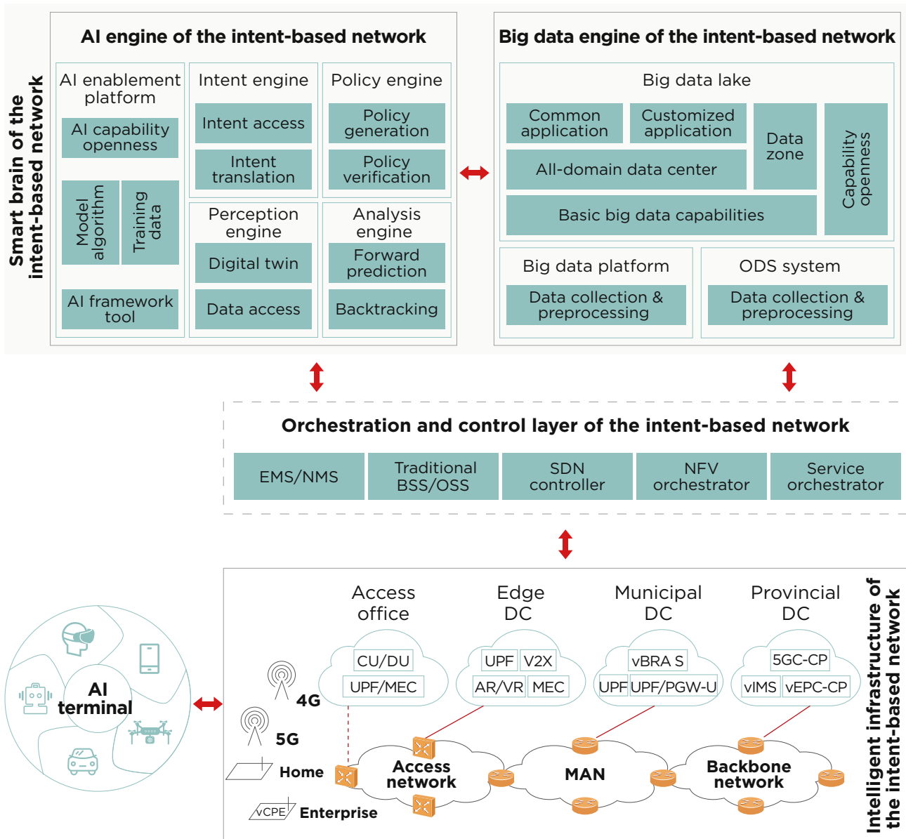
Figure 1-4 Target architecture of China Telecom's intent-based network
