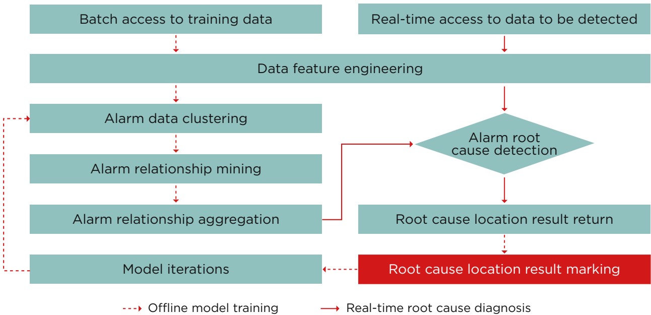
Figure 3-11 Intelligent alarm RCA process
