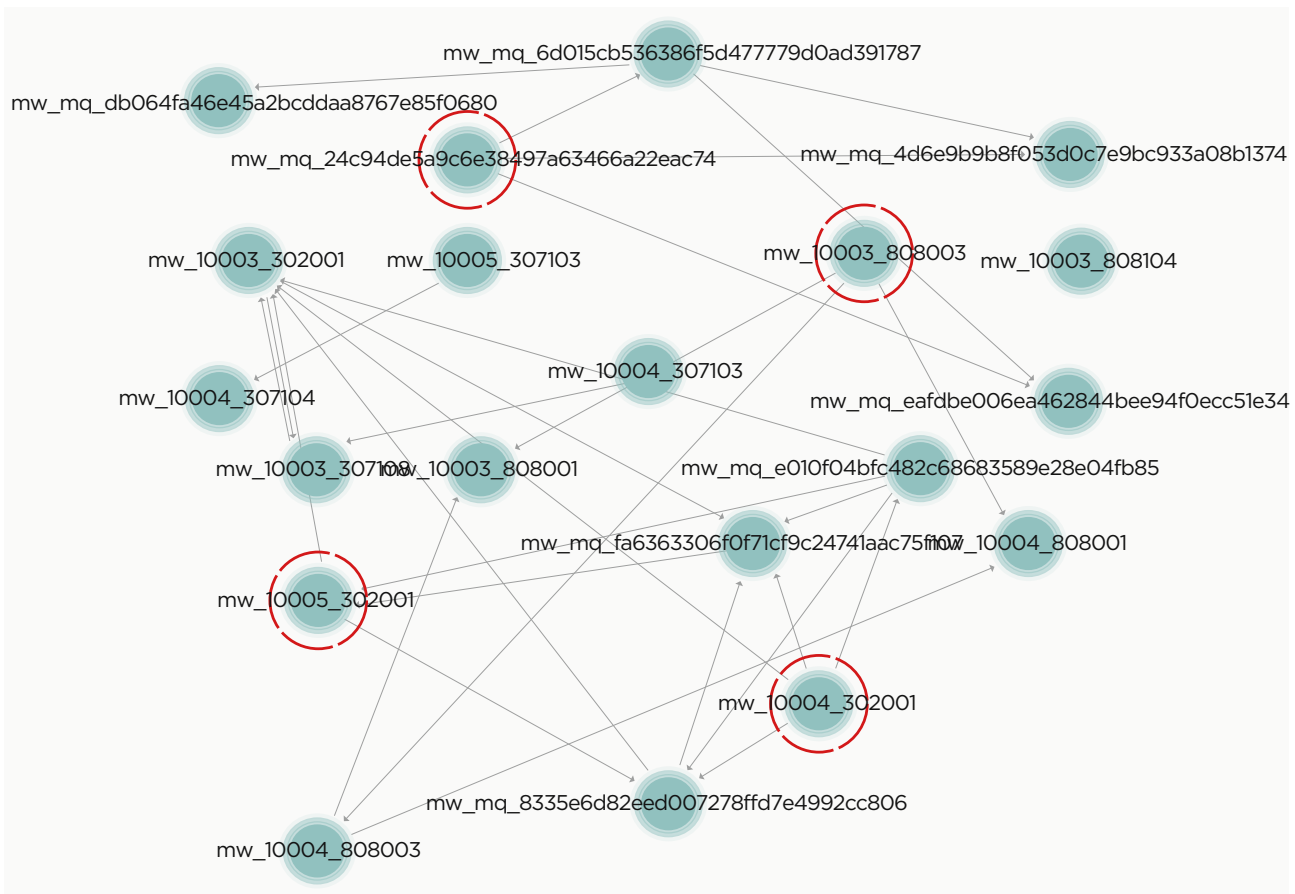
Figure 3-12 Example of the alarm relationship map
