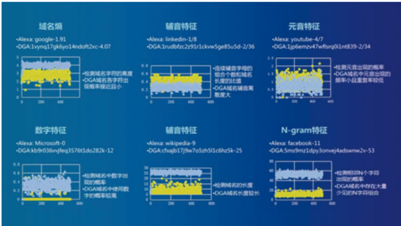
Figure 3-42 Comparison of feature vector modeling data between C&C server domain names and normal domain names
