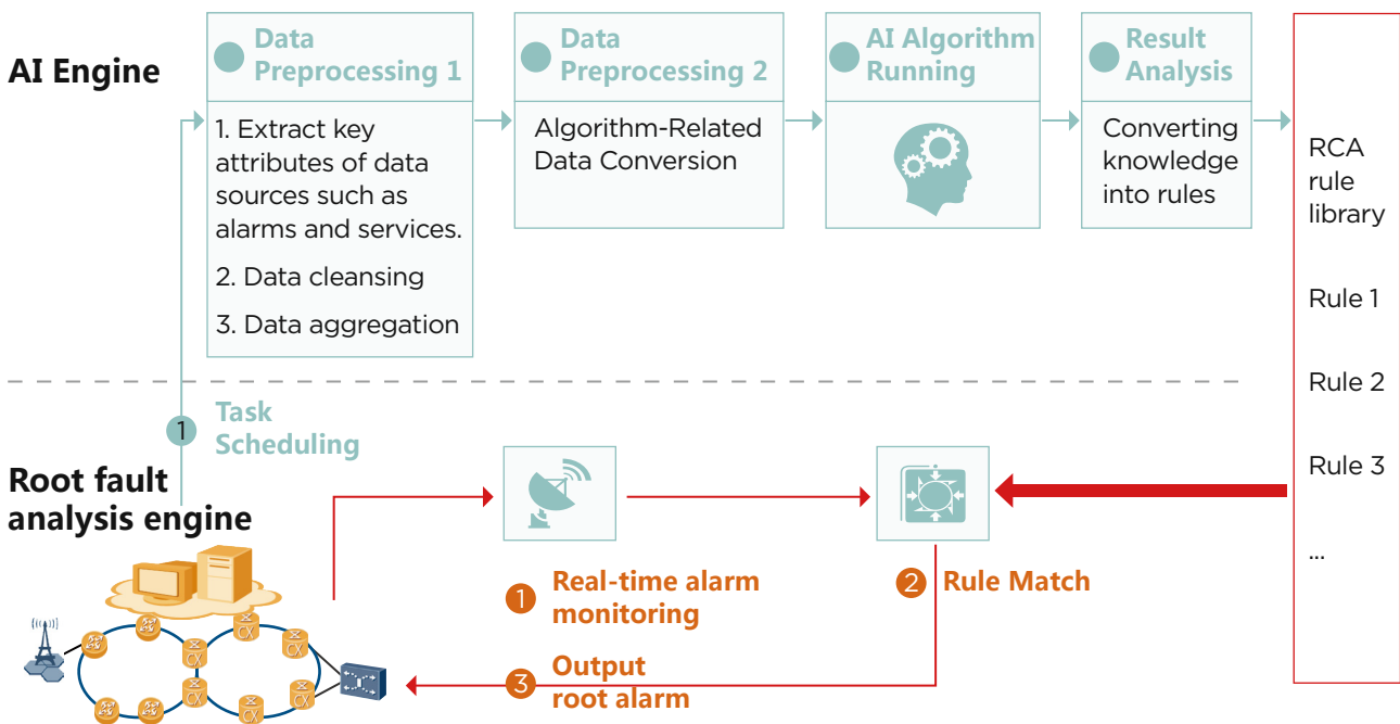
Figure Alarm Root Cause Analysis Process
