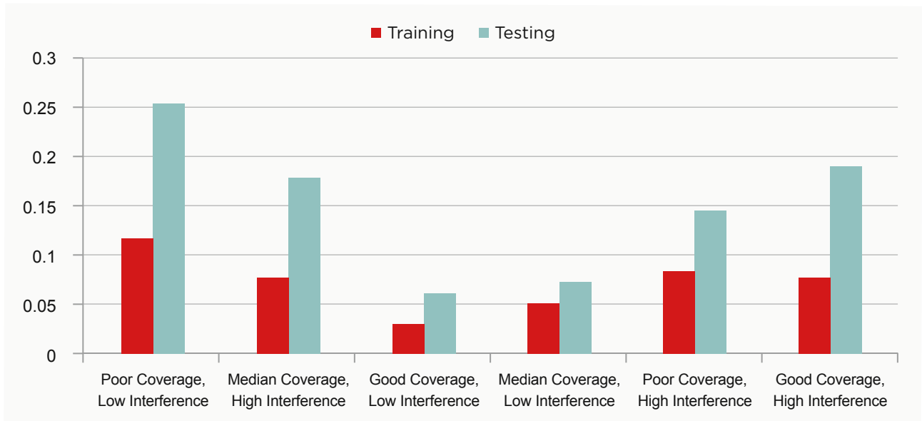
Figure 3-30 Data simulation performance
