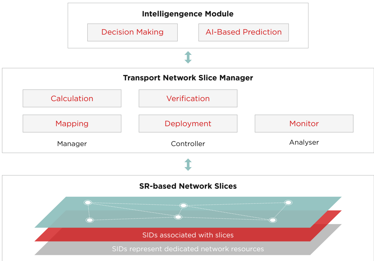
Figure 3-25 System structure of the TNSM
