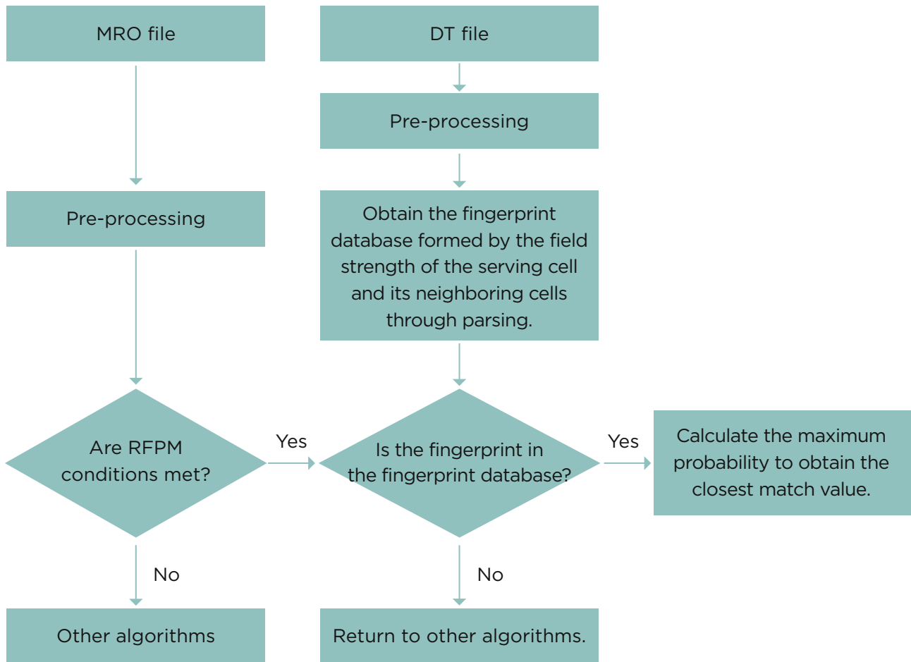
Figure 3-2 Fingerprint database algorithm selection process based on neural networks
