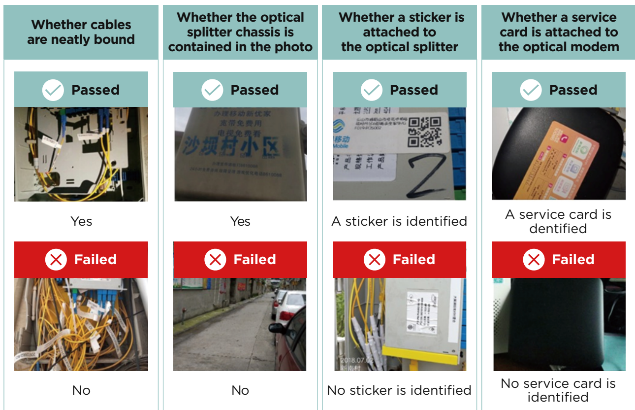
Figure 3-7 Quality inspection of basic installation techniques
