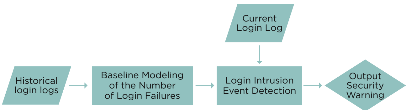
• Login Intrusion Detection Flow
