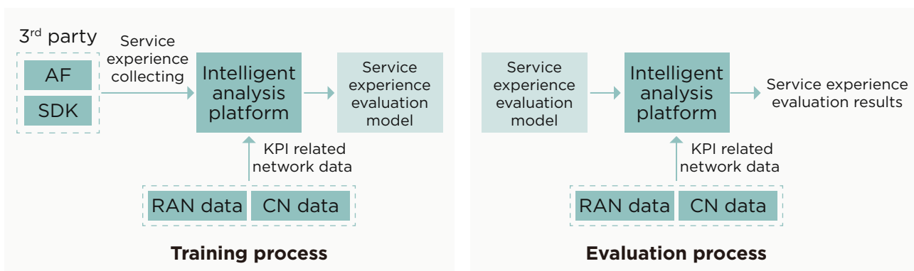
Figure 3-28 Process of offline training and online evaluation
