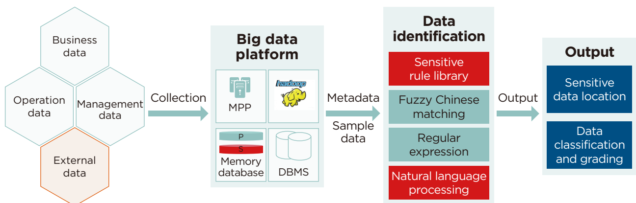
Figure 3-38 System processing flow
