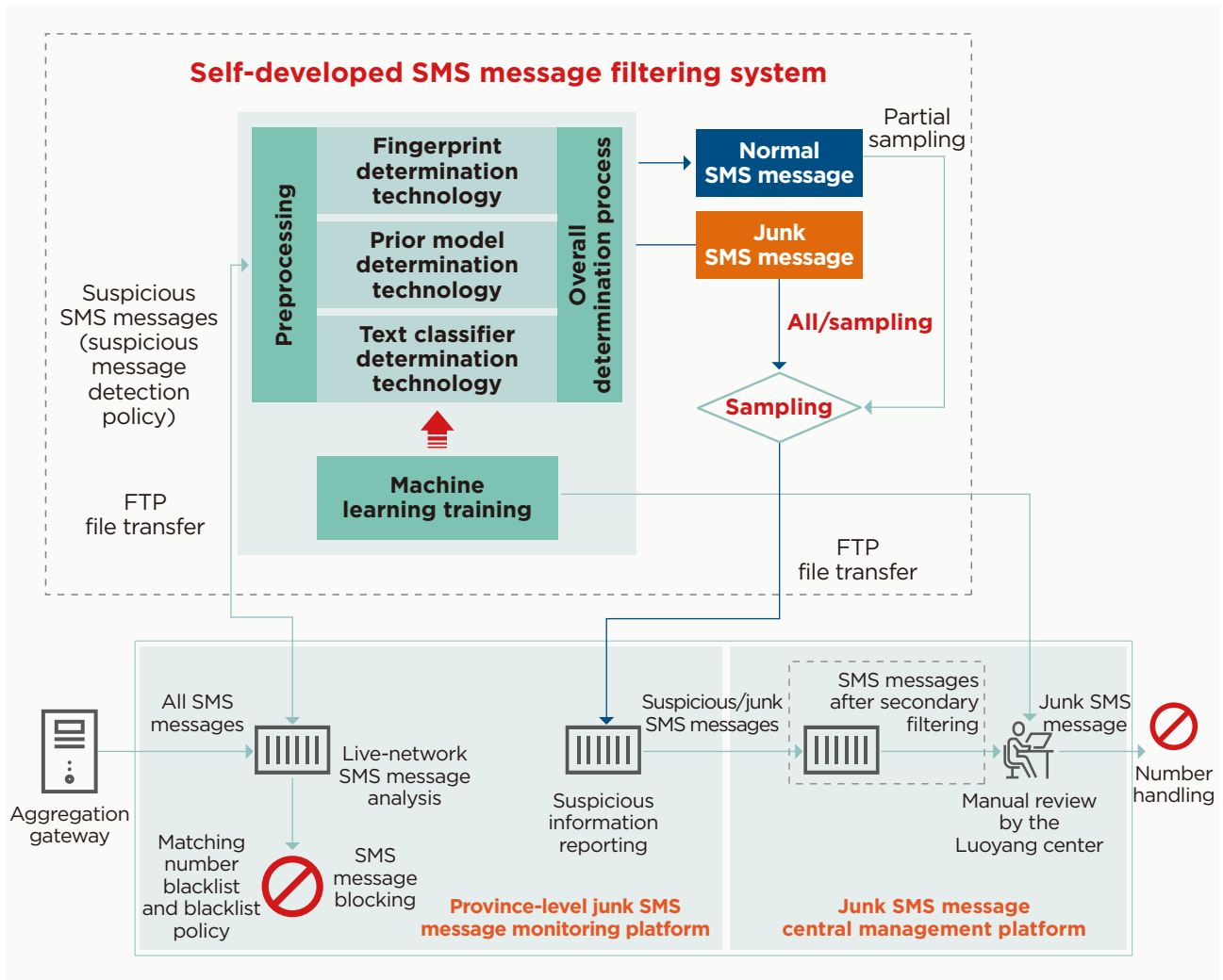
Figure 3-34 Overall architecture of the intelligent junk SMS message analysis and optimization system
