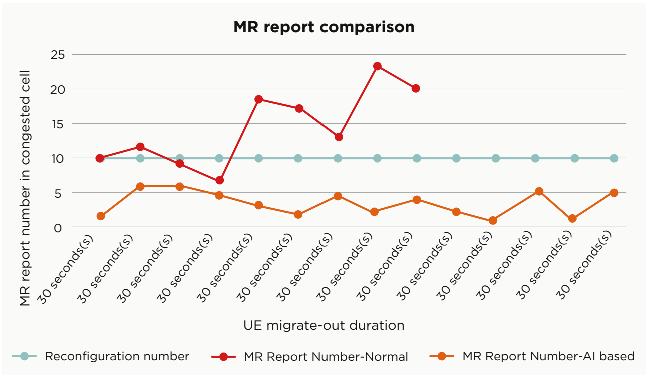
Figure Comparison of MR Report Number in Load Balancing Test Result
