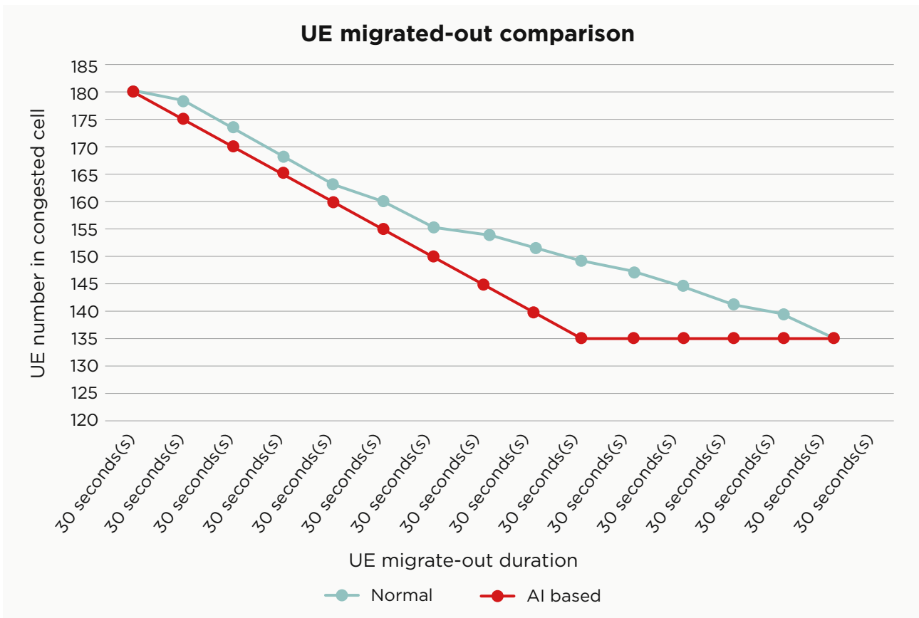
Figure Test Result of Load Balancing -UE Migrate-out Speed
