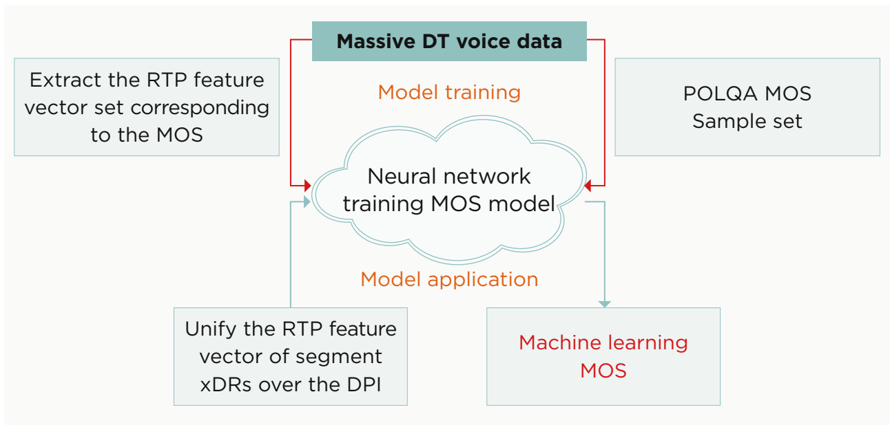
Figure 3-29 MOS model training by using a neural network
