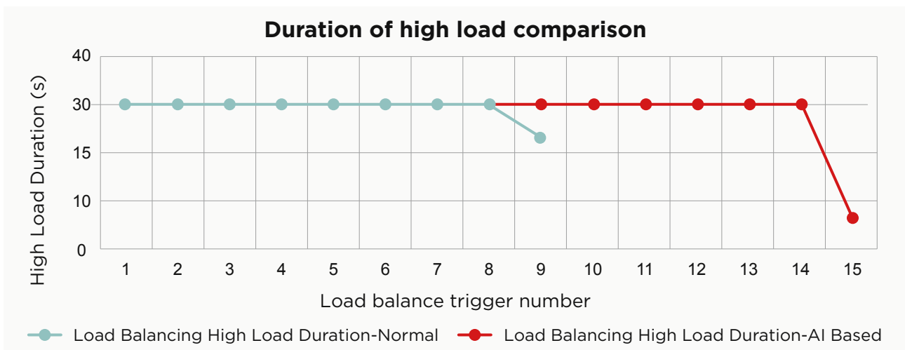
Figure Test Result of Load Balancing - Comparison of Duration of High Load
