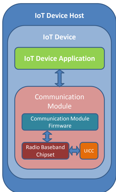
Figure 1 – Generalised IoT Device Architecture
