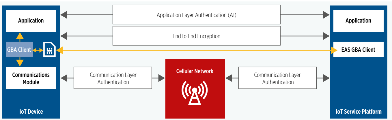
FIGURE 9: IoT SERVICE CONFIGURATION #1 WITH GBA ENHANCEMENT
