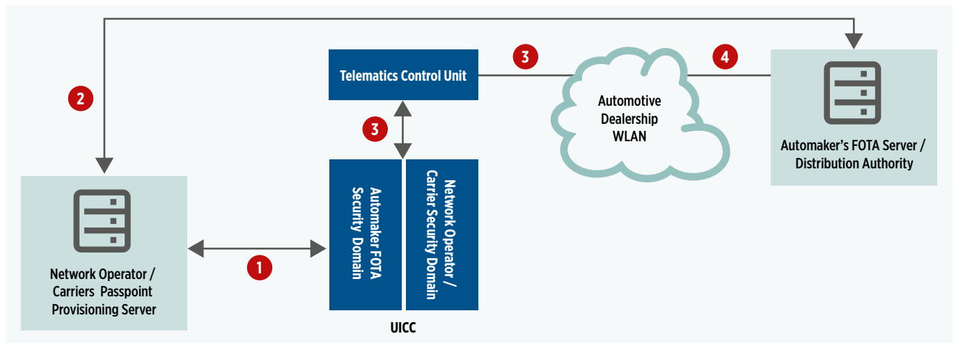
FIGURE 5: PROCESS FLOW FOR WI-FI OFFLOAD USING A SIM CARD IN CONJUNCTION WITH PASSPOINT AND EAP-AKA [28]
