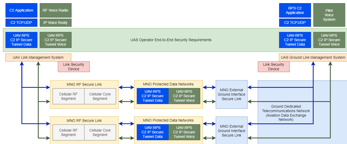
Figure 6. Overall representation of secure infrastructure for multiple tunnels scenario.
