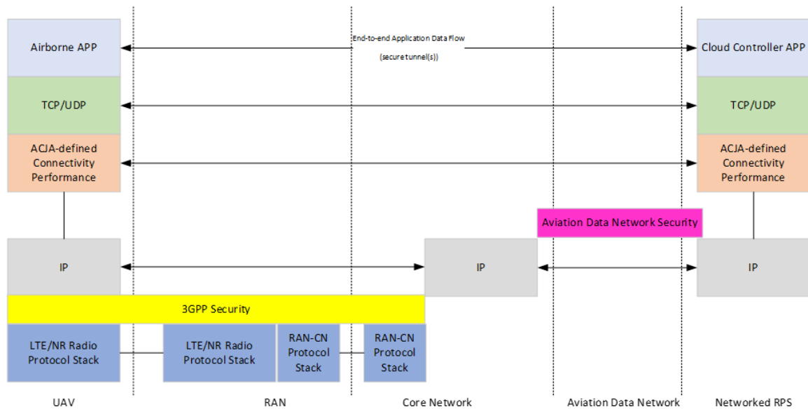
Figure 4. OSI Model Representation for single Air-Ground RF link scenarios.
