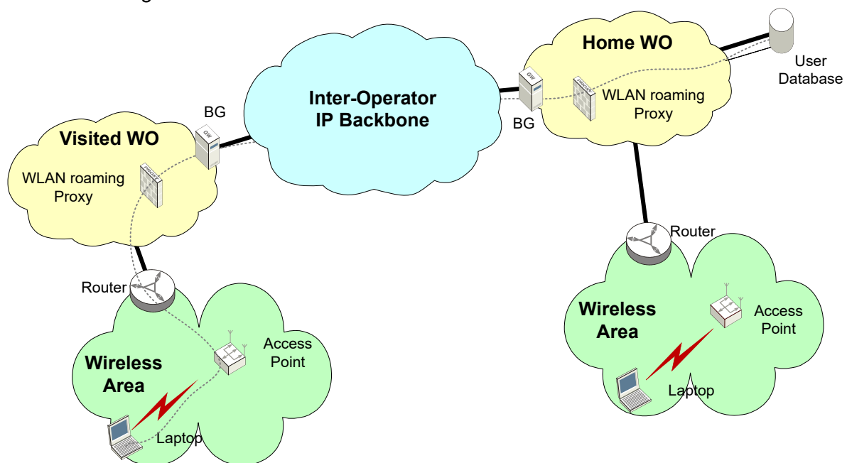
Figure 12: Inter-Service Provider IP Backbone used for the WLAN roaming
