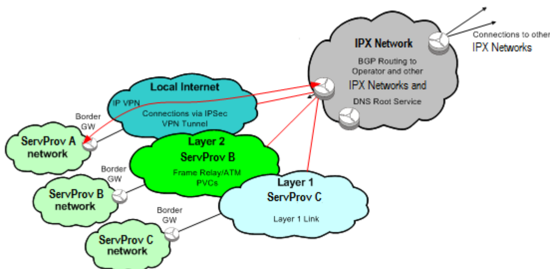
Figure 10: Hub Connectivity Option Scenario
