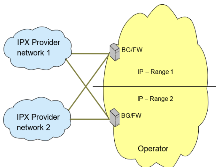
Figure 19: Full-meshed IPX Provider network interconnection
