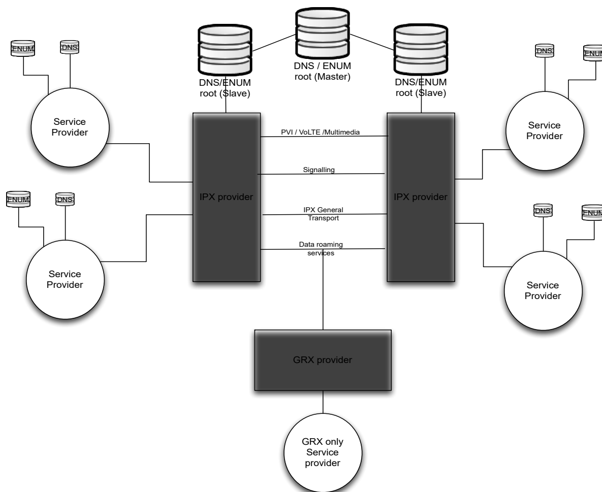
Figure 4: Peering between IPX Provider Networks
