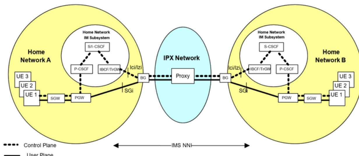
Figure 14: IPX Network used for the IMS Interworking
