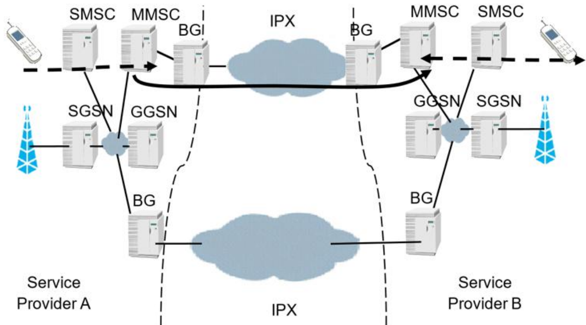
Figure 13: Inter-Service Provider IP Backbone used for MM4
