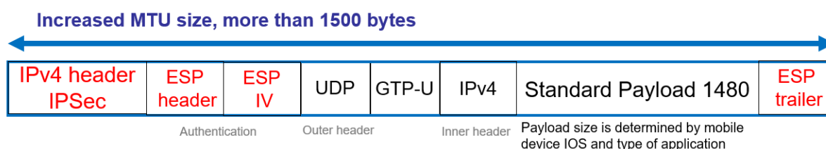
Figure 9: IPv4 packet for GTP with IPSec ESP encryption
