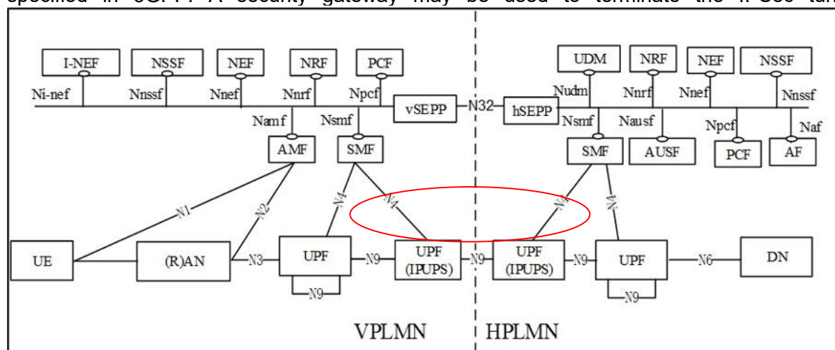
Figure 7: : N9 Interface / Roaming traffic between VPLMN and HPLMN
