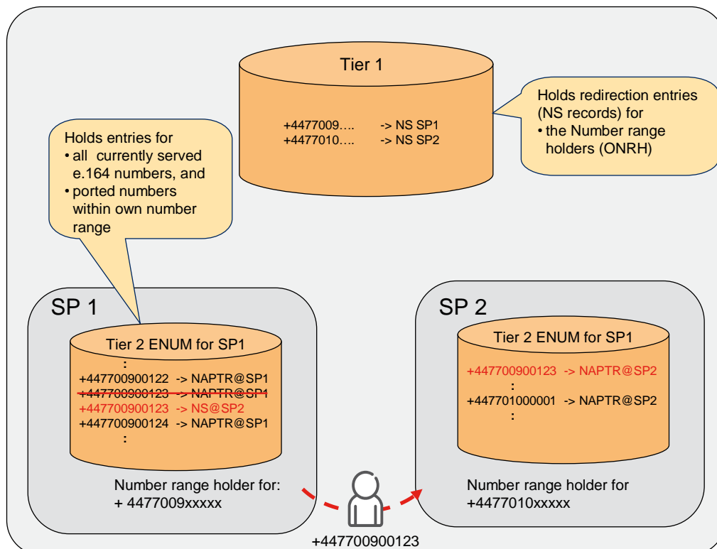
Figure 20: : Redirection at Tier-2
