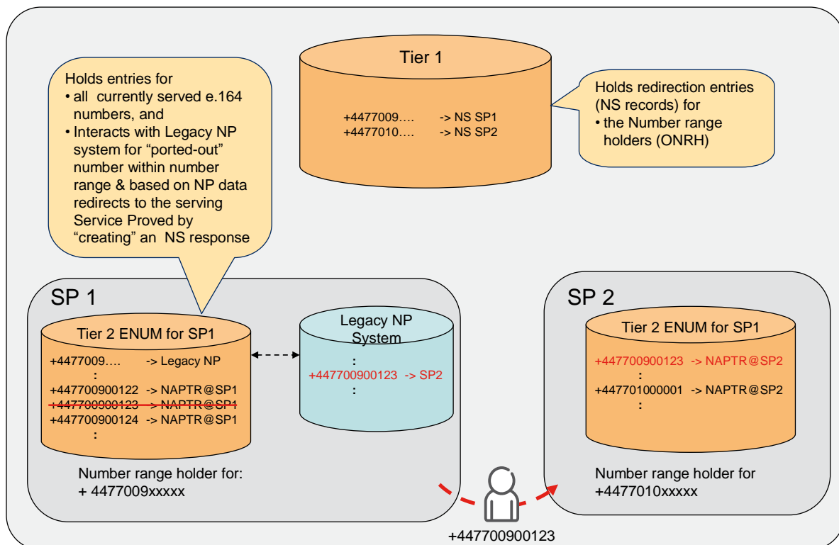
Figure 21: Redirection at Tier-2 based on Legacy NP system interaction
