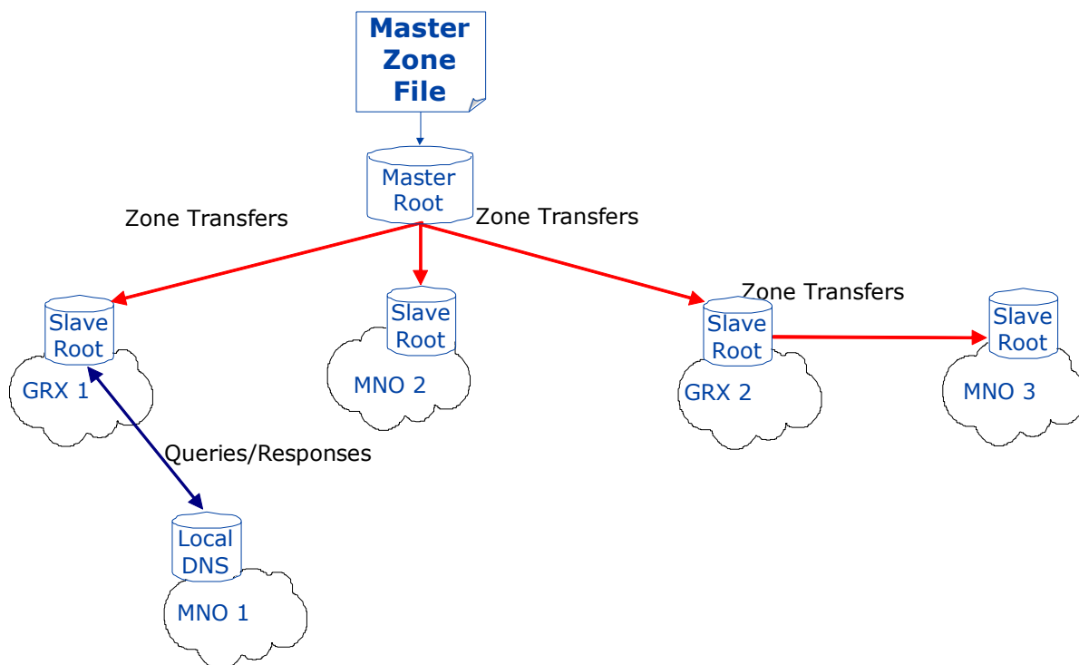
Figure 1: Backbone Architecture
