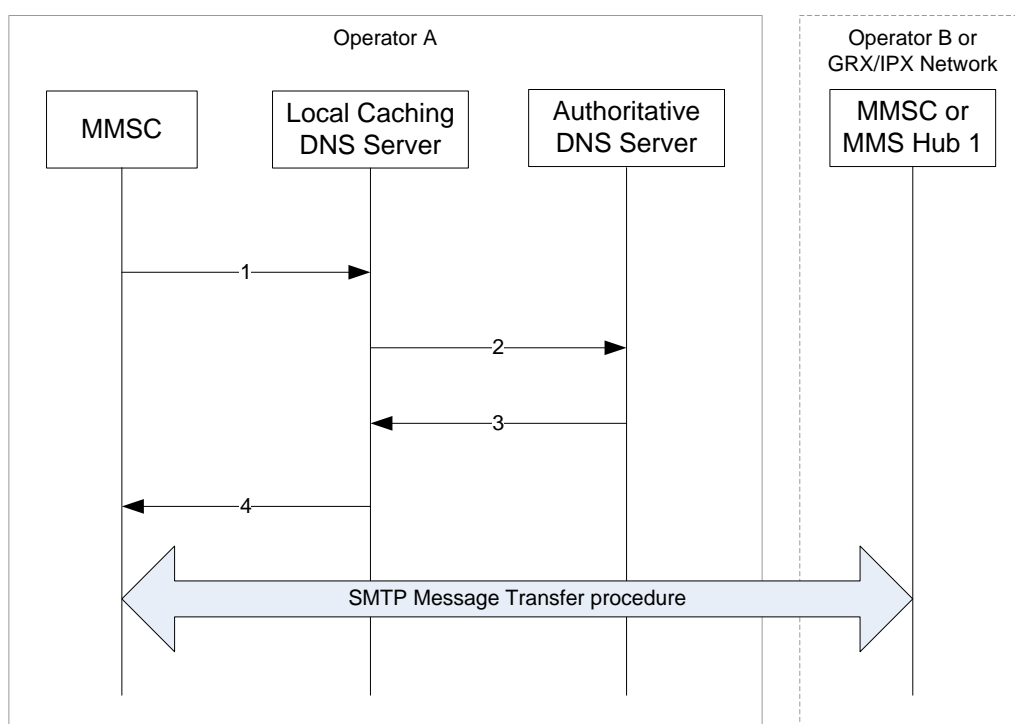
Figure 8: MMS Inter-operator Delivery
