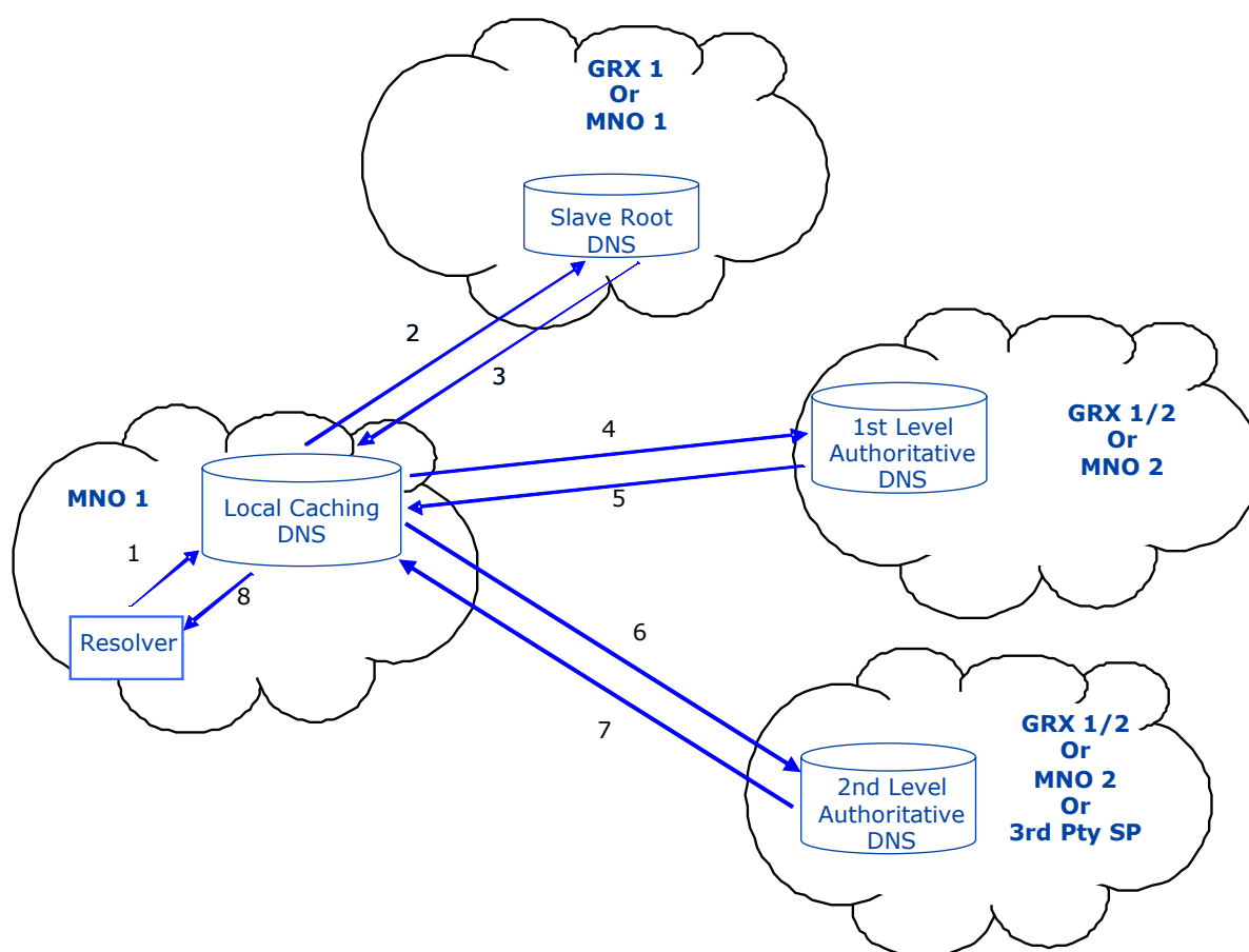
Figure 1a: Resolver Architecture with multiple levels of Authoritative DNS
