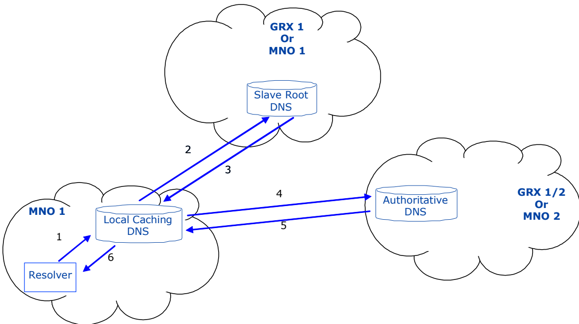
Figure 3: Resolver Architecture
