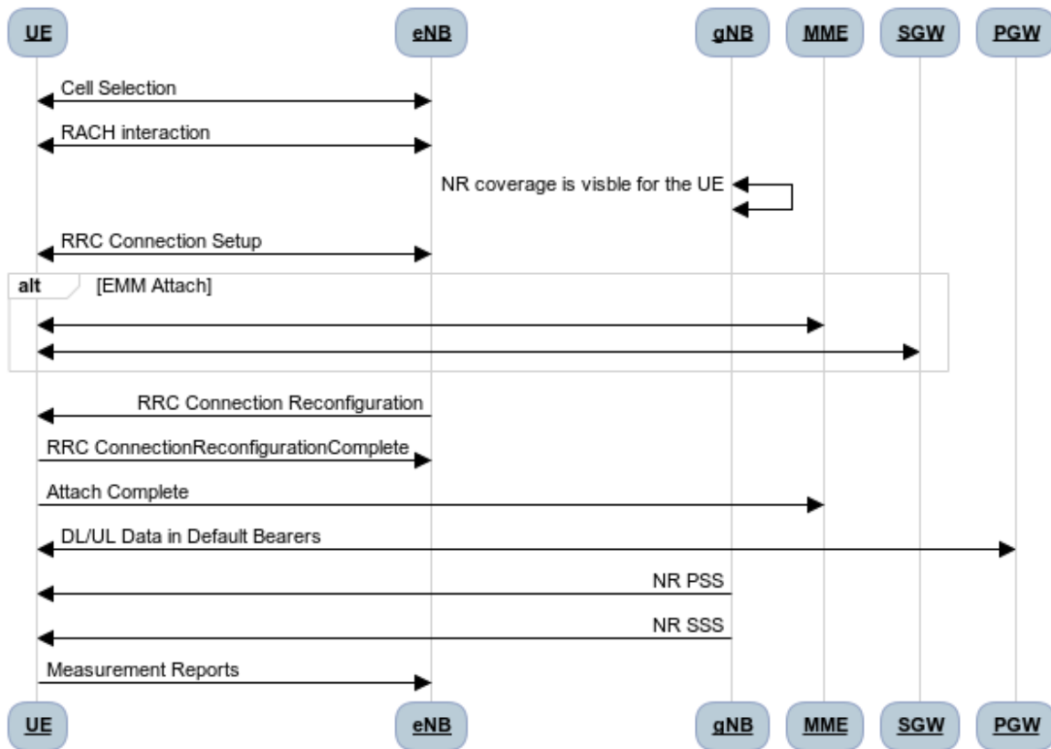
Figure 21 5G NSA ENDC Registration
