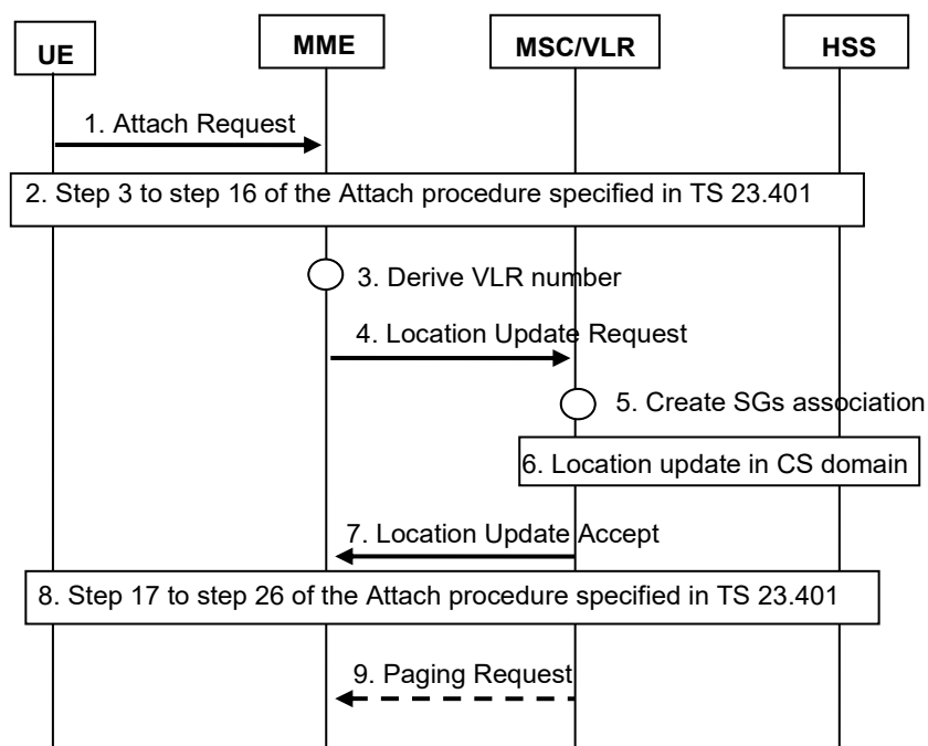
Figure 14: Combined EPS /IMSI attach
