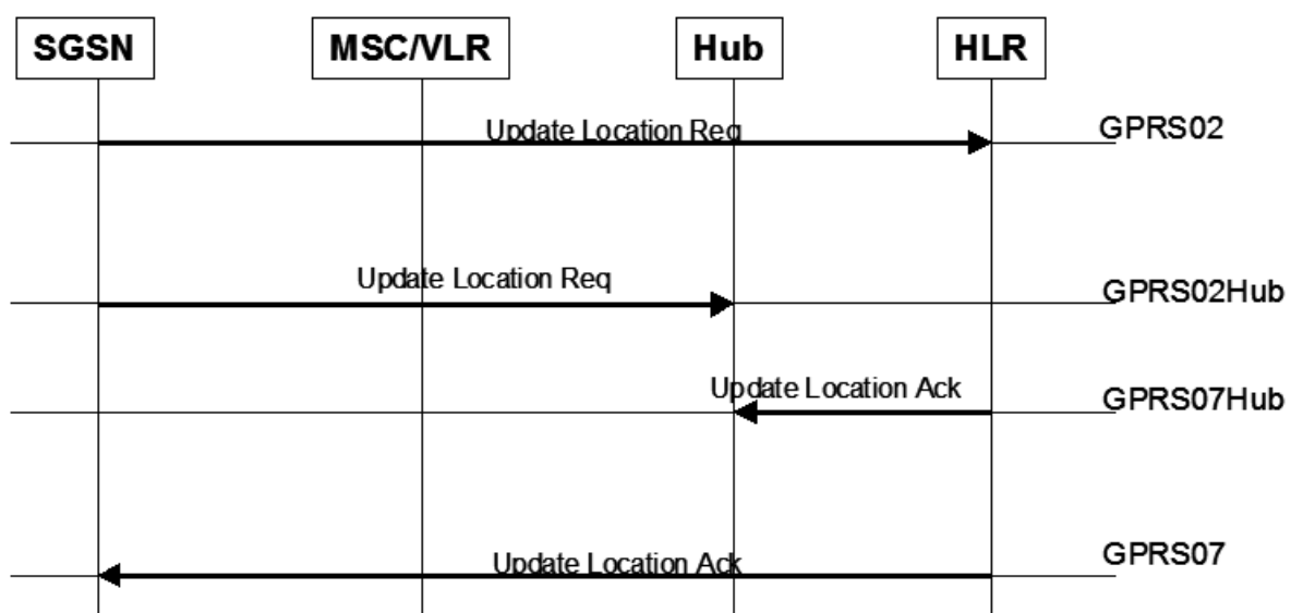
Figure 7: Packet Switch flow for Roaming Hub Provider
