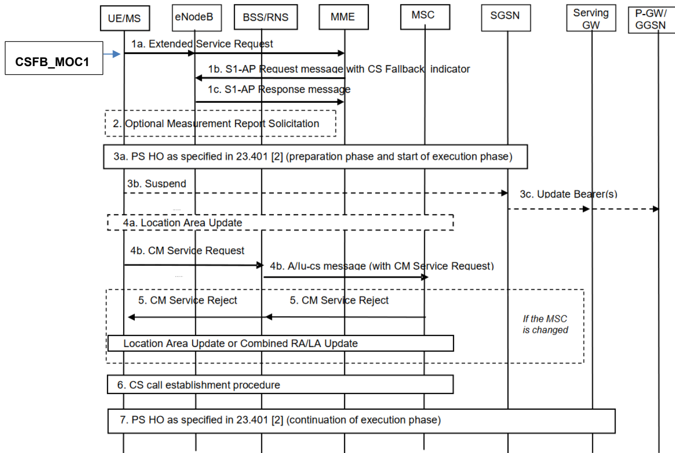
Figure 15: Voice CSFB MO call with PS / CS HO [4]
