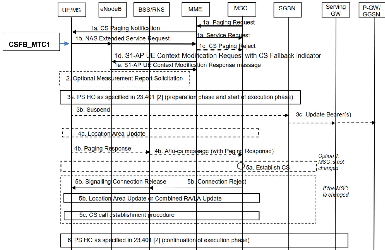
Figure 17: Voice CSFB MT call with PS / CS HO [4]
