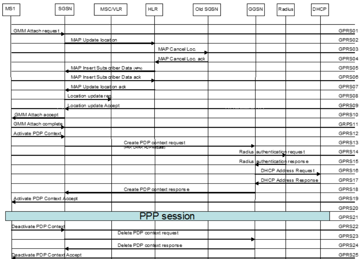
Figure 6: GPRS PDP context and data transfer in bilateral case
