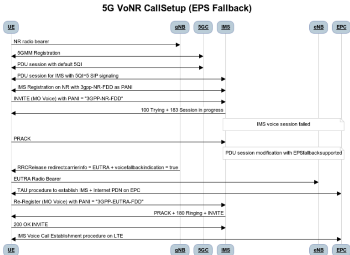
Figure 22 5G VoNR Call Set Up
