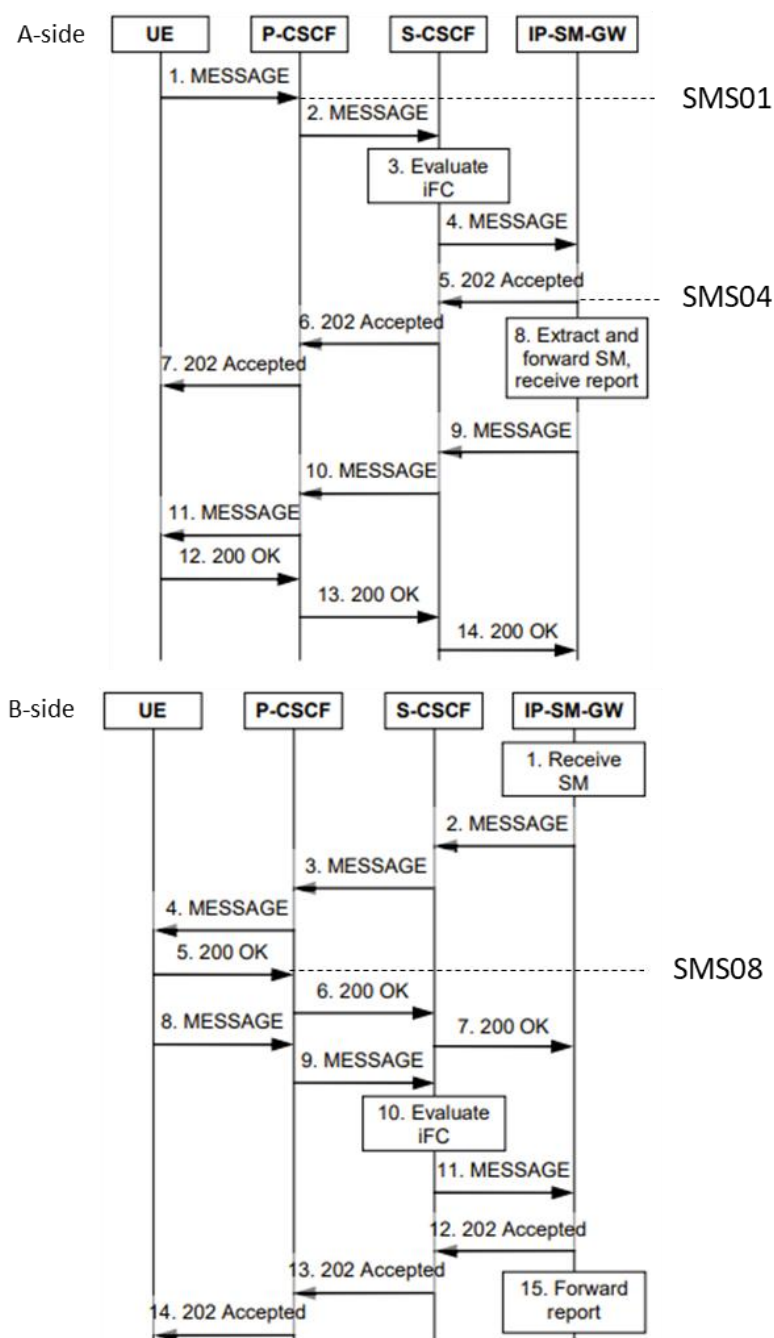
Figure 12: SMS0IP (SIP)
