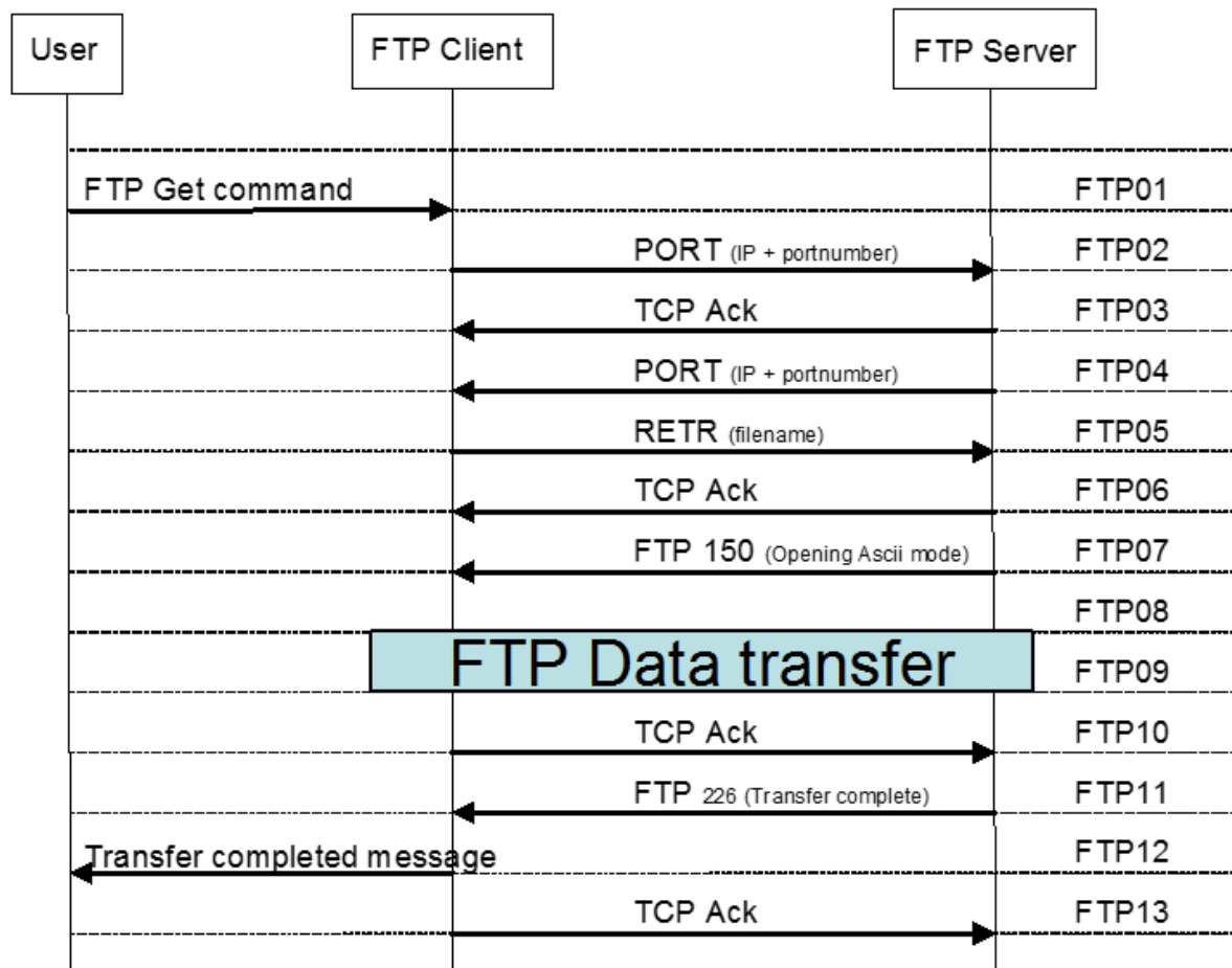
Figure 8: FTP
