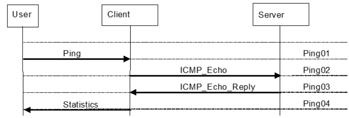
Figure 9: Ping
