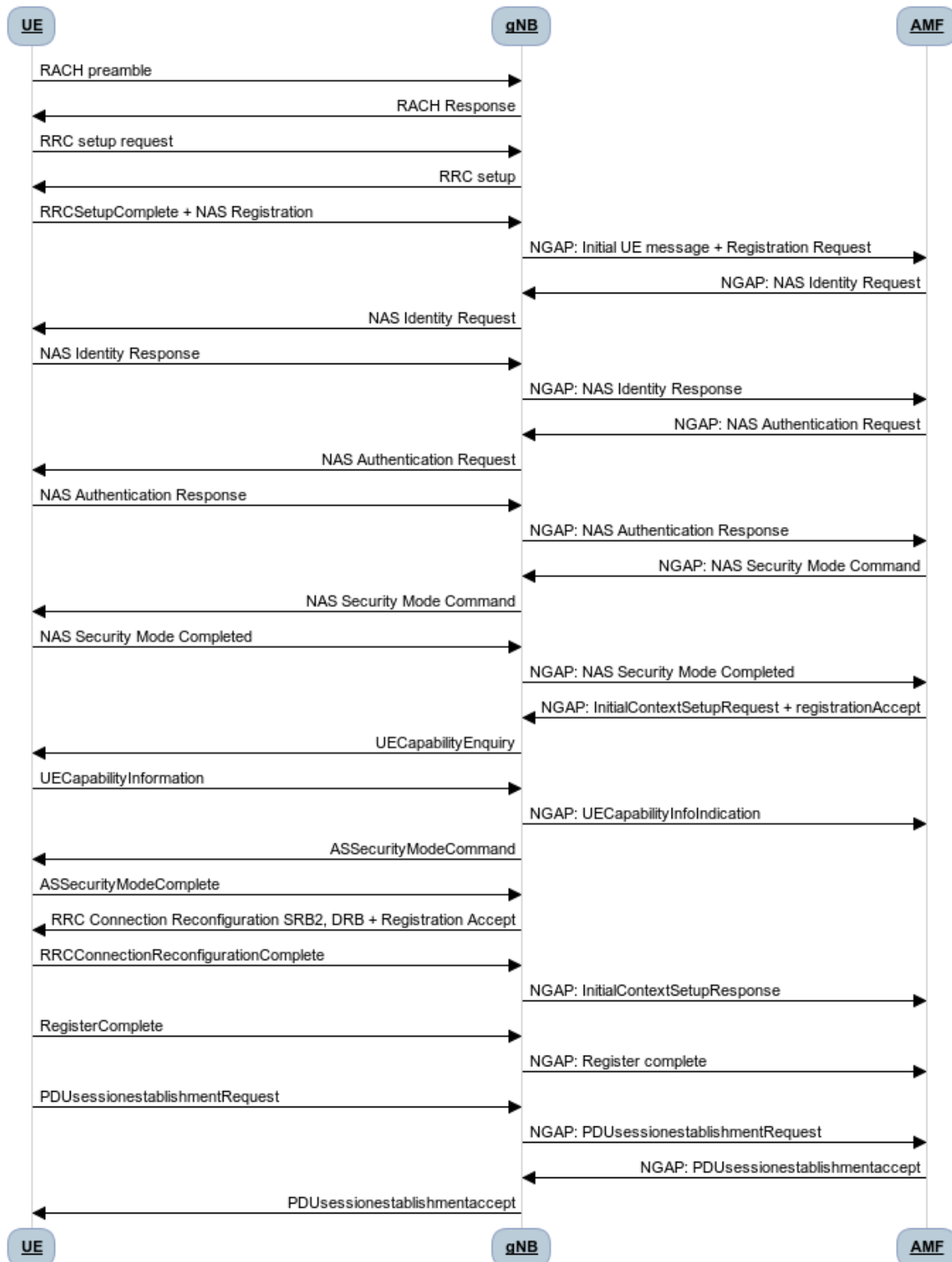
Figure 19 5G Stand Alone Registration
