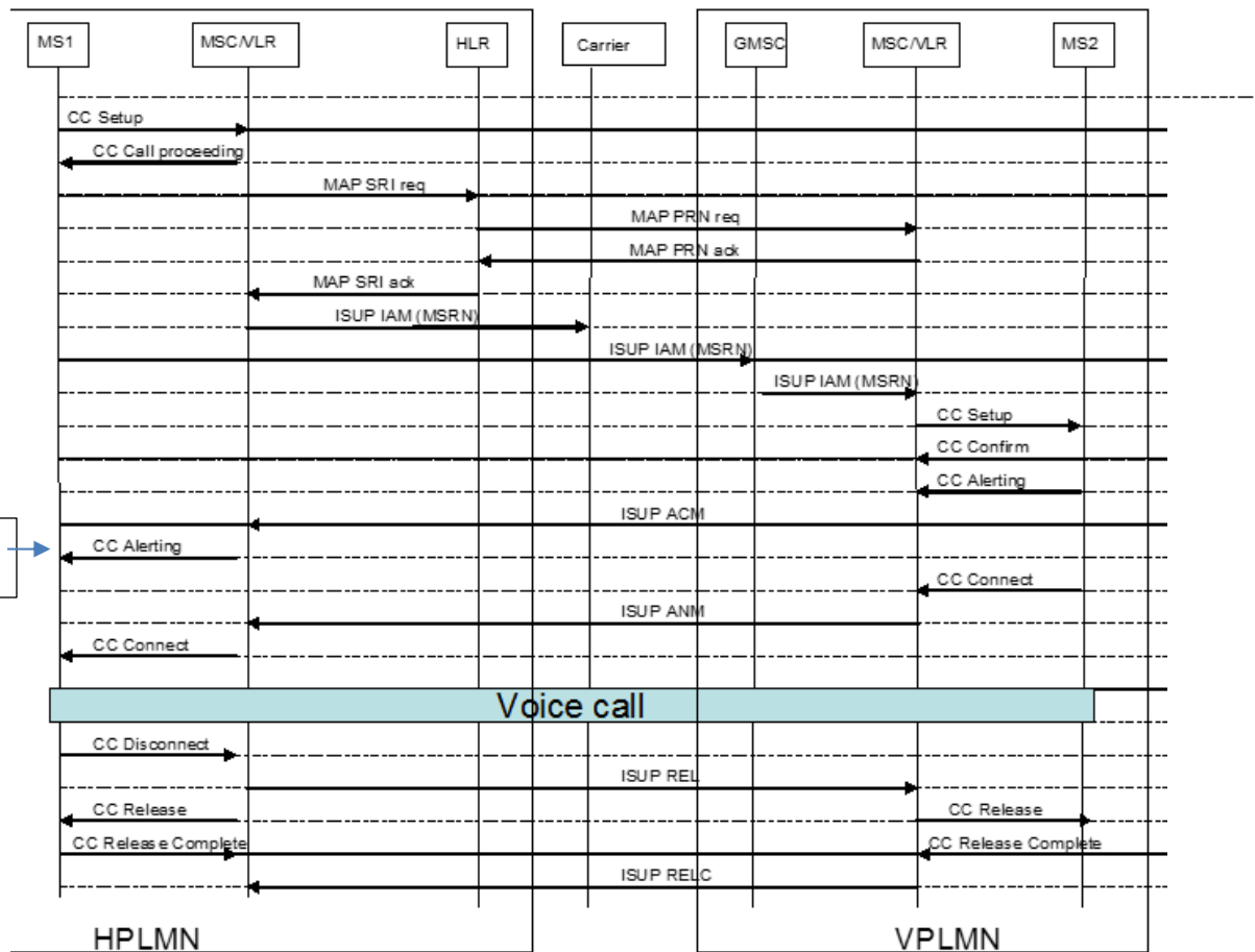
Figure 18: CS MT call establishment
