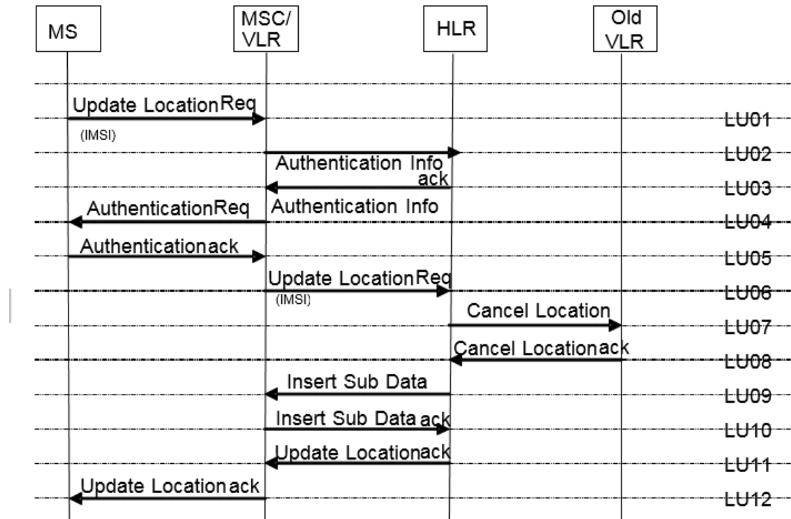
Figure 2: Location update with HLR and VLR
