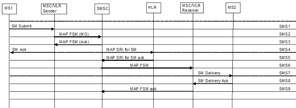
Figure 11: SMS and SMSoSGs
