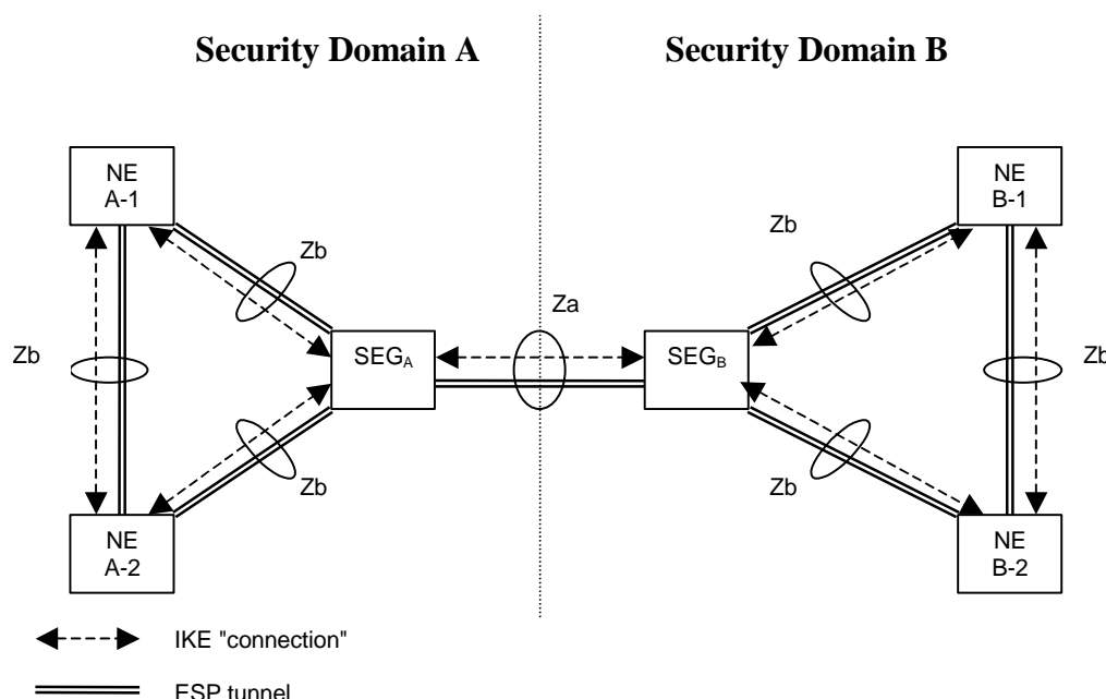
Figure 40: NDS/IP Architecture
