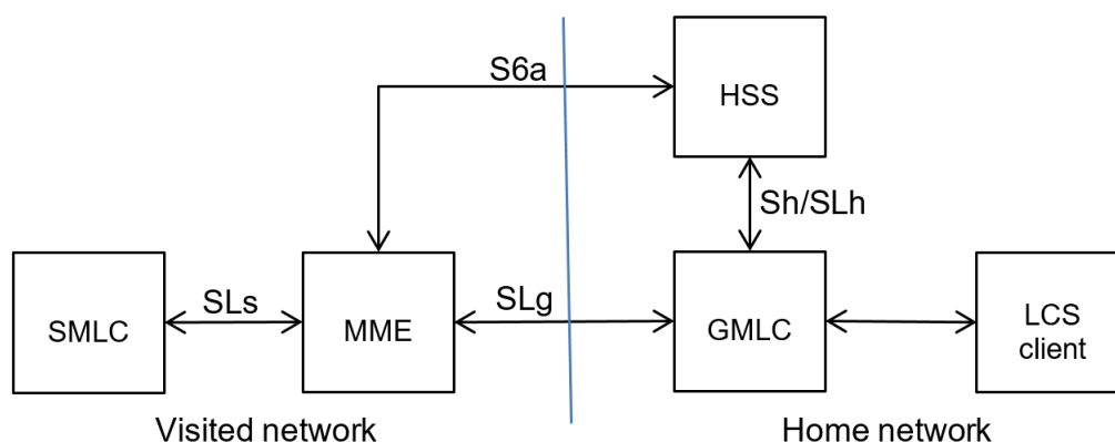
Figure 24GMLC/MME/SMC architecture
