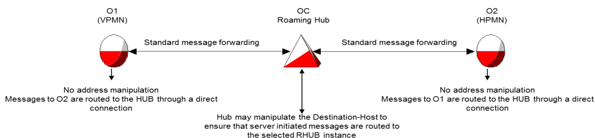
Figure 30: Direct connection
