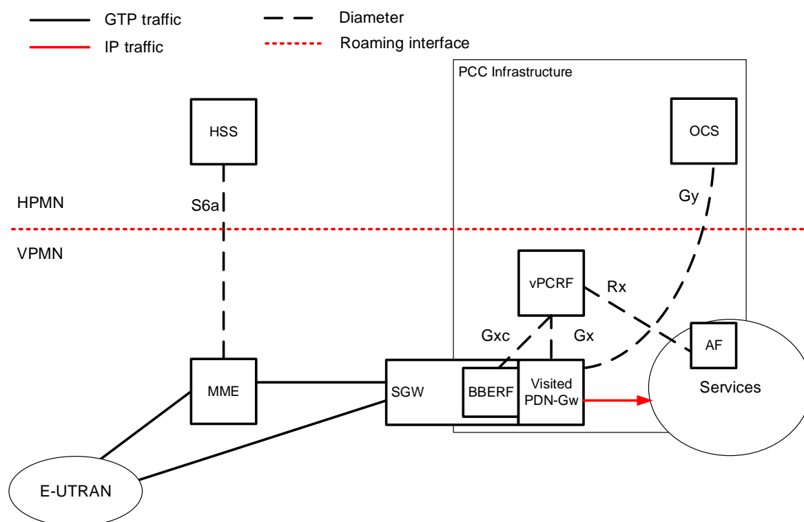
Figure 34: PCC Architecture with Local Break Out architecture
