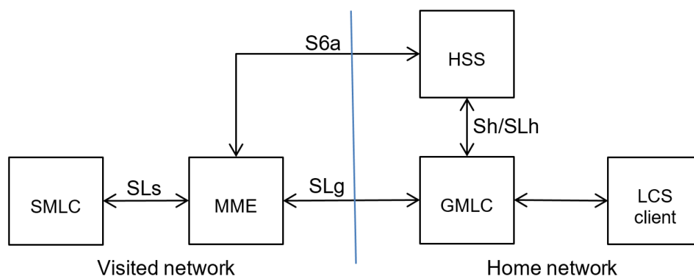
Figure 23 GMLC/MME/SMC architecture
