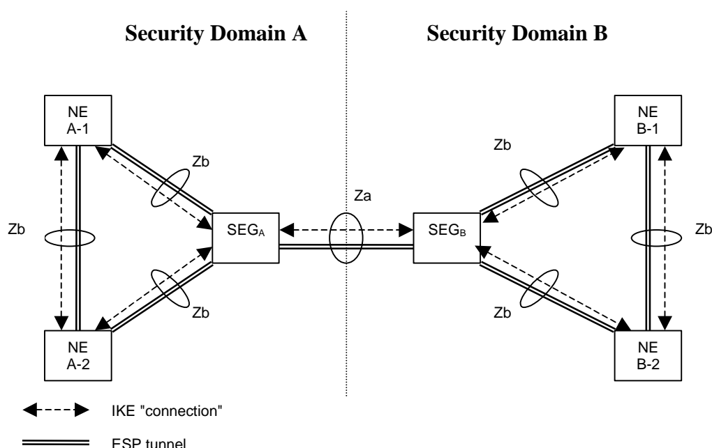
Figure 41: NDS/IP Architecture
