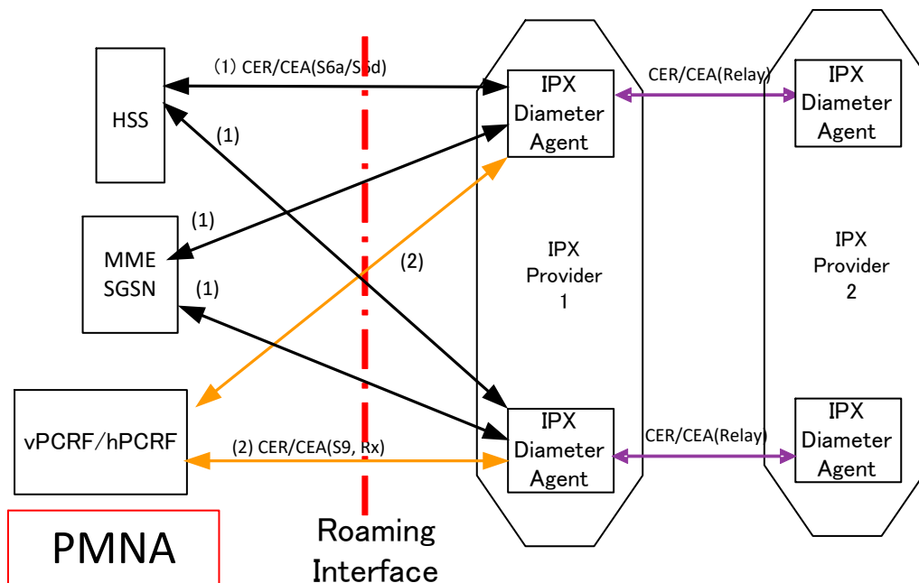
Figure 40: Diameter architecture example 6
