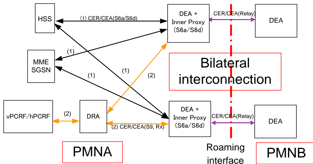
Figure 38: Diameter architecture example 4
