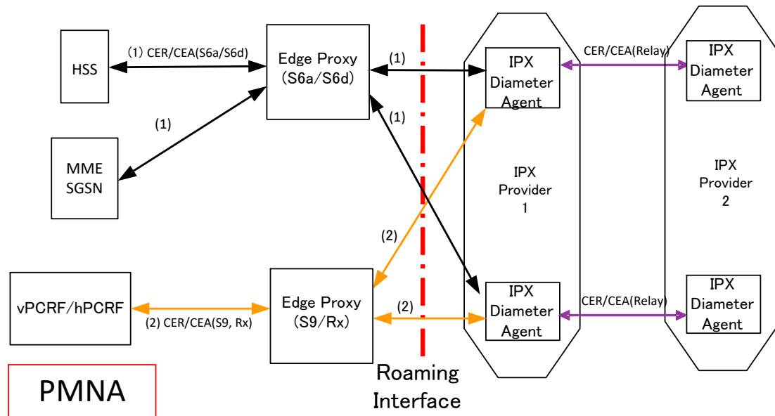
Figure 39: Diameter architecture example 5
