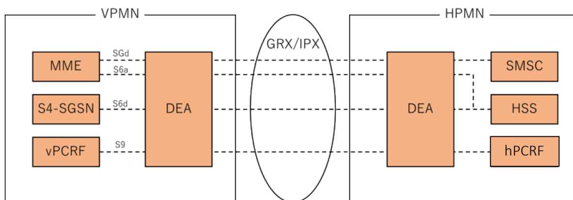
Figure 4: Diameter Roaming Implementation Architecture
