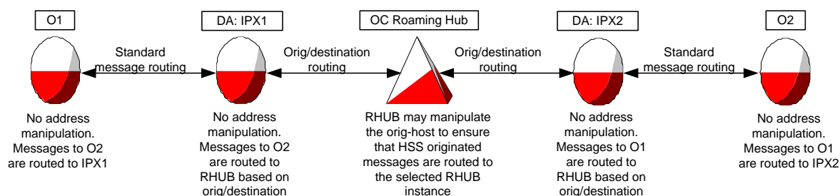
Figure 31: Origin/Destination realm based routing
