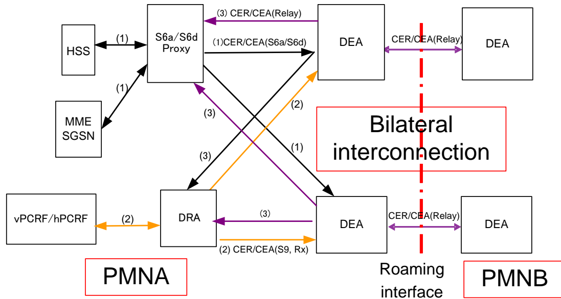
Figure 35: Diameter architecture example 1
