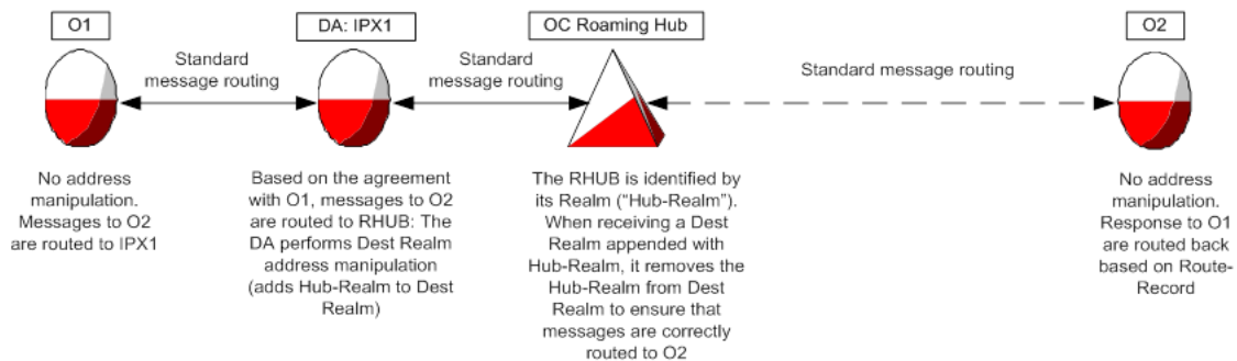
Figure 32: Destination realm modification
