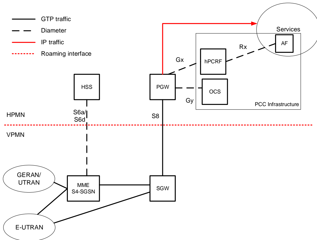
Figure 33: PCC Architecture with Home Routed architecture
