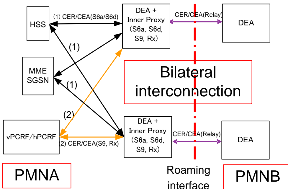
Figure 36: Diameter architecture example 2
