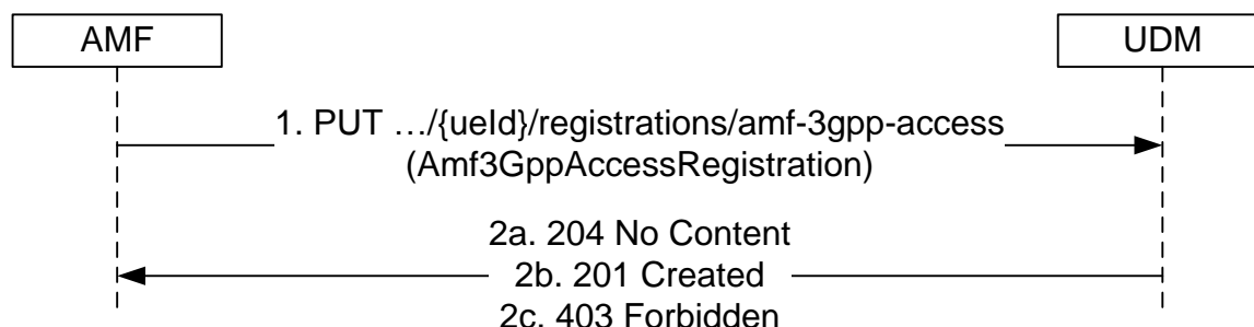
Figure 9 AMF registering for 3GPP access [10] Section 5.3.2.2.2
