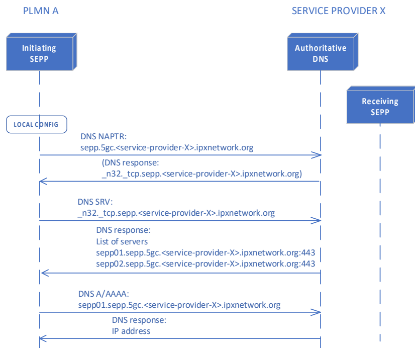
Figure 60 - Dynamic SP SEPP Discovery
