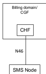
Figure 33 – 5G Reference point Representation (SMS charging)
