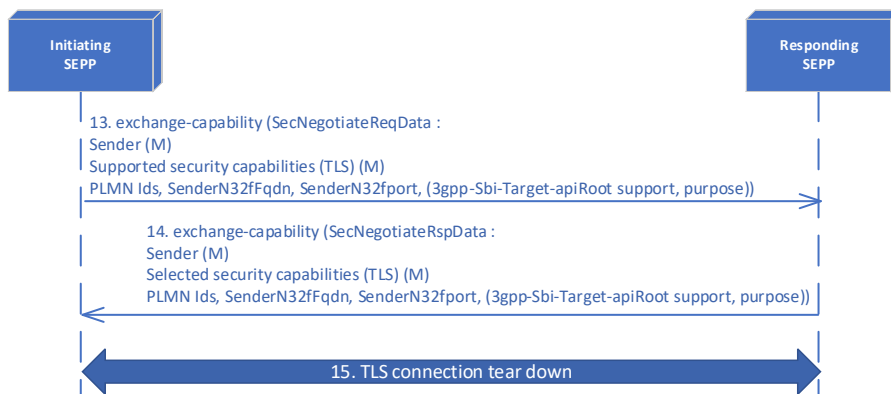
Figure 41 - N32-c Handshake
