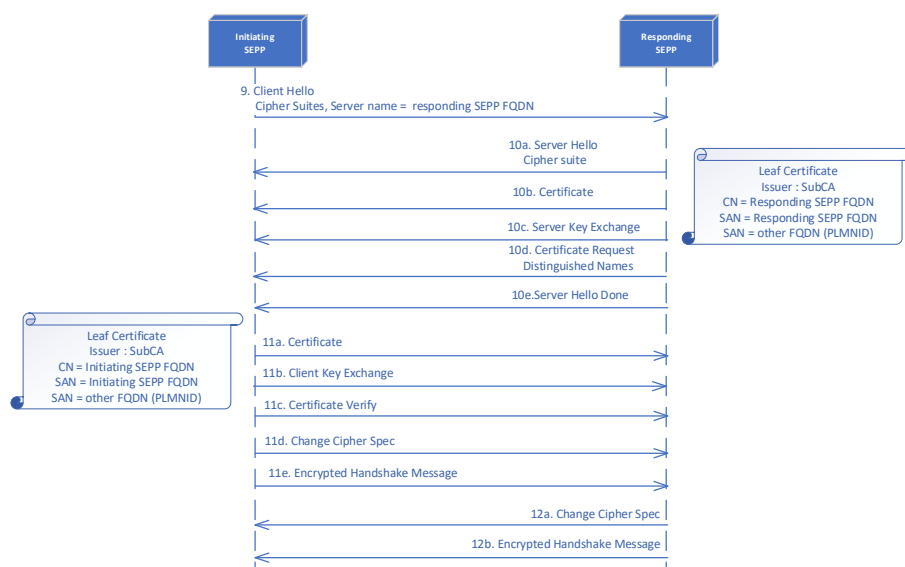
Figure 40 - TLS Handshake
