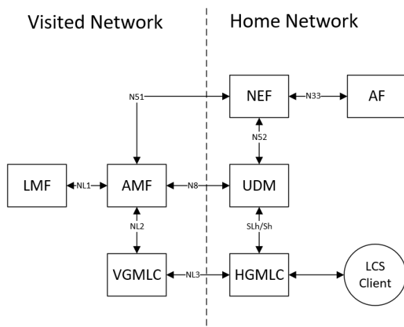
Figure 28 – Location Support
