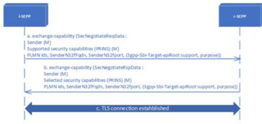
Figure 53 - N32-c Handshake
