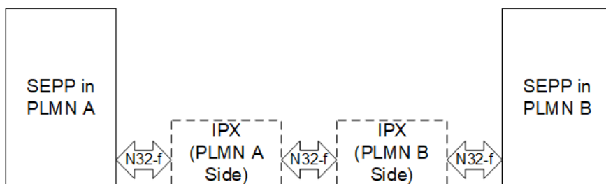
Figure 10 – N32-f Interface with PRINS (ALS)
