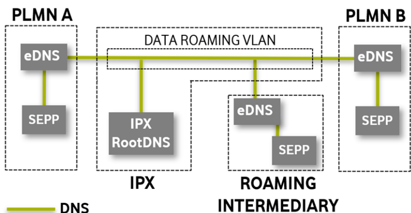
Figure 24– Data roaming VLAN overview.
