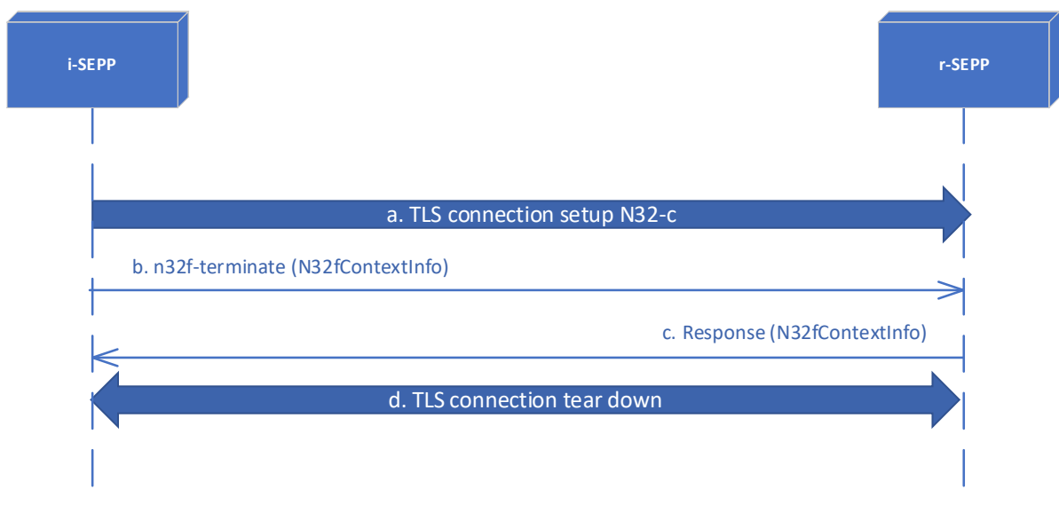
Figure 56 - N32-f Context Termination
