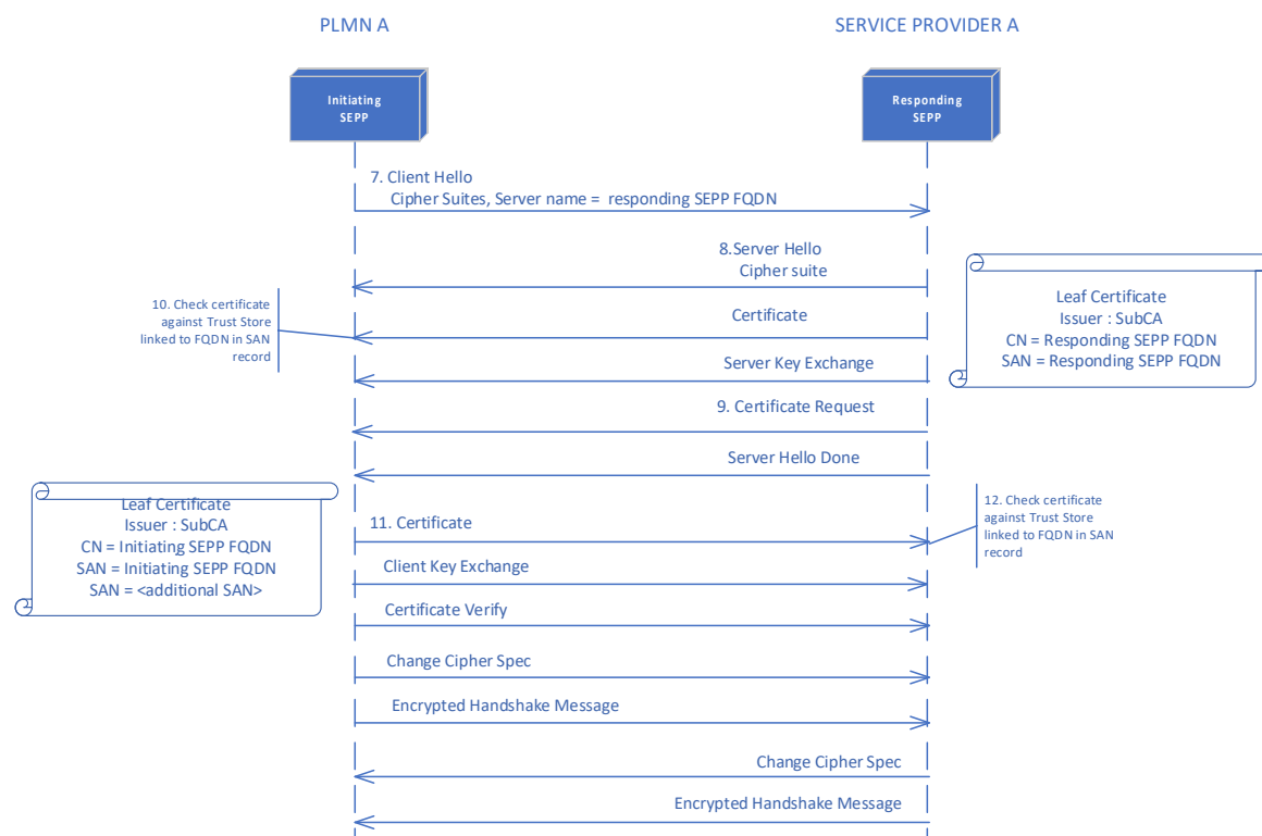
Figure 45 - TLS Handshake
