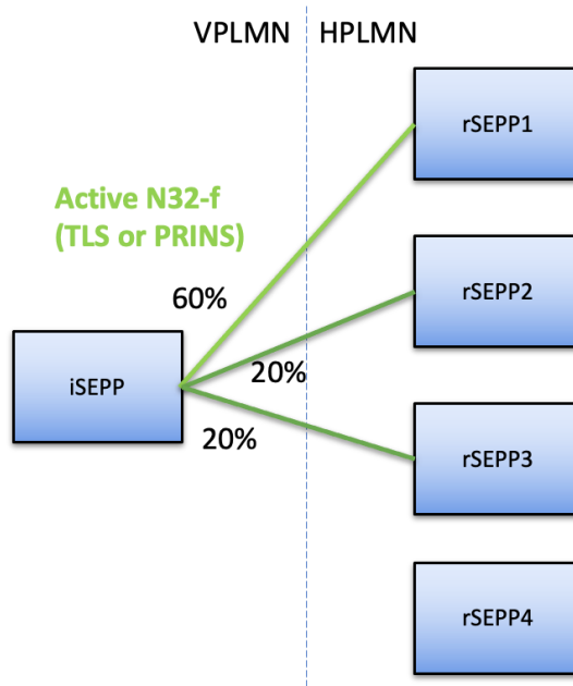
Figure 26 – Sample load distribution over rSEPPs
