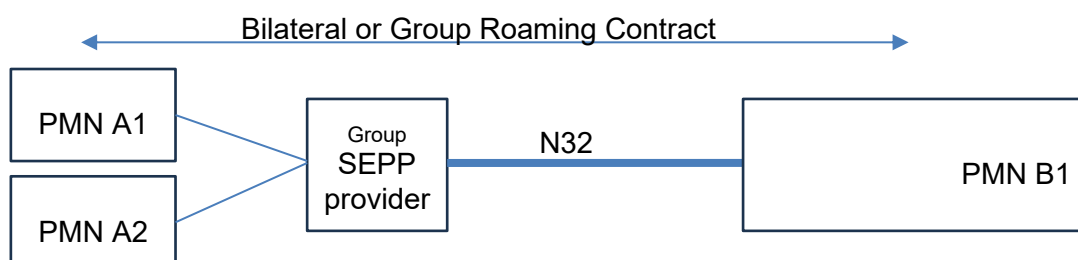
Figure 17 - Bilateral scenario between Mobile Operator Groups
