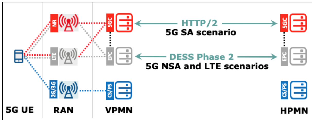
Figure 13 – Confidentiality Protected Roaming Scenarios
