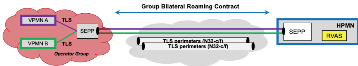
Figure 18 – Bilateral scenario between Mobile Operator Groups with a shared SEPP
