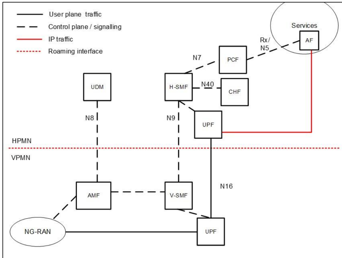
Figure 15 – PCC Architecture with Home Routed Architecture
