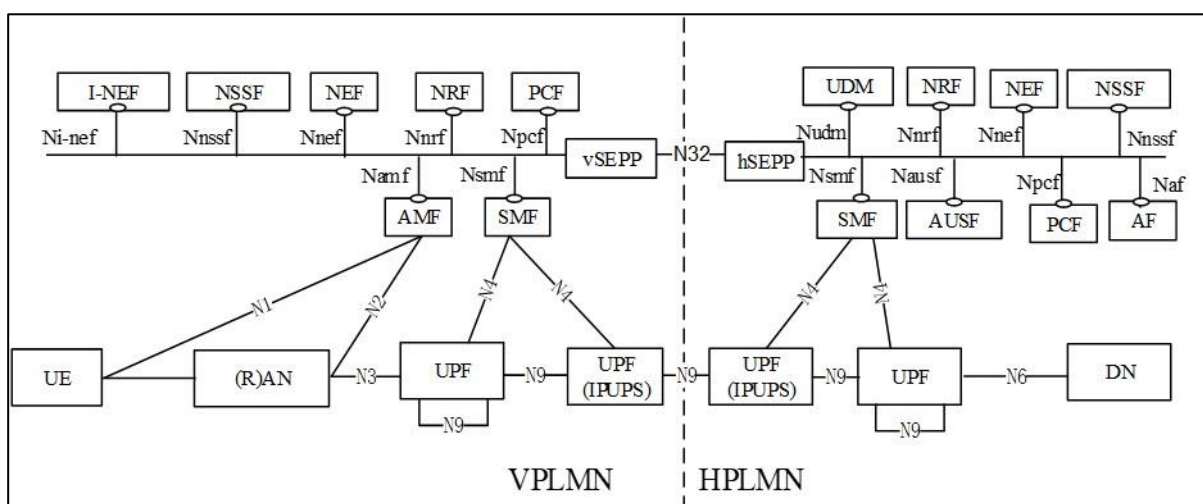
Figure 13 – Roaming Home Routing Scenario – In Serviced Based Interface Presentation
