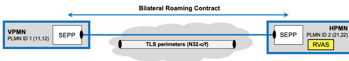
Figure 16– Bilateral scenario between VPMN and HPMN with internal SEPPs
