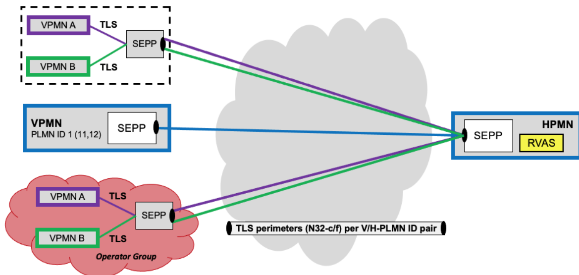
Figure 19 – Combined bilateral inter-PMN connection scenarios
