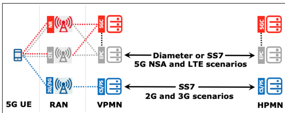
Figure 14 – Least Protected Roaming Traffic Scenarios
