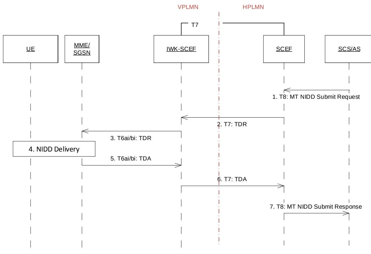
Figure 8: MIoT Mobile Terminated NIDD Procedure for roaming MIoT Device
