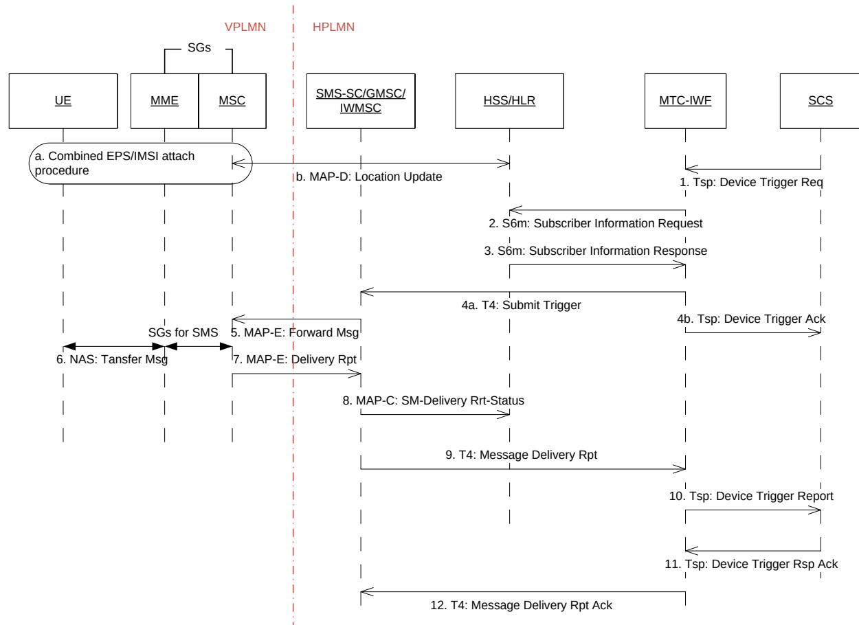
Figure 5: MIoT delivery using T4 trigger over MAP-E.
