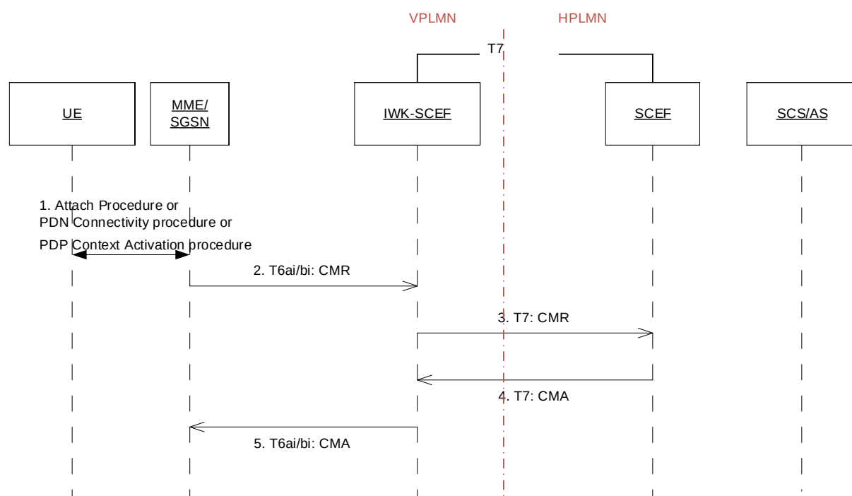
Figure 7: MlIoT T6a/T6b Connection Establishment Procedure for roaming MlIoT Device
