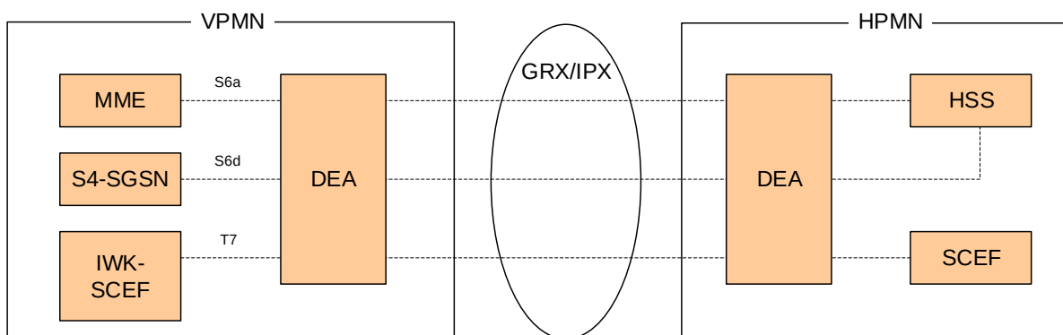
Figure 2: Diameter Roaming Implementation Architecture to support MIoT Roaming
