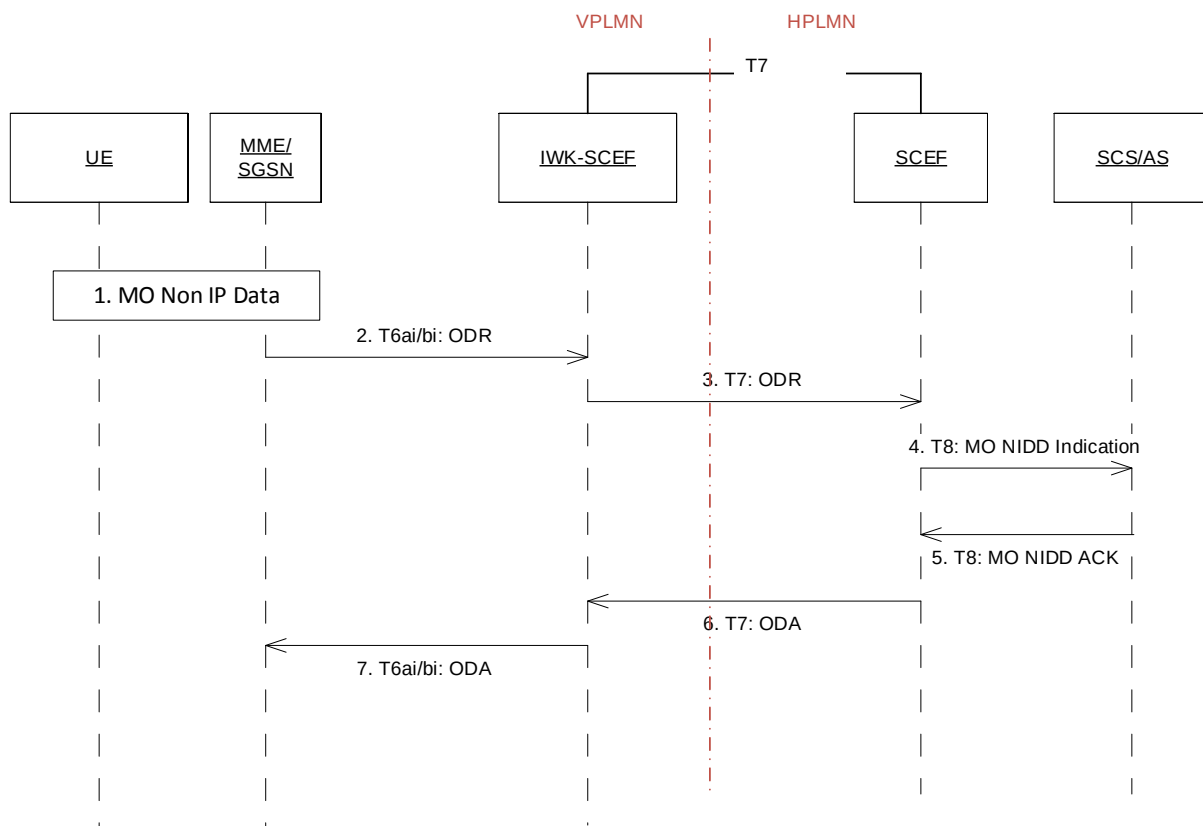
Figure 9: MIoT Mobile Originated NIDD Procedure for roaming MIoT Device
