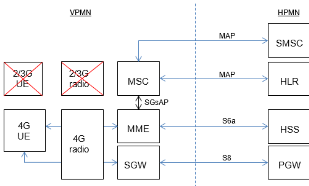
Figure 5: Partial removal of 2/3G
