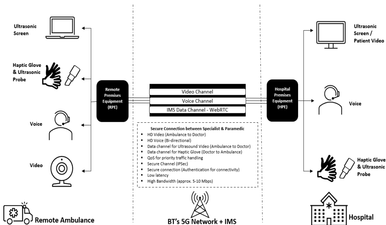
Figure Error! No text of specified style in document.-3 : Setup showing connected ambulance with remote ultrasound scanning using IMS data channel.
