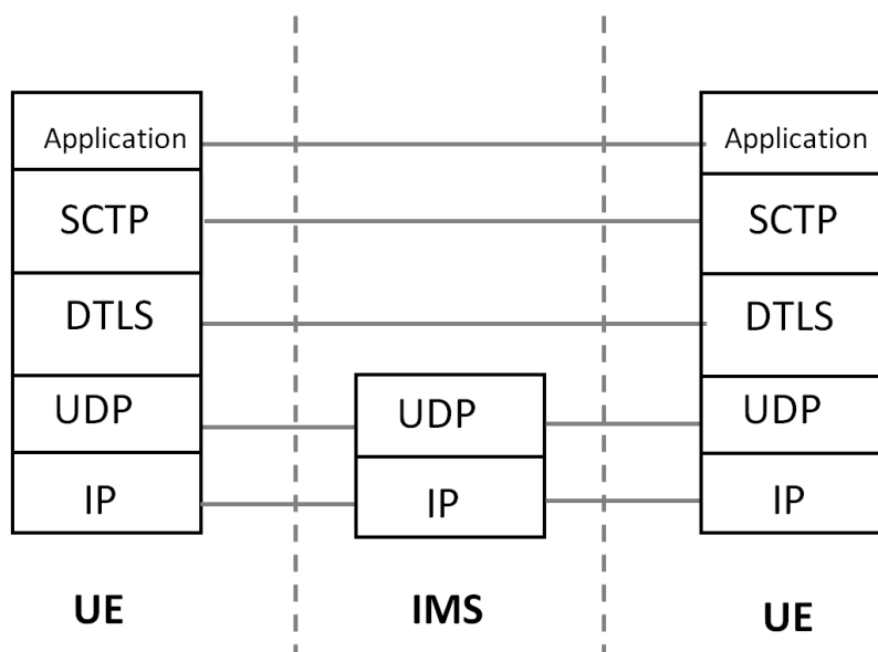
Figure A.1-6: End-to-end UNI-UNI (Mb) and UNI-NNI (lzi) user plane
