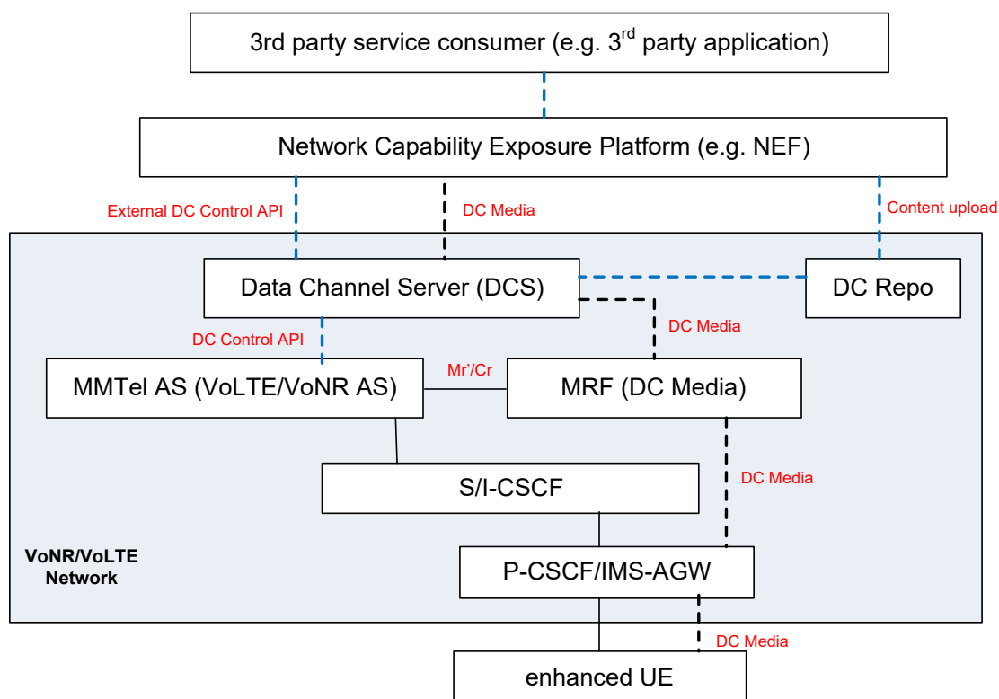
Figure Error! No text of specified style in document.-2: The DC control API and its relationship with other network entities.
