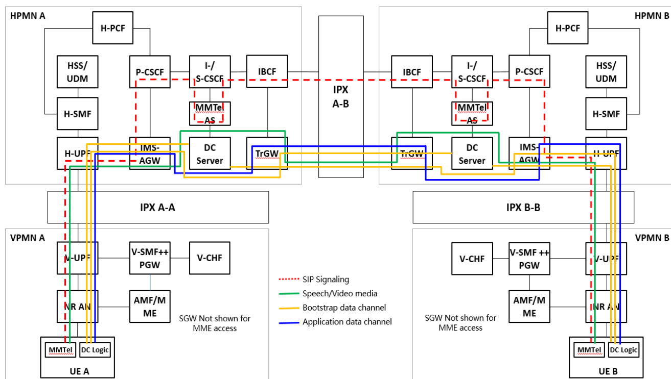
Figure Error! No text of specified style in document.-1: IMS data channel roaming architecture using S8HR/N9HR
