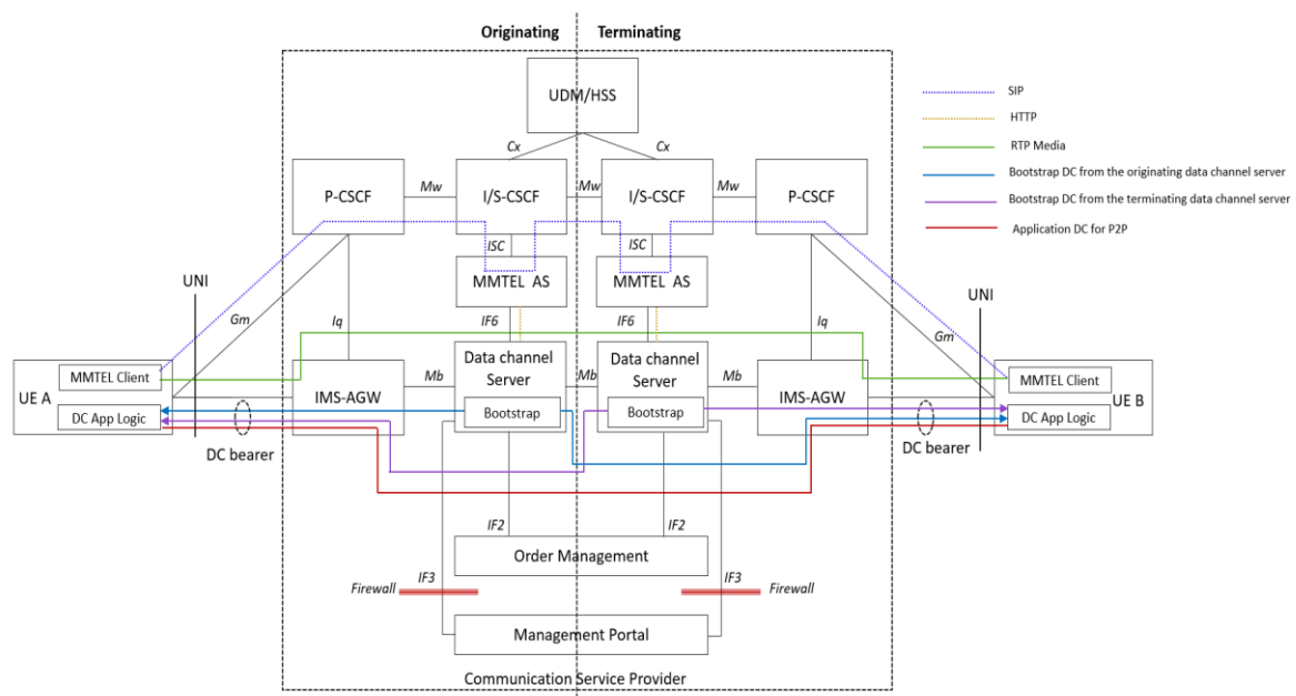
Figure A.2.2.1-1: P2P data channel architecture
