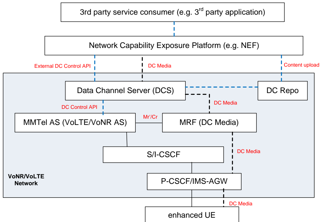
Figure Error! No text of specified style in document.-2: The DC control API and its relationship to other network entities
