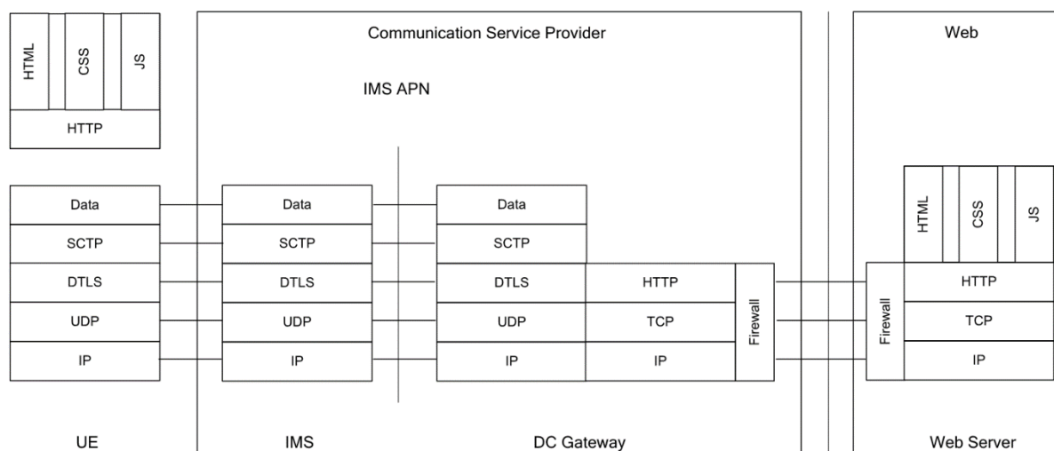
Figure A.1-5: A2P/P2A UNI-NNI user plane
