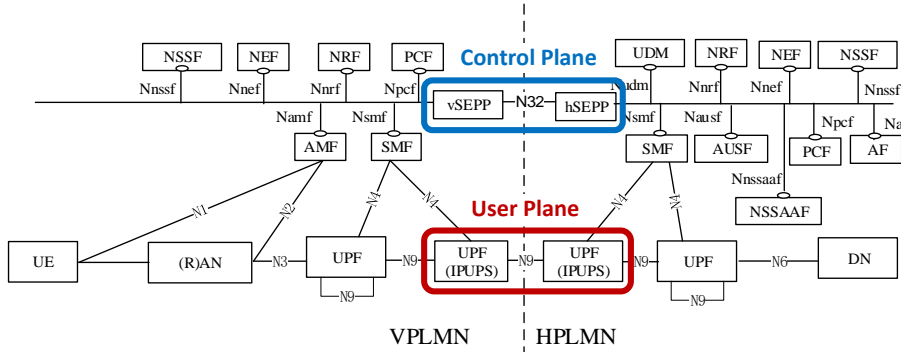
– Roaming 5G System Architecture
