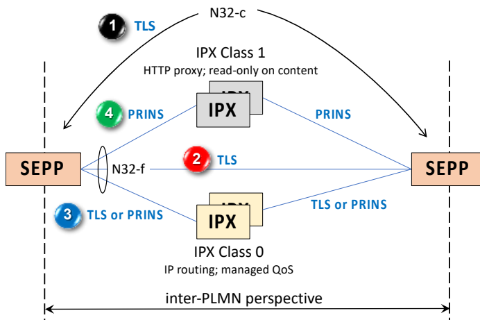
– SEPP using separate N32-connection for connected PLMNs
