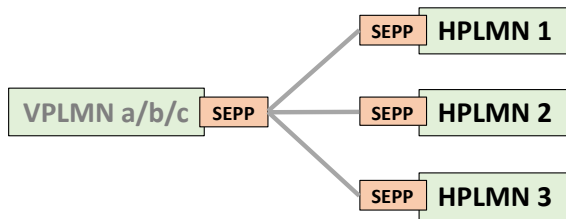
– SEPP using same N32-connection for all VPLMN's PLMN IDs
