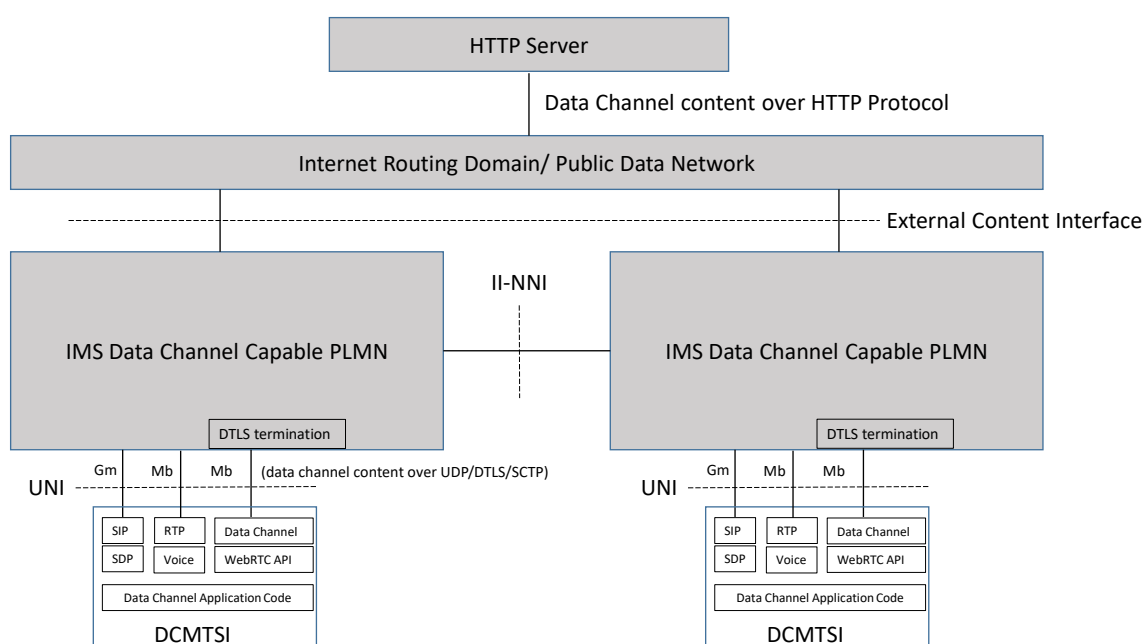
Figure C.1-1: Model A – IMS data channel access to external HTTP Server
