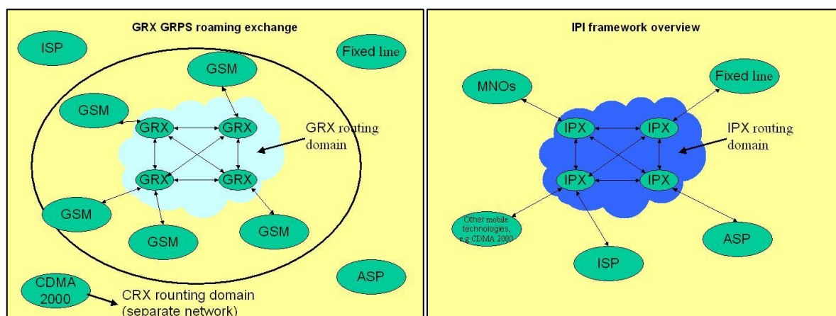
Figure 2: The Evolution of the GRX Model to the IPI Framework
