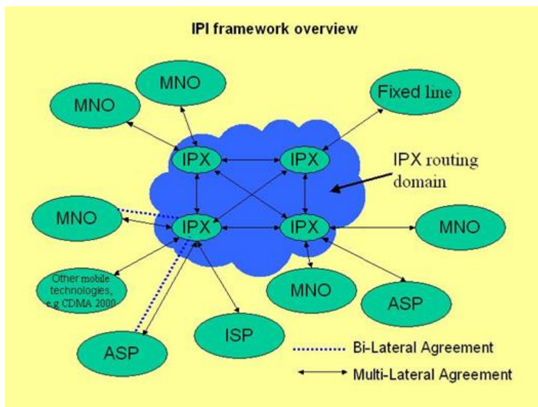
Figure 3: IPI Framework business entities
