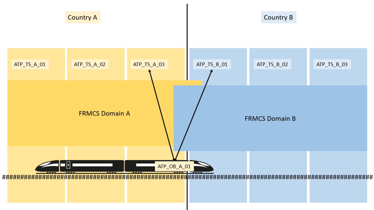
Figure 4: Service Flow
