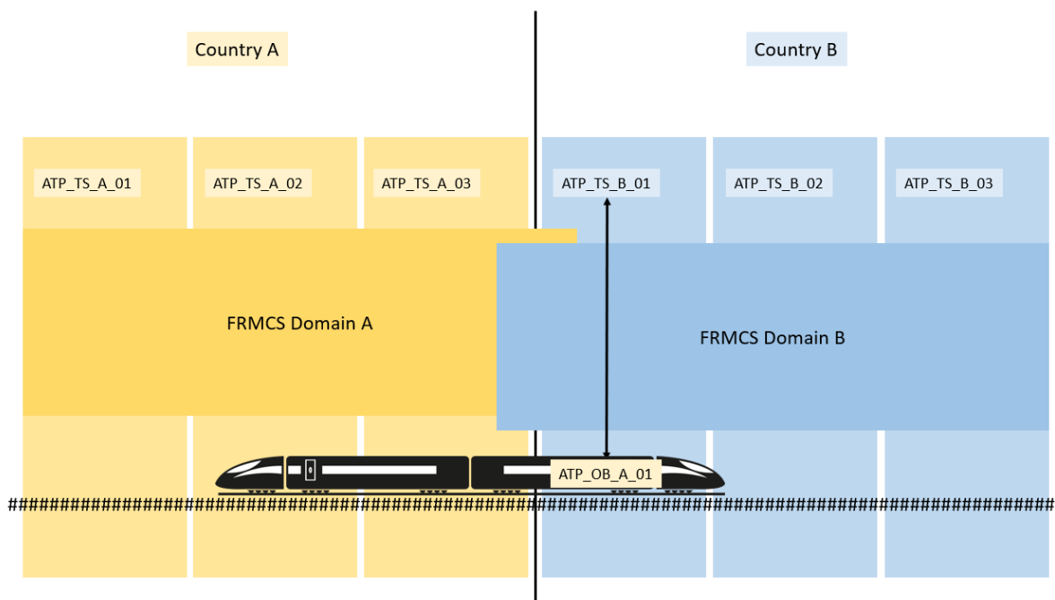
Figure 5: Post conditions
