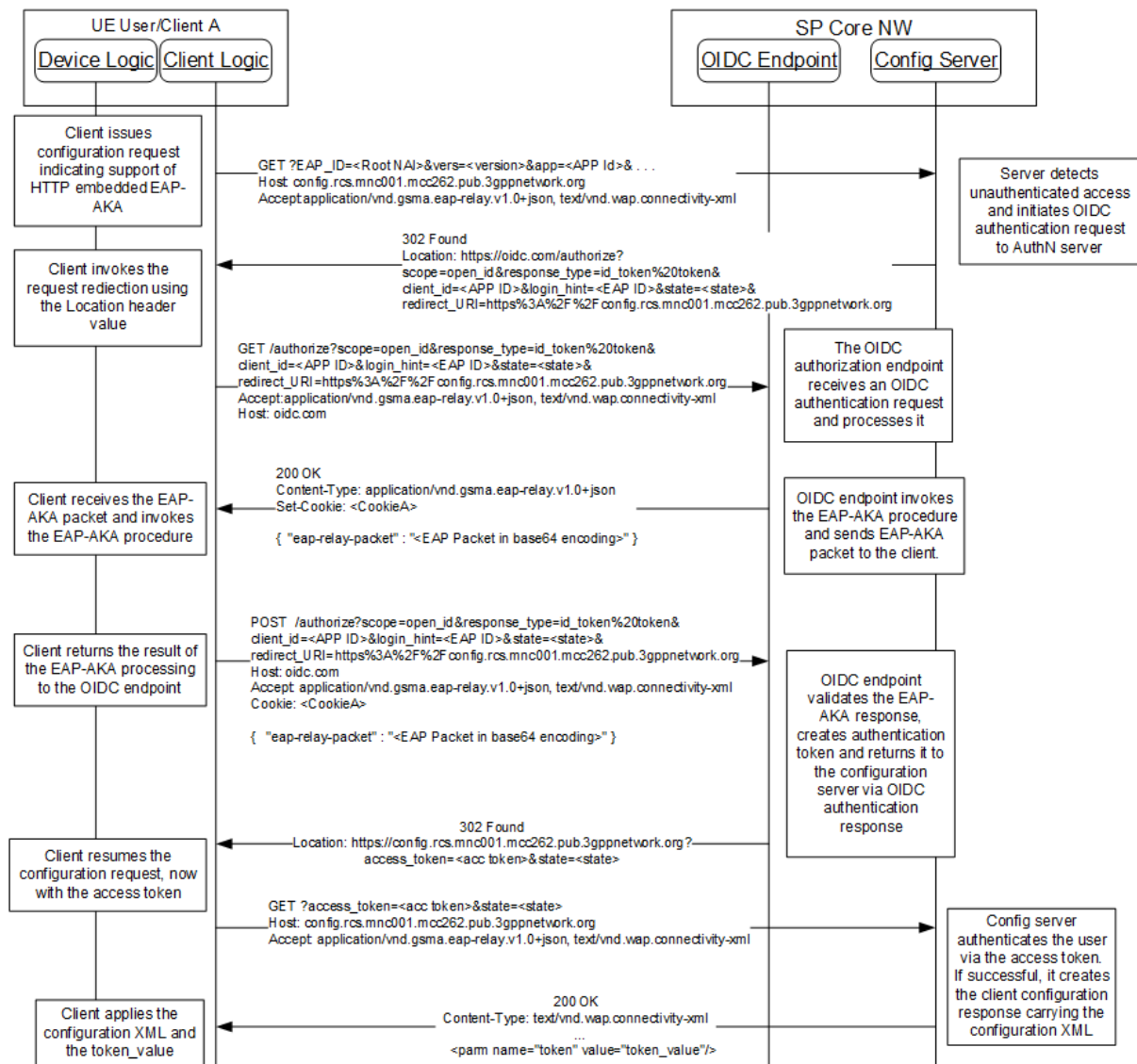
Figure 10: Authentication Flow using HTTP embedded EAP-AKA
