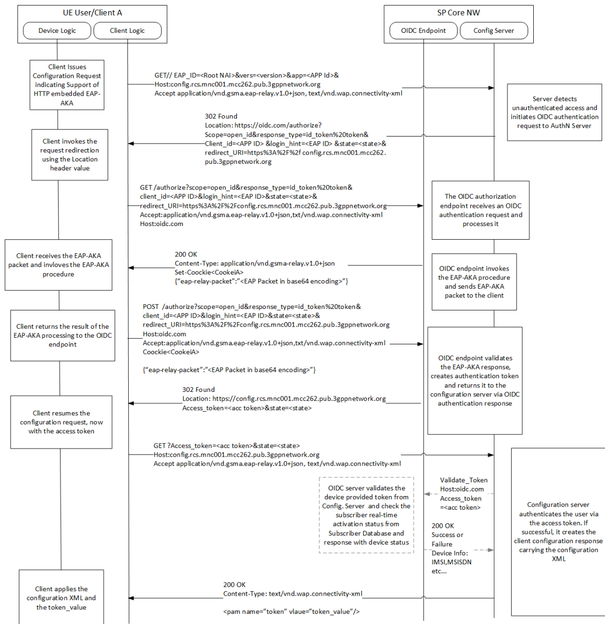
Figure 10: Authentication Flow using HTTP embedded EAP-AKA
