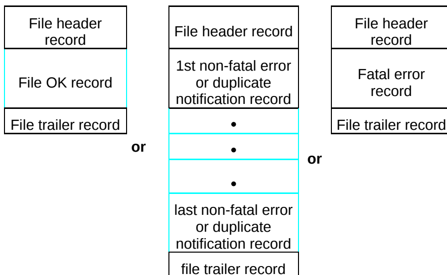
Figure 4: IMEI DB Log file structure
