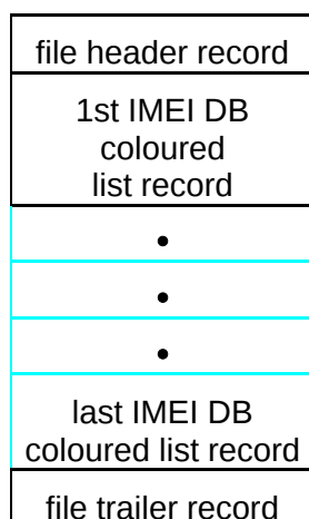
Figure 3: IMEI DB Coloured List file structure
