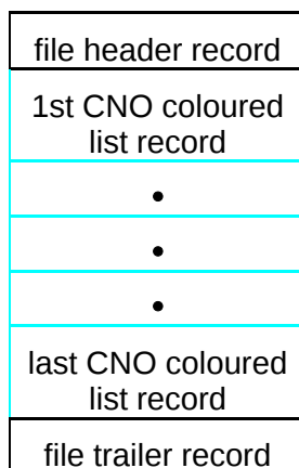
Figure 2: CNO Coloured List file structure
