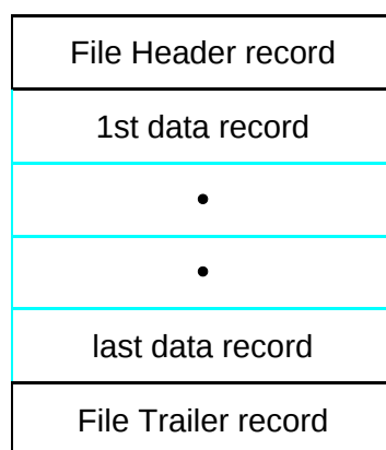
Figure 1: IMEI Database File Transfer – File Structure
