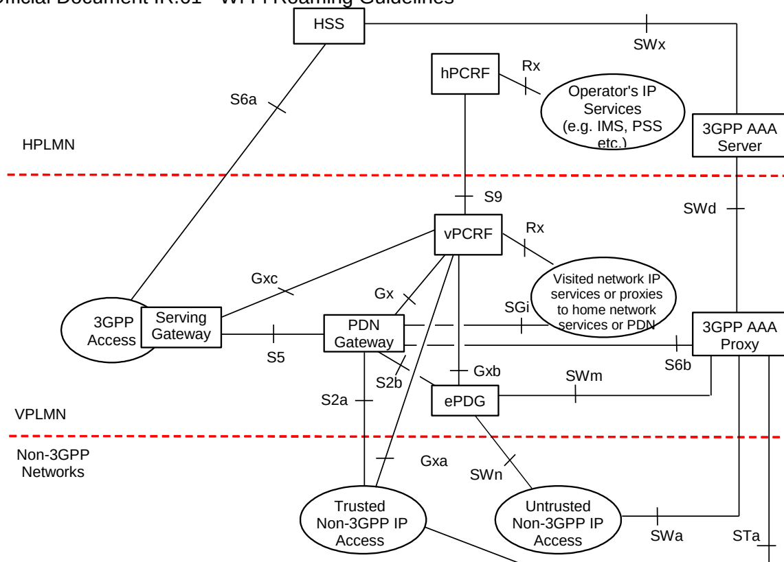
Figure 1b: Roaming Architecture for EPC using S5, S2a, S2b – Local Breakout (from 3GPP TS 23.402)
