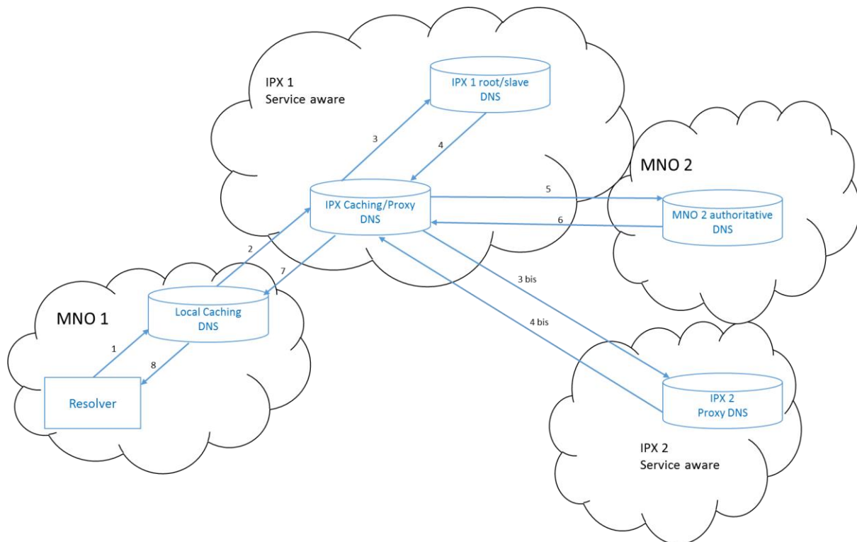
Figure 4 Service aware network resolver architecture
