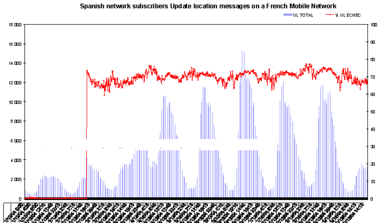
Figure 2: Example for Steering of Roaming (Multiple MAP error cause)
